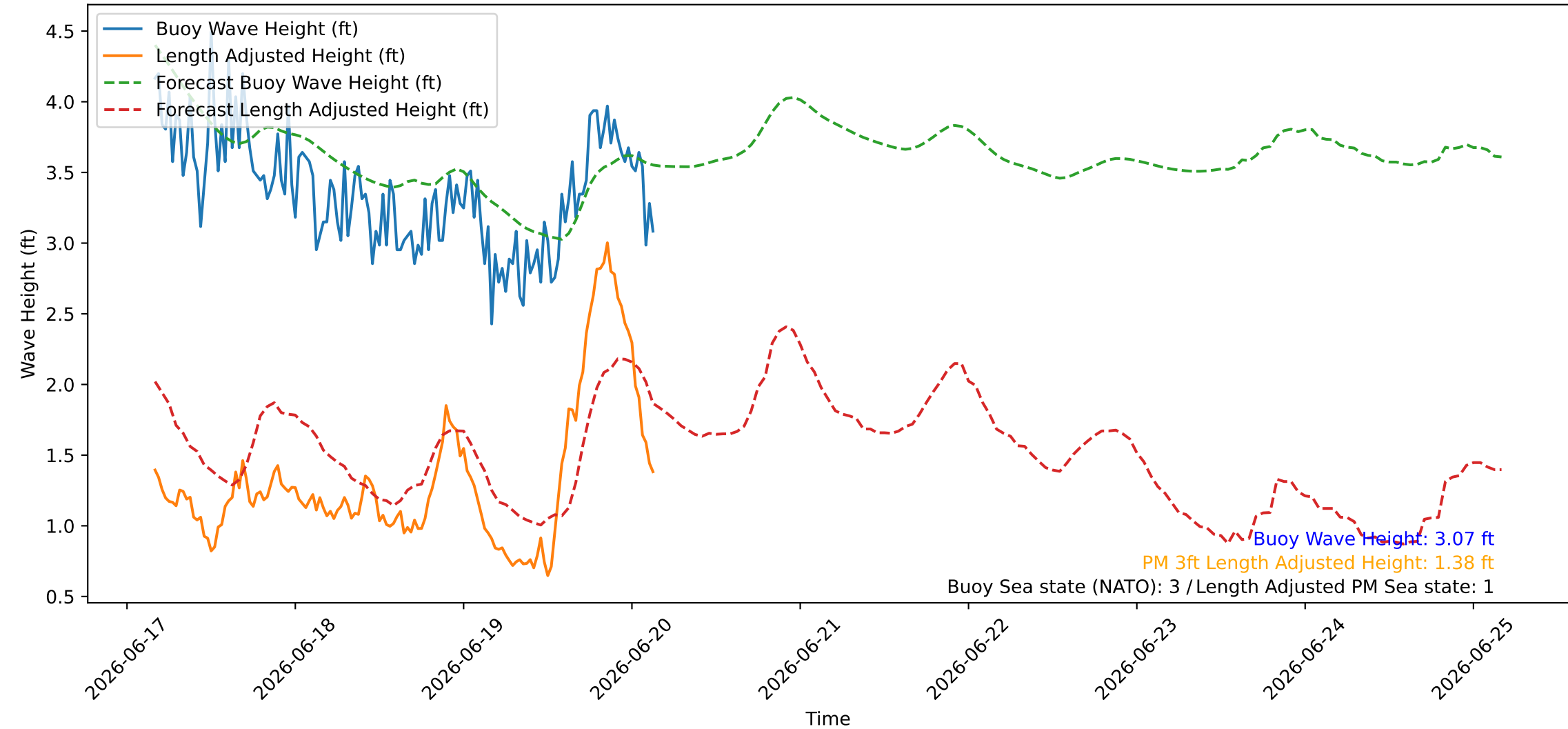
Wave Heights over Time for Green Beach at 2026-06-20 03:51:08
