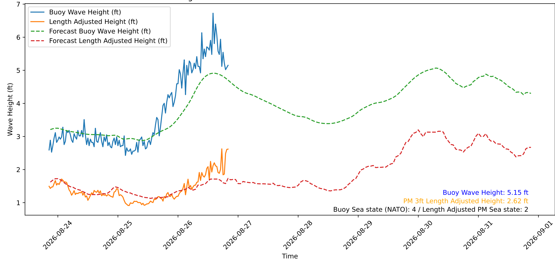
Wave Heights over Time for Oceanside Harbor at 2026-08-26 20:40:29
