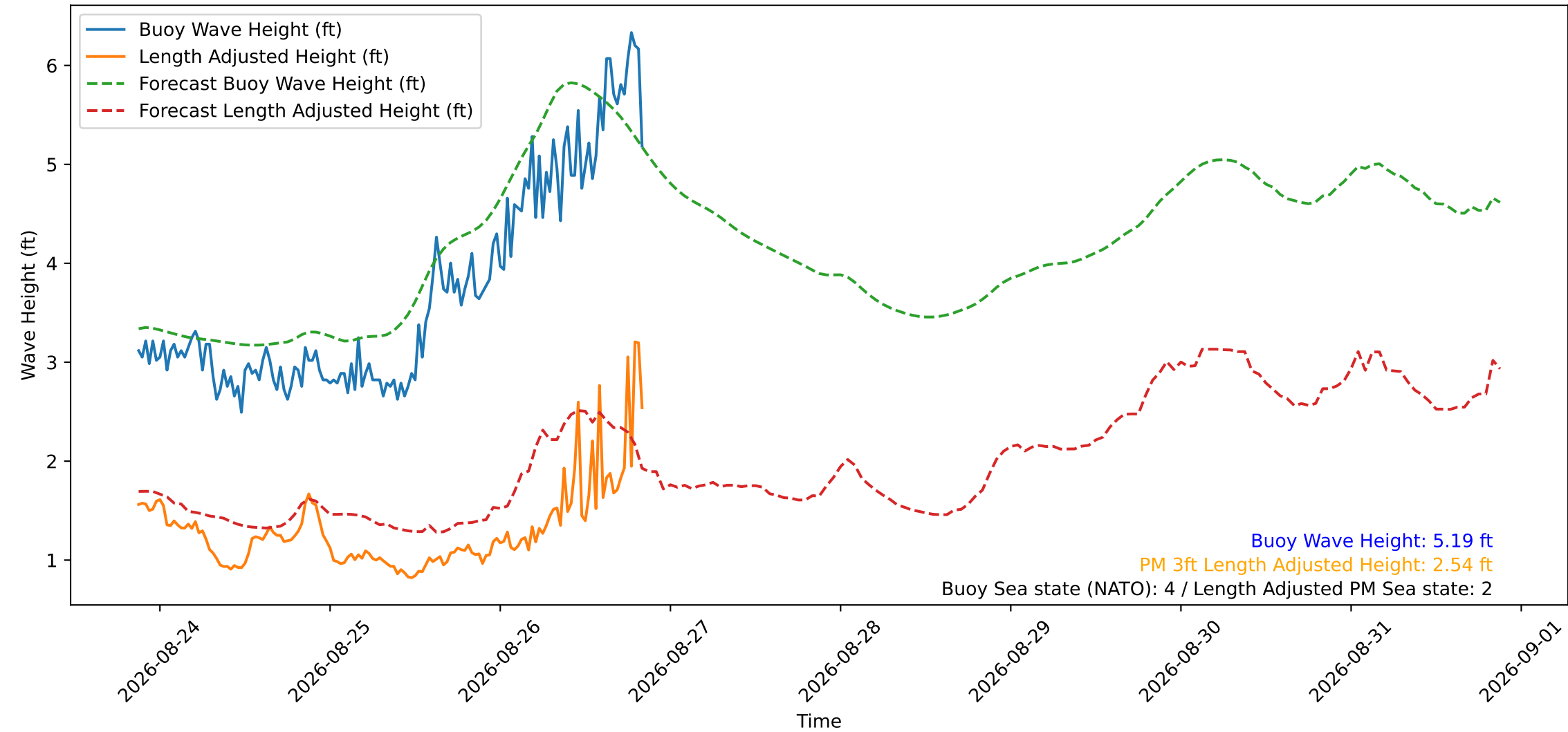
Wave Heights over Time for Green Beach at 2026-08-26 20:41:12
