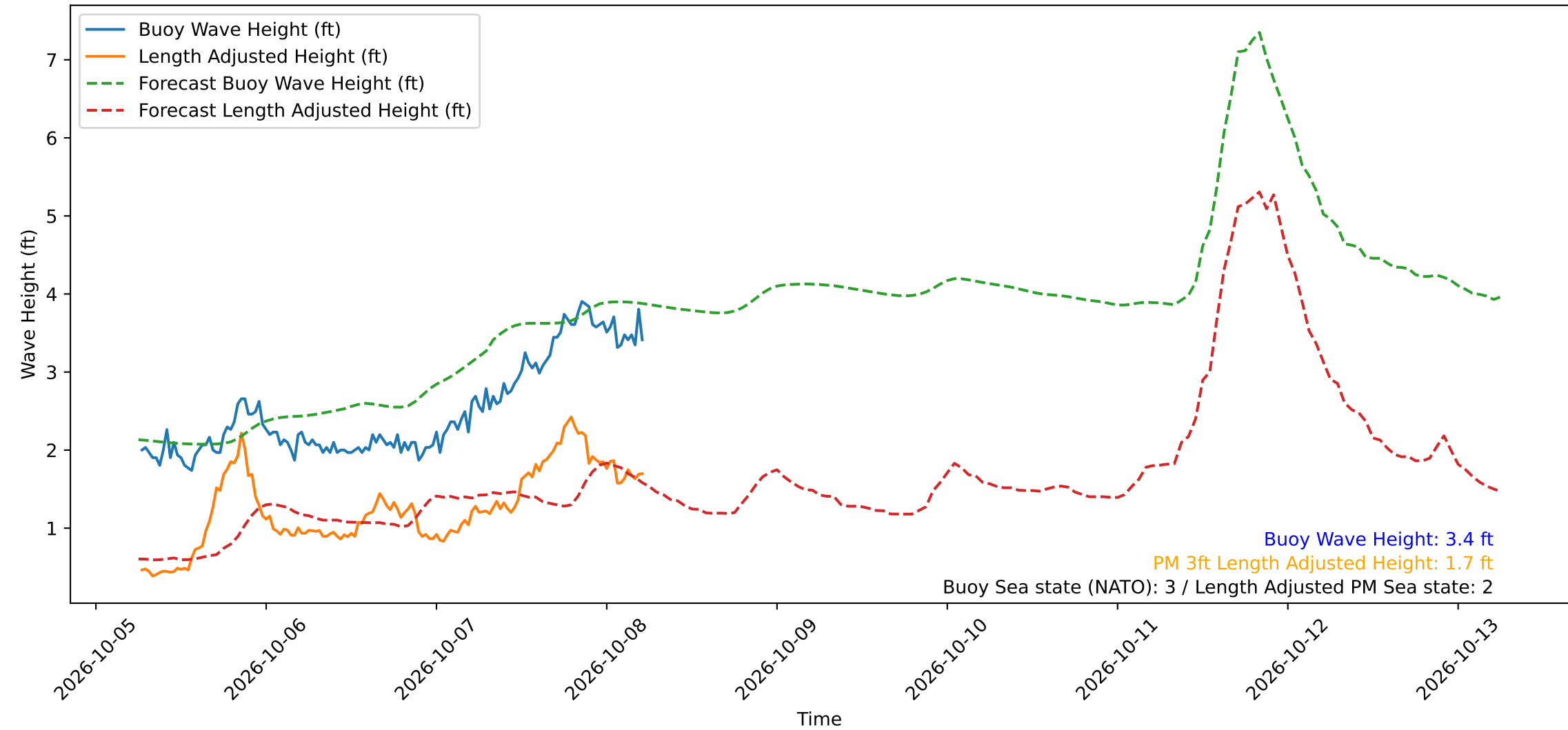
Wave Heights over Time for Red Beach at 2026-10-08 06:00:49
