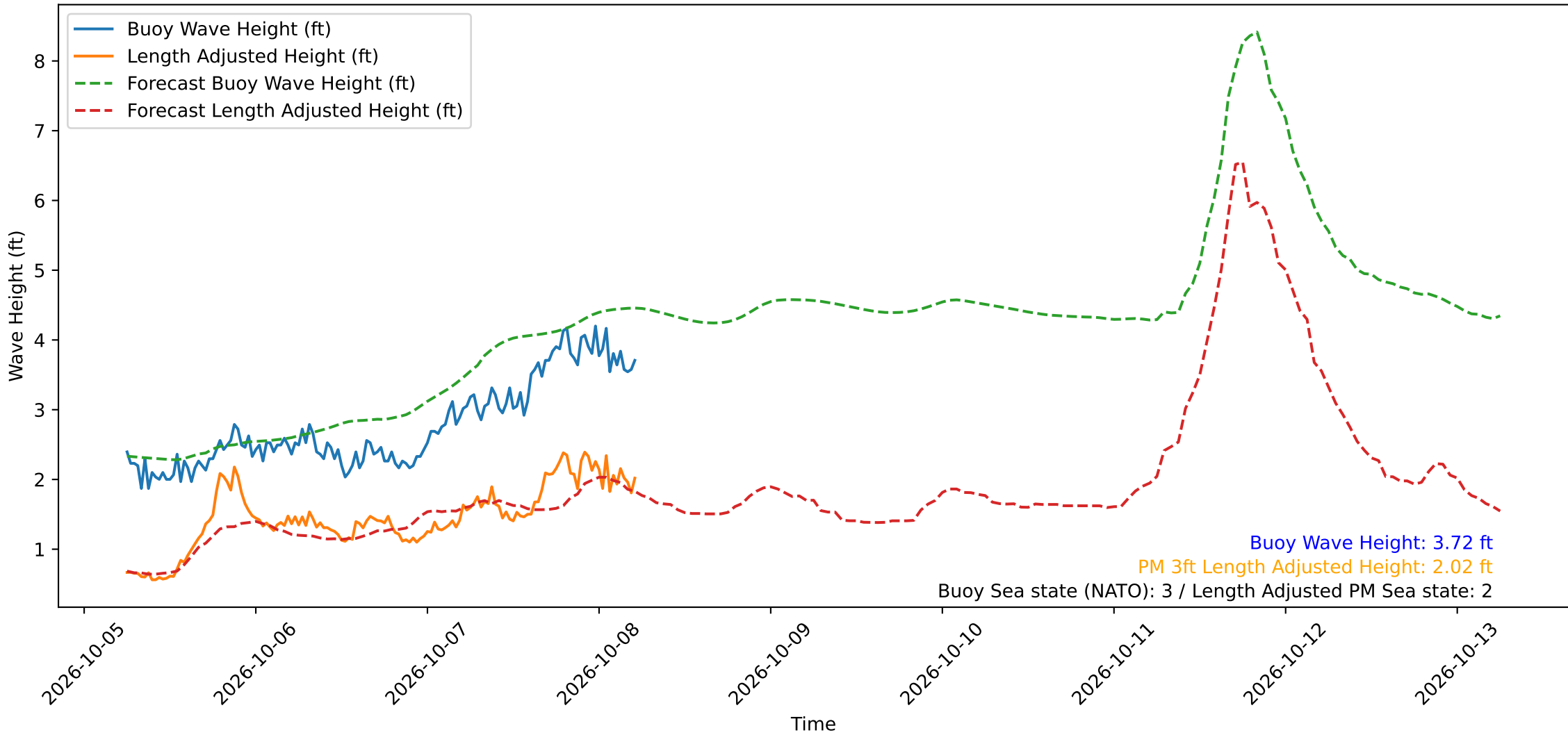
Wave Heights over Time for Oceanside Harbor at 2026-10-08 06:00:29
