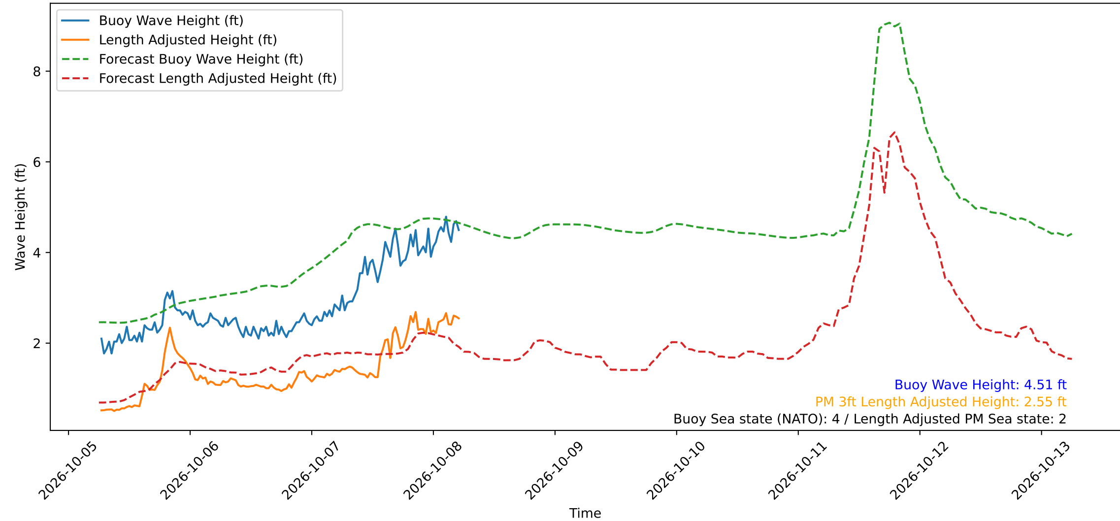
Wave Heights over Time for Green Beach at 2026-10-08 06:01:11
