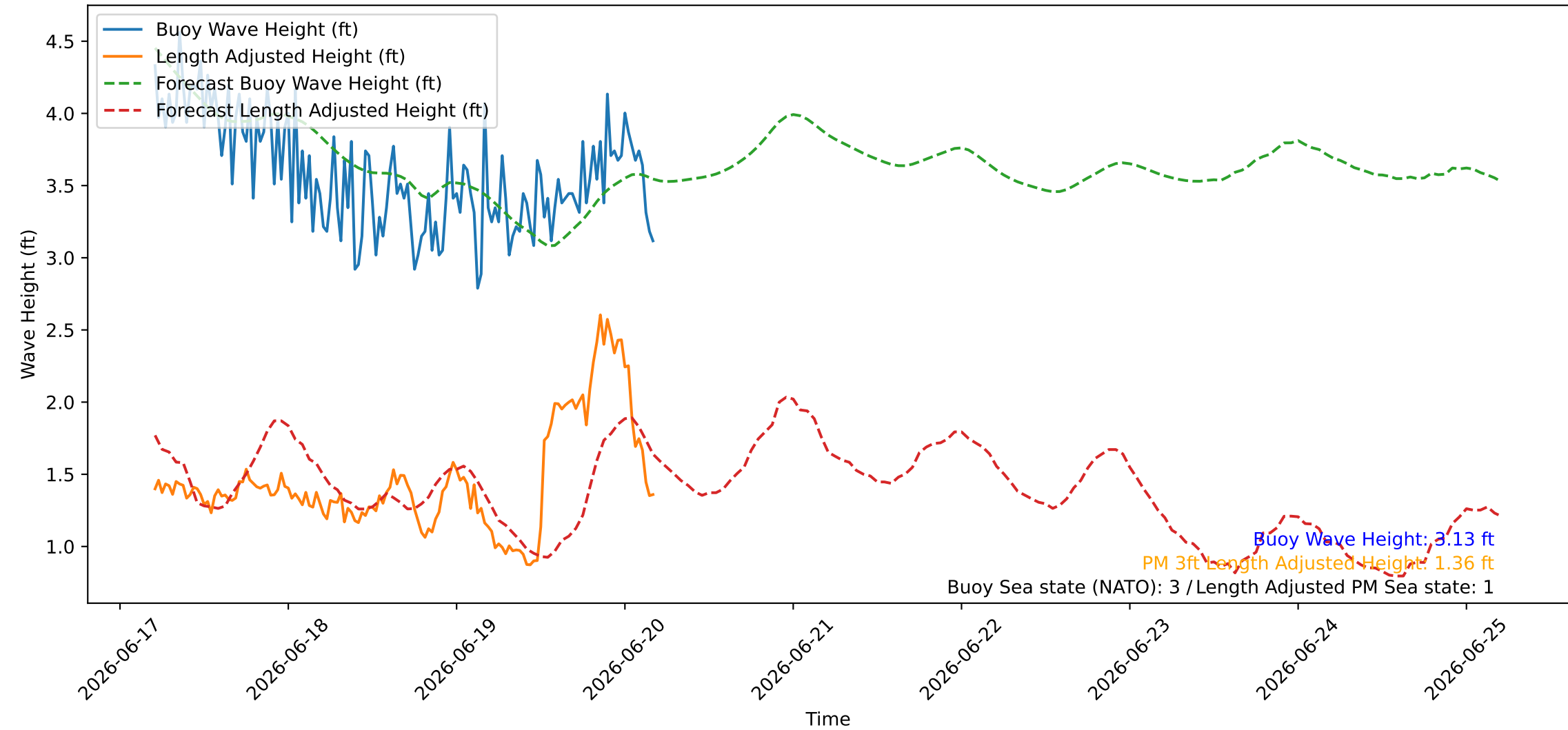
Wave Heights over Time for Oceanside Harbor at 2026-06-20 04:50:26
