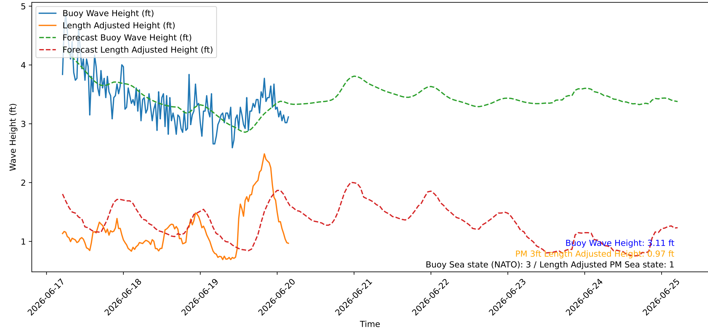
Wave Heights over Time for Red Beach at 2026-06-20 04:50:46
