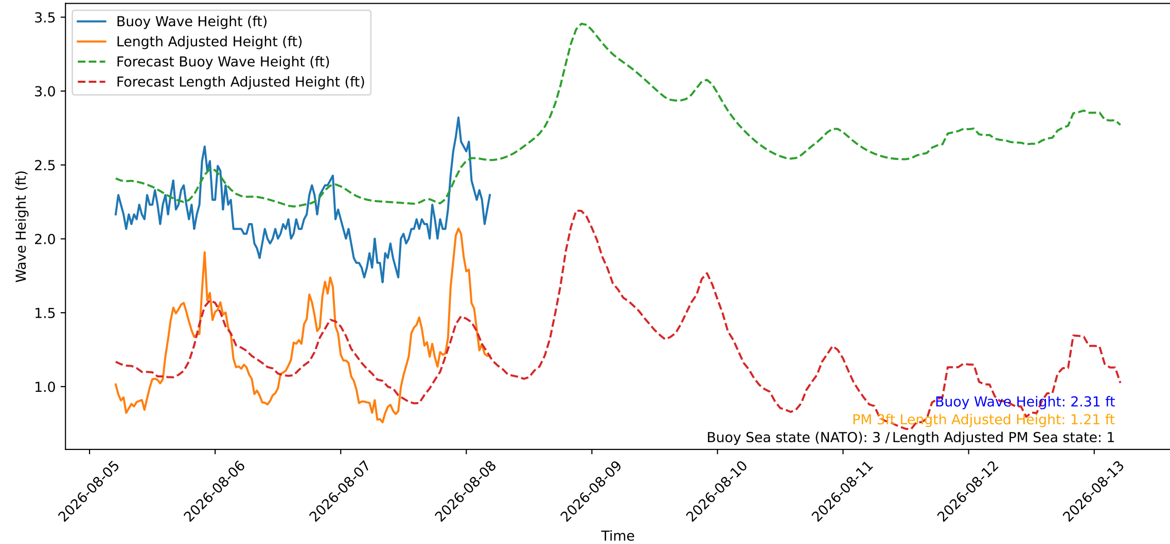
Wave Heights over Time for Green Beach at 2026-08-08 05:11:08
