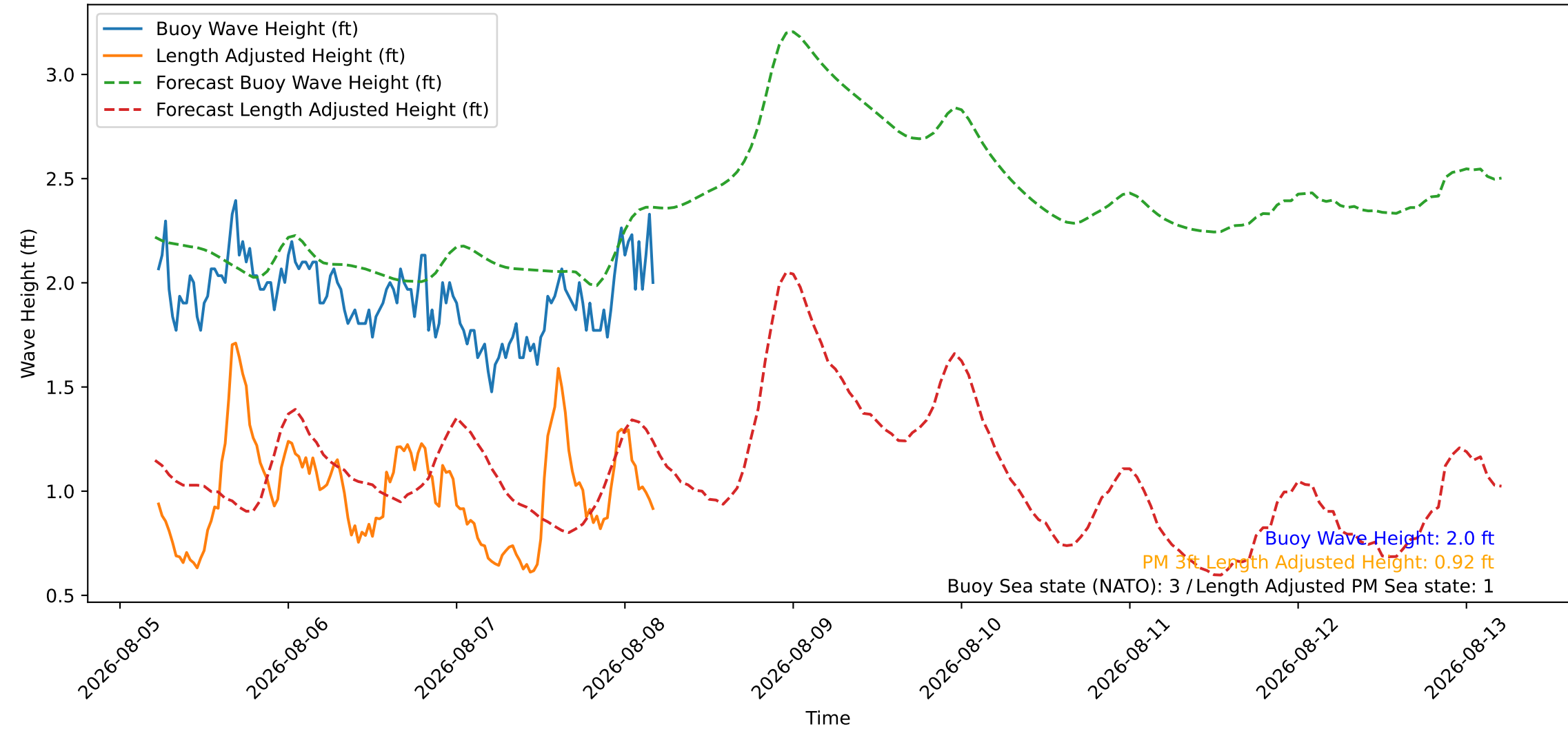
Wave Heights over Time for Red Beach at 2026-08-08 05:10:45
