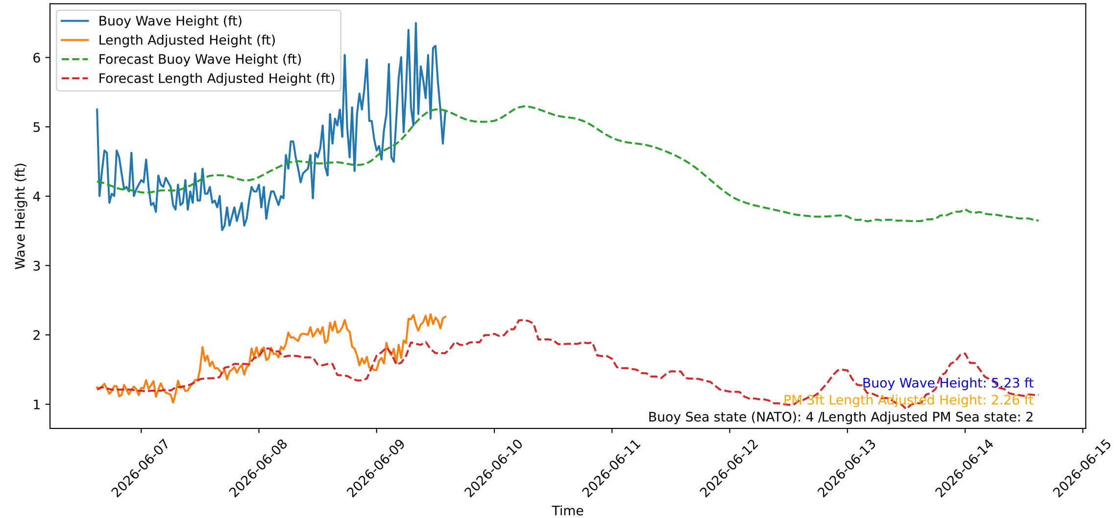
Wave Heights over Time for Oceanside Harbor at 2026-06-09 15:00:26
