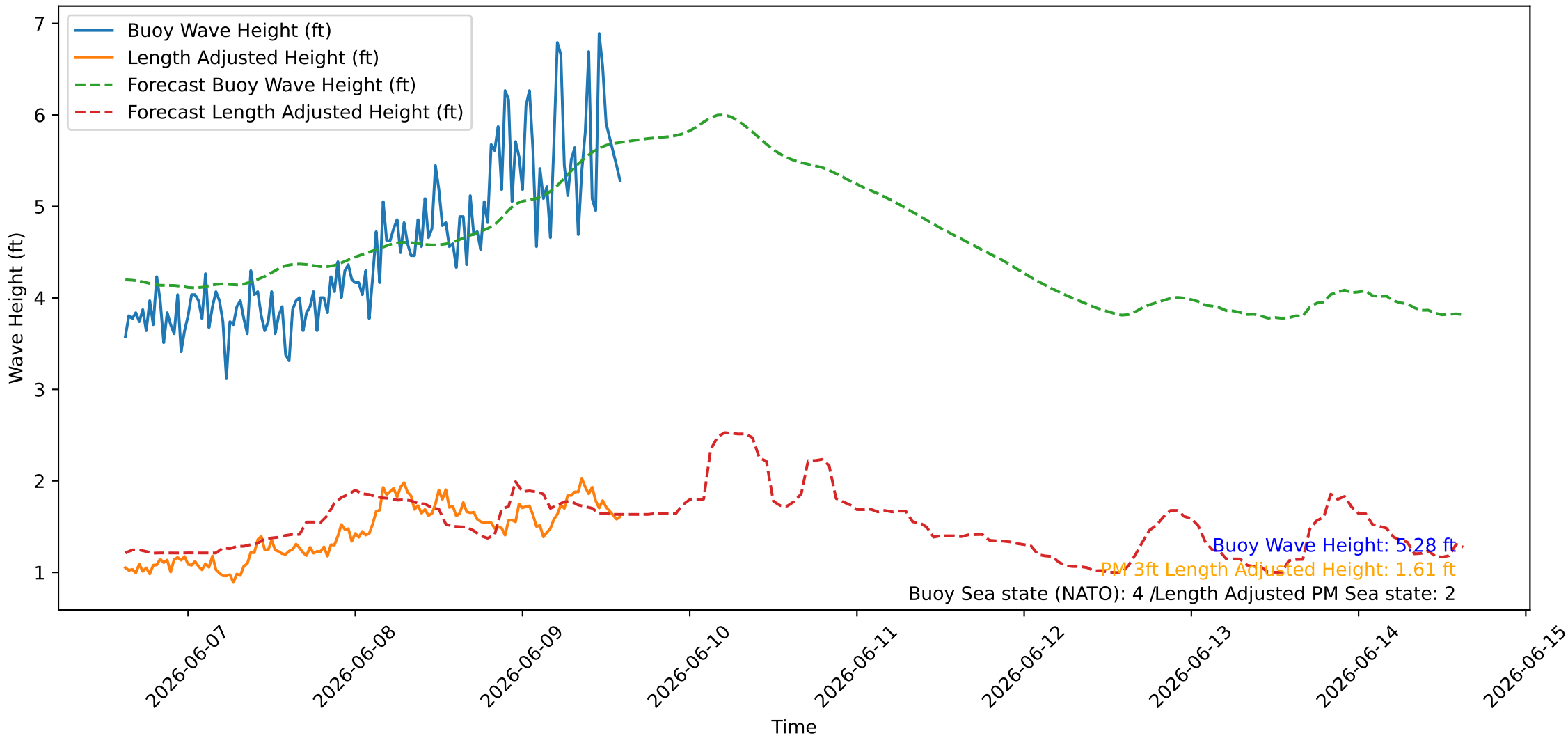
Wave Heights over Time for Green Beach at 2026-06-09 15:01:07
