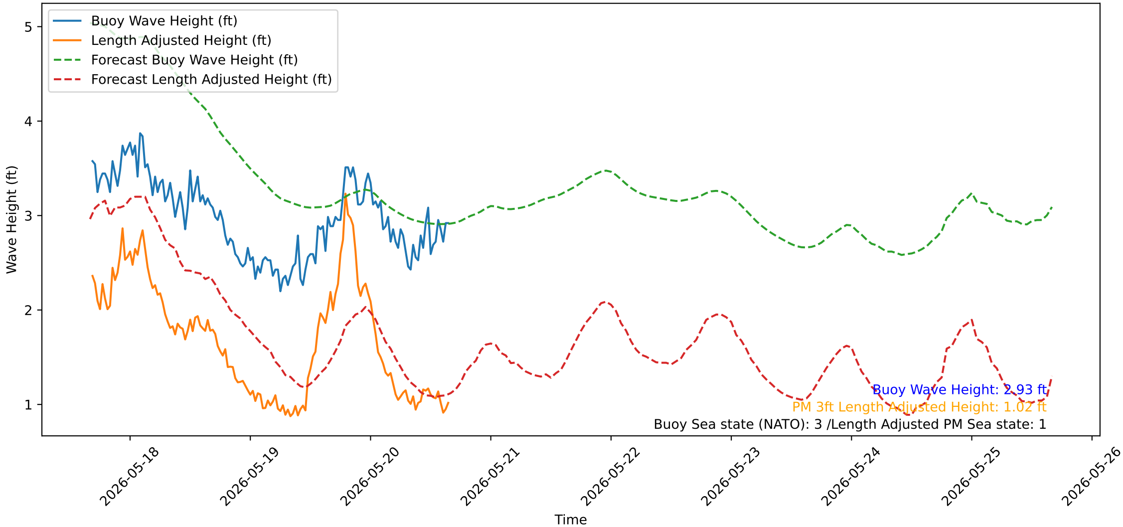
Wave Heights over Time for Oceanside Harbor at 2026-05-20 16:20:32
