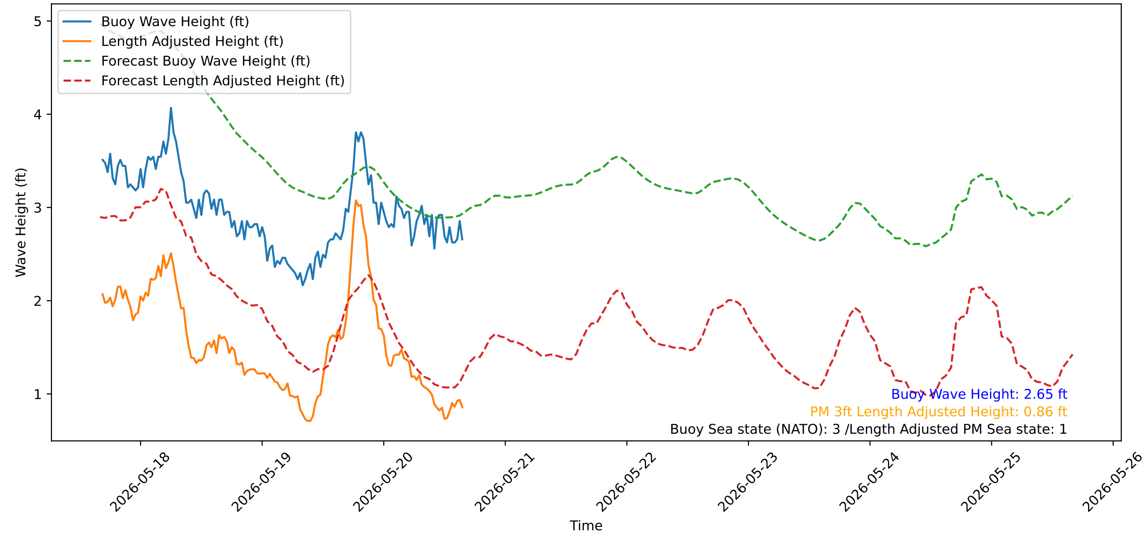
Wave Heights over Time for Green Beach at 2026-05-20 16:21:16
