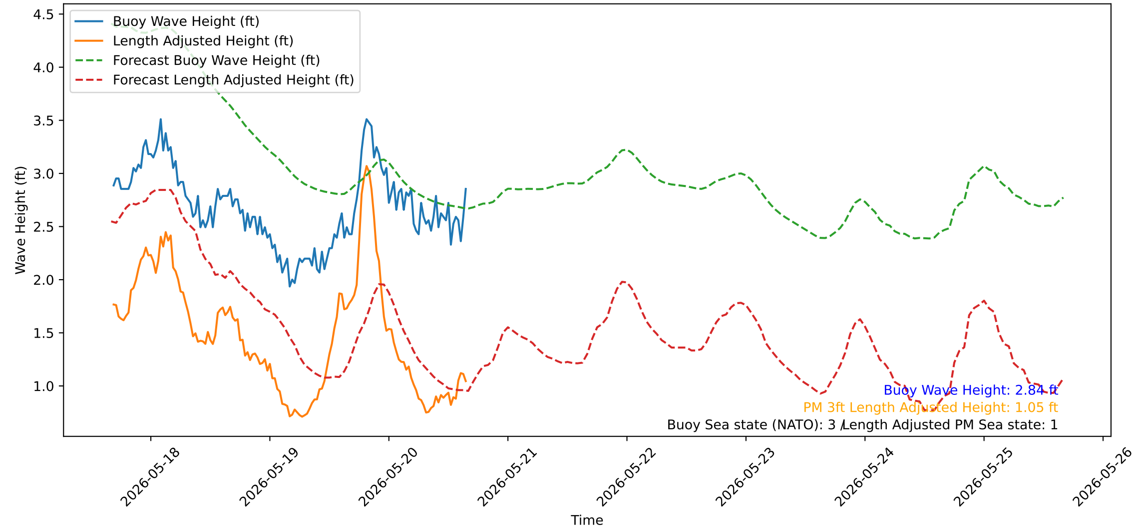
Wave Heights over Time for Red Beach at 2026-05-20 16:20:53
