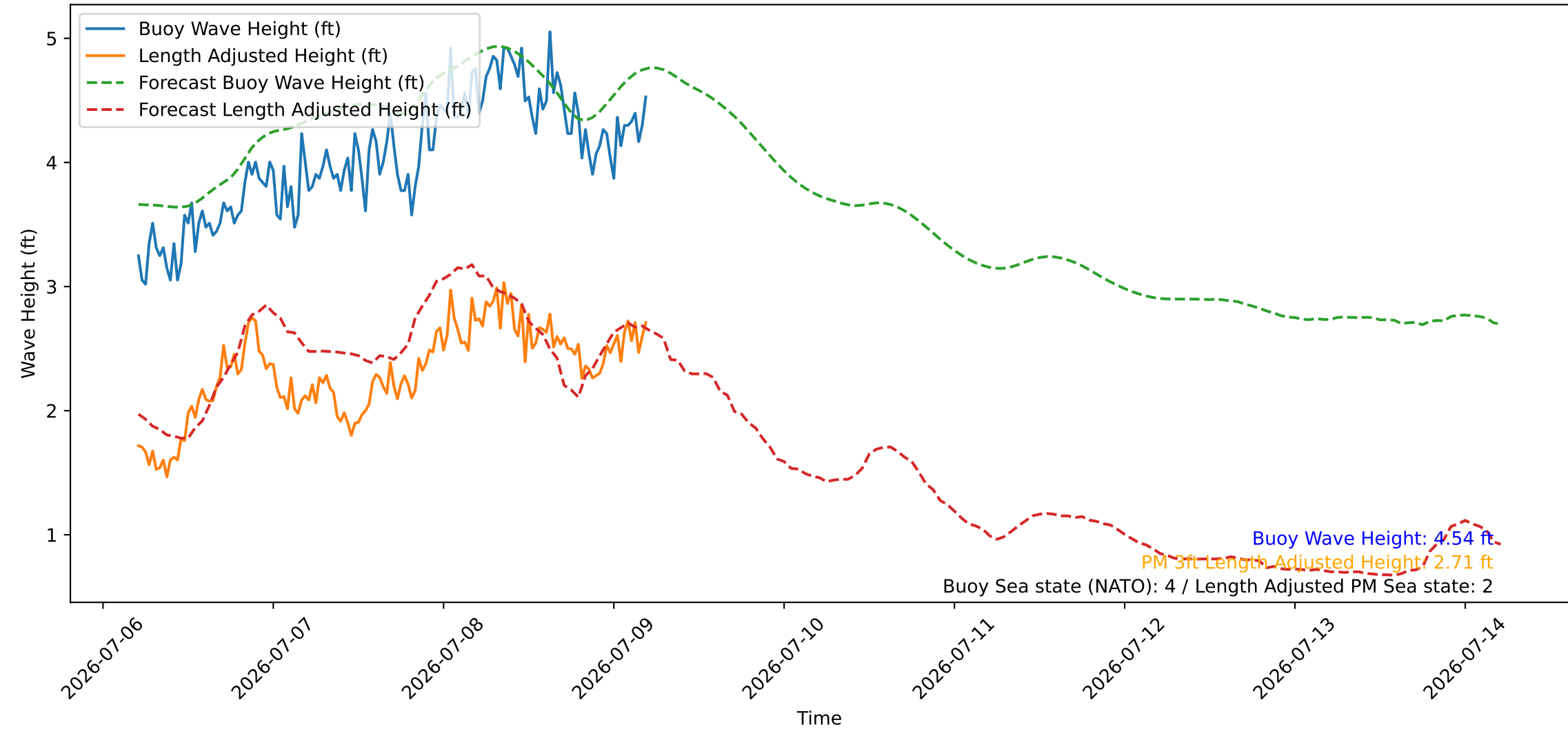
Wave Heights over Time for Oceanside Harbor at 2026-07-09 05:10:26
