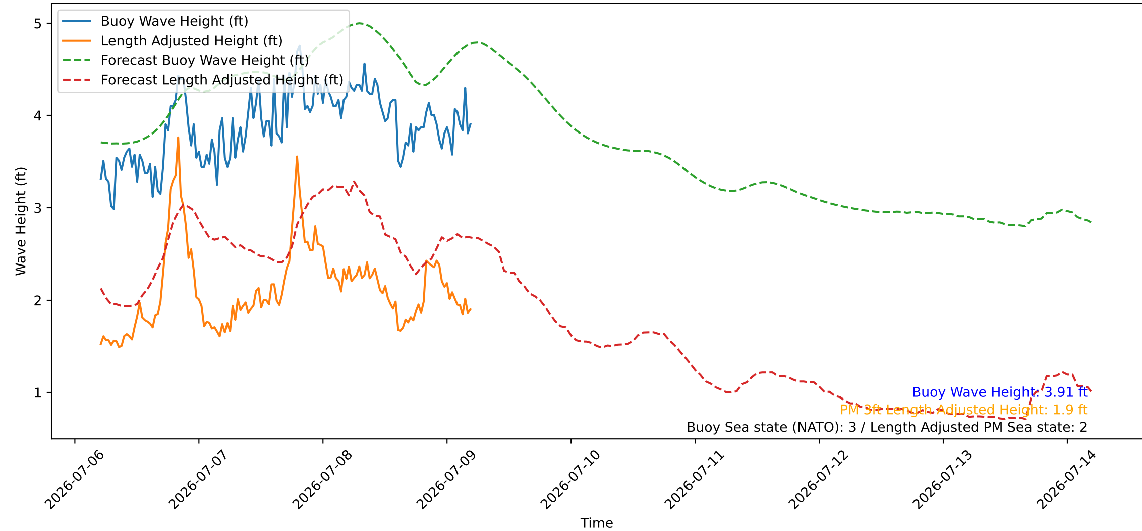
Wave Heights over Time for Green Beach at 2026-07-09 05:11:08
