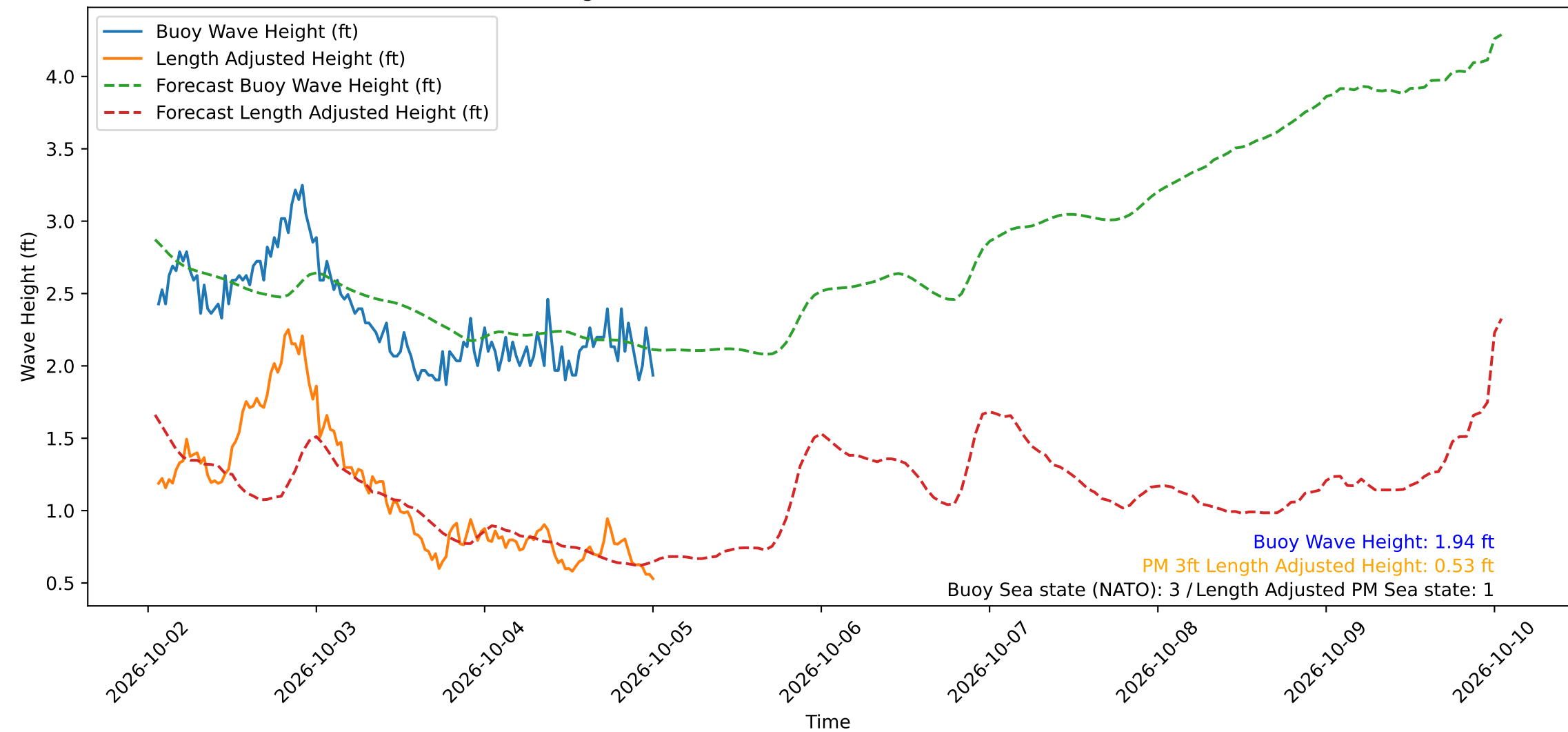
Wave Heights over Time for Red Beach at 2026-10-05 01:00:49
