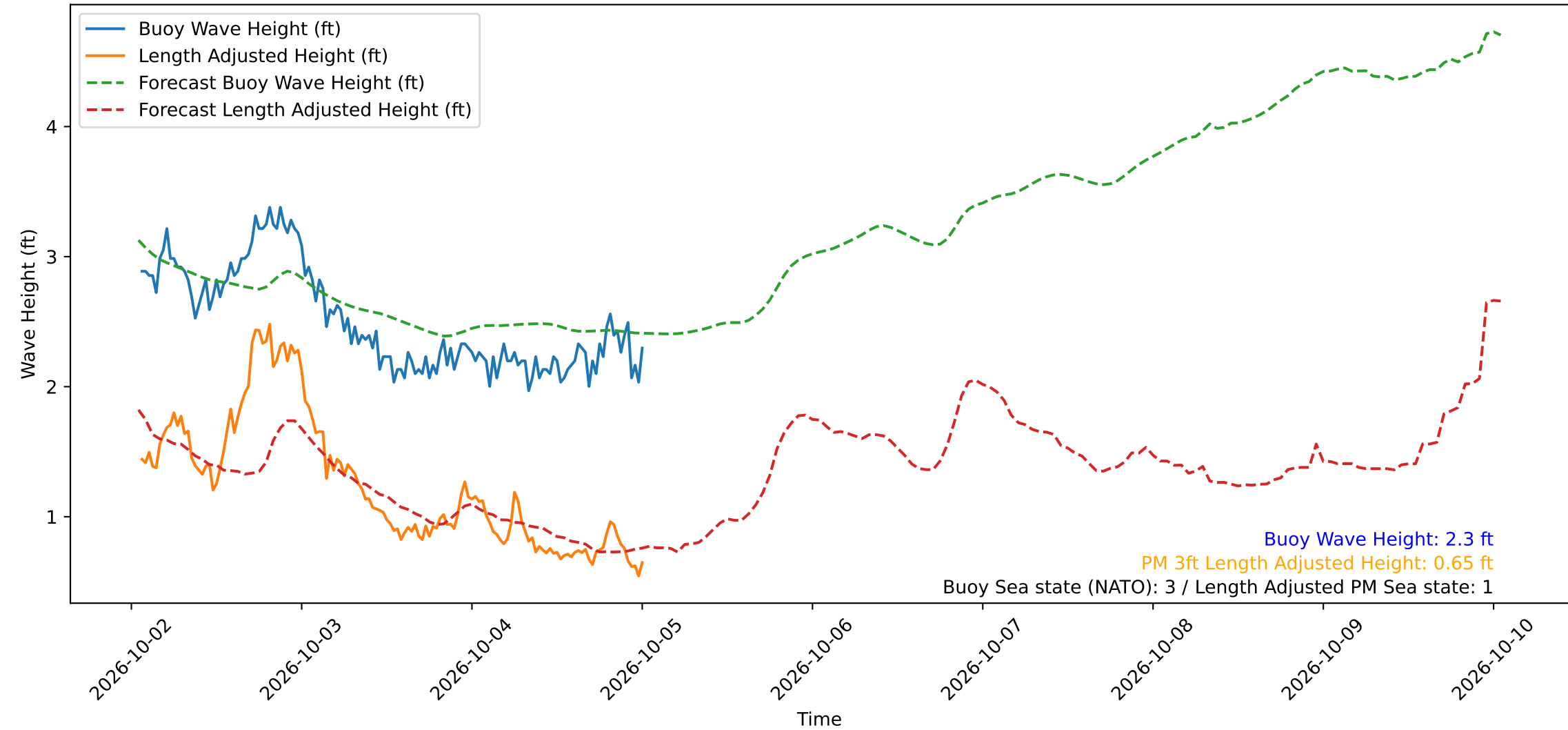
Wave Heights over Time for Green Beach at 2026-10-05 01:01:11
