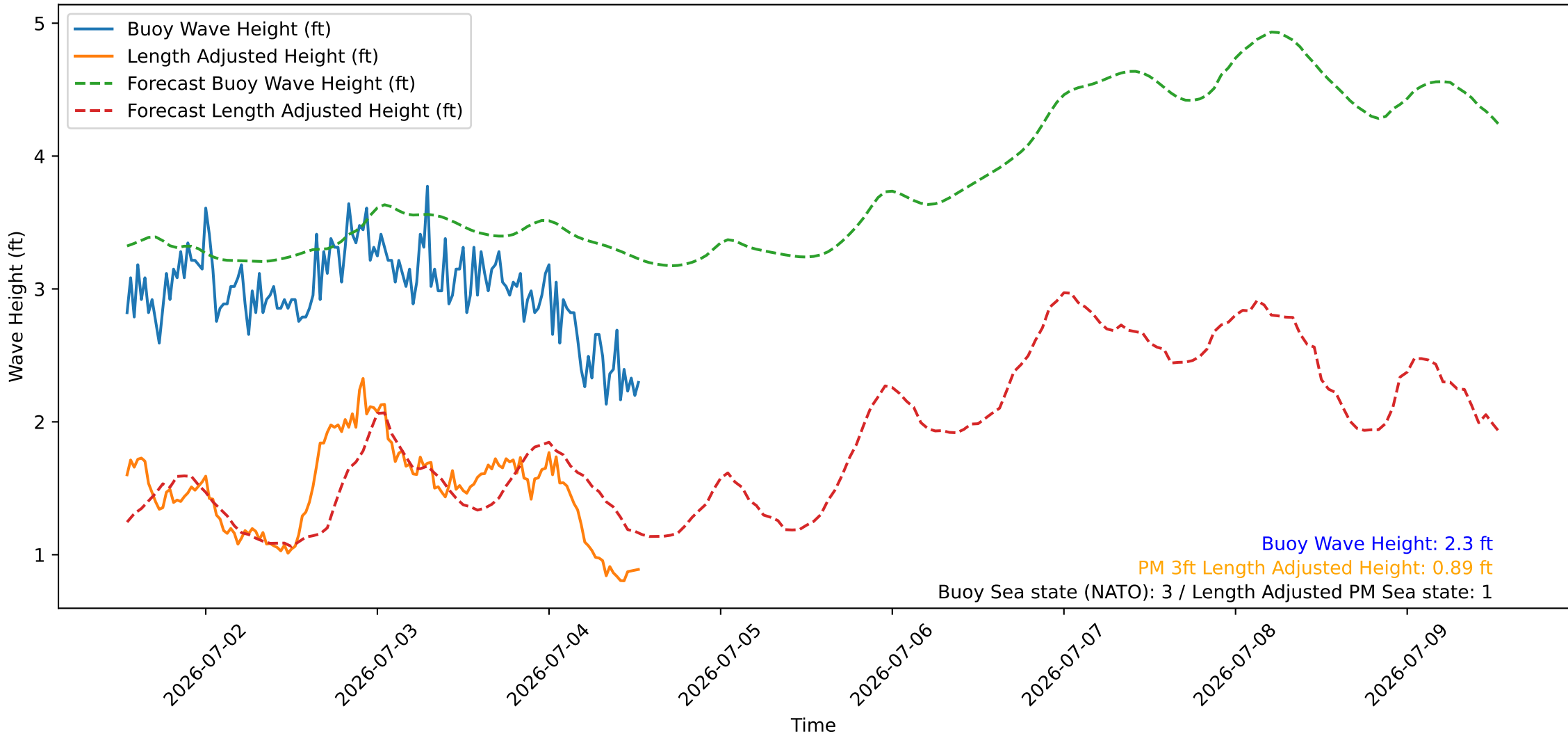
Wave Heights over Time for Oceanside Harbor at 2026-07-04 13:10:26
