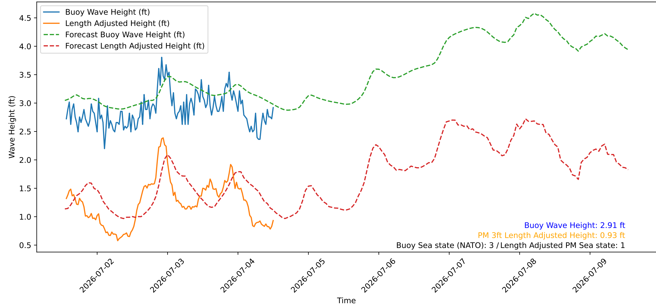
Wave Heights over Time for Red Beach at 2026-07-04 13:10:46
