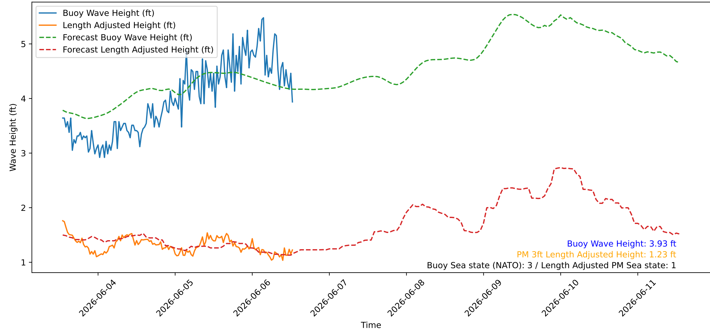
Wave Heights over Time for Oceanside Harbor at 2026-06-06 13:10:27
