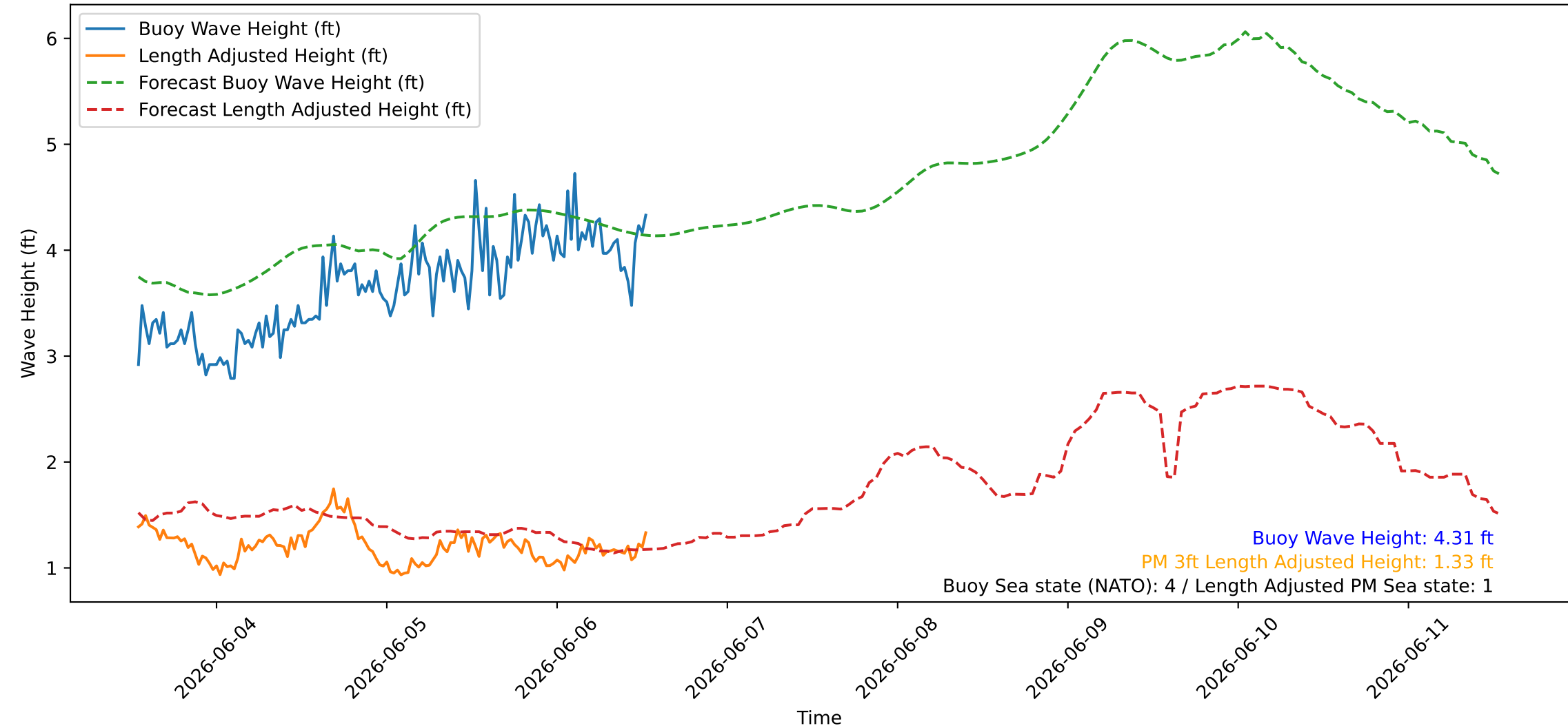
Wave Heights over Time for Green Beach at 2026-06-06 13:11:09
