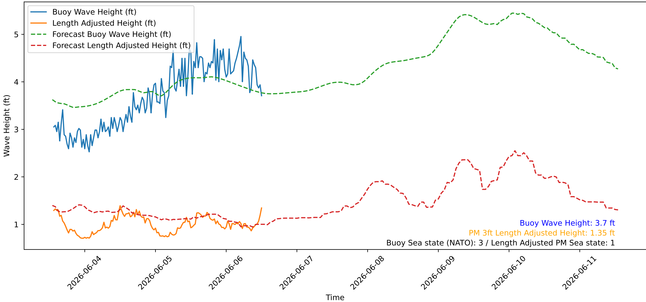
Wave Heights over Time for Red Beach at 2026-06-06 13:10:46
