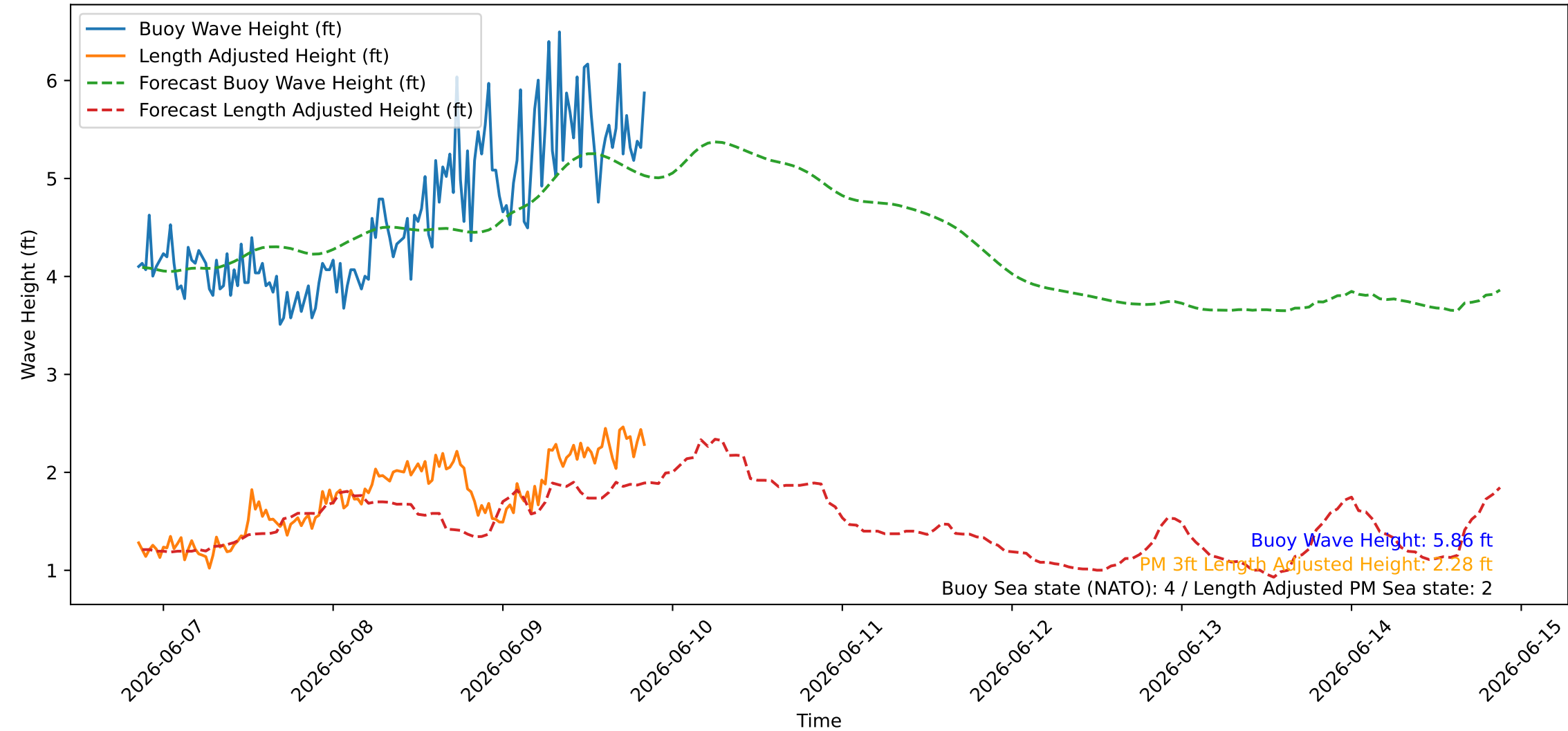
Wave Heights over Time for Oceanside Harbor at 2026-06-09 20:30:26
