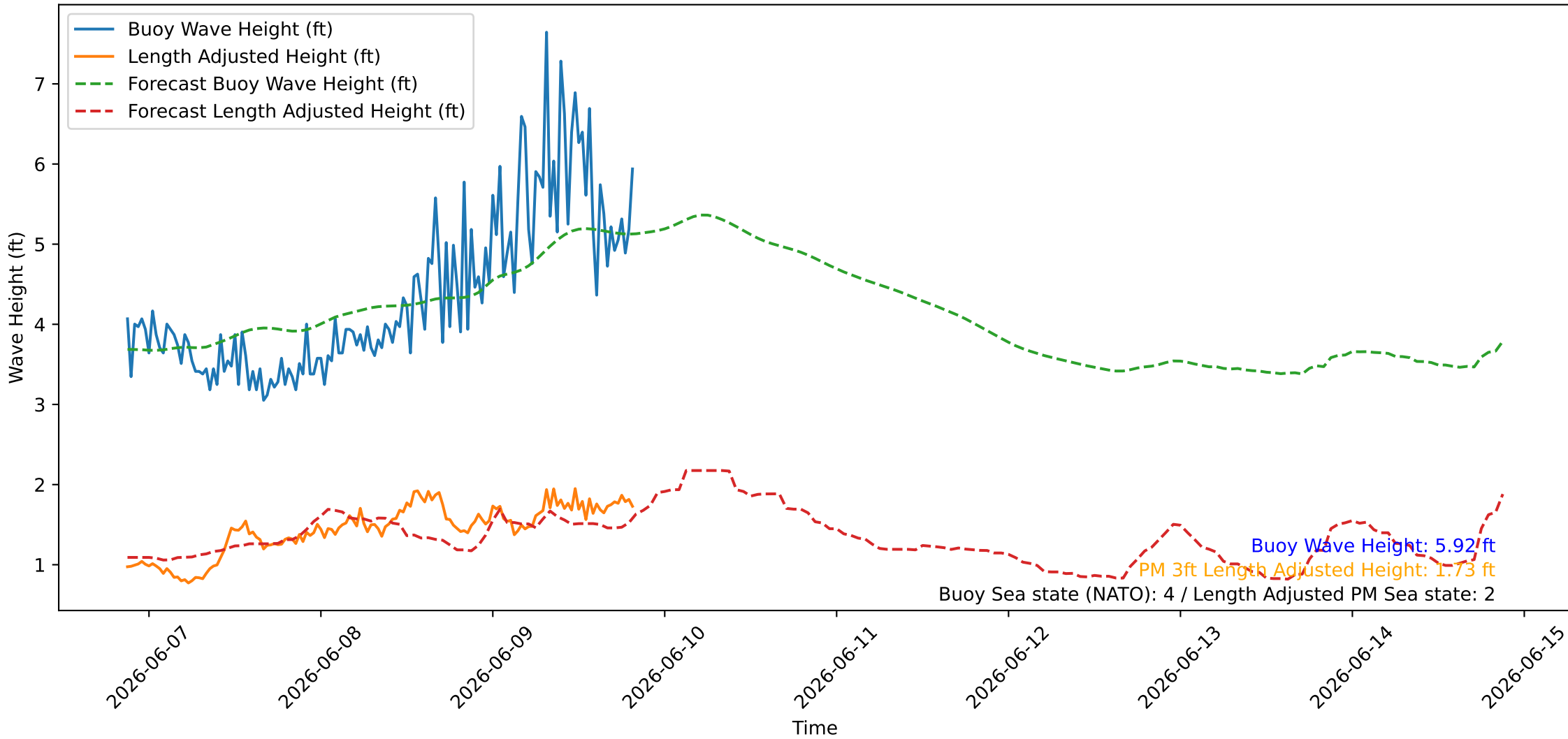
Wave Heights over Time for Red Beach at 2026-06-09 20:30:46
