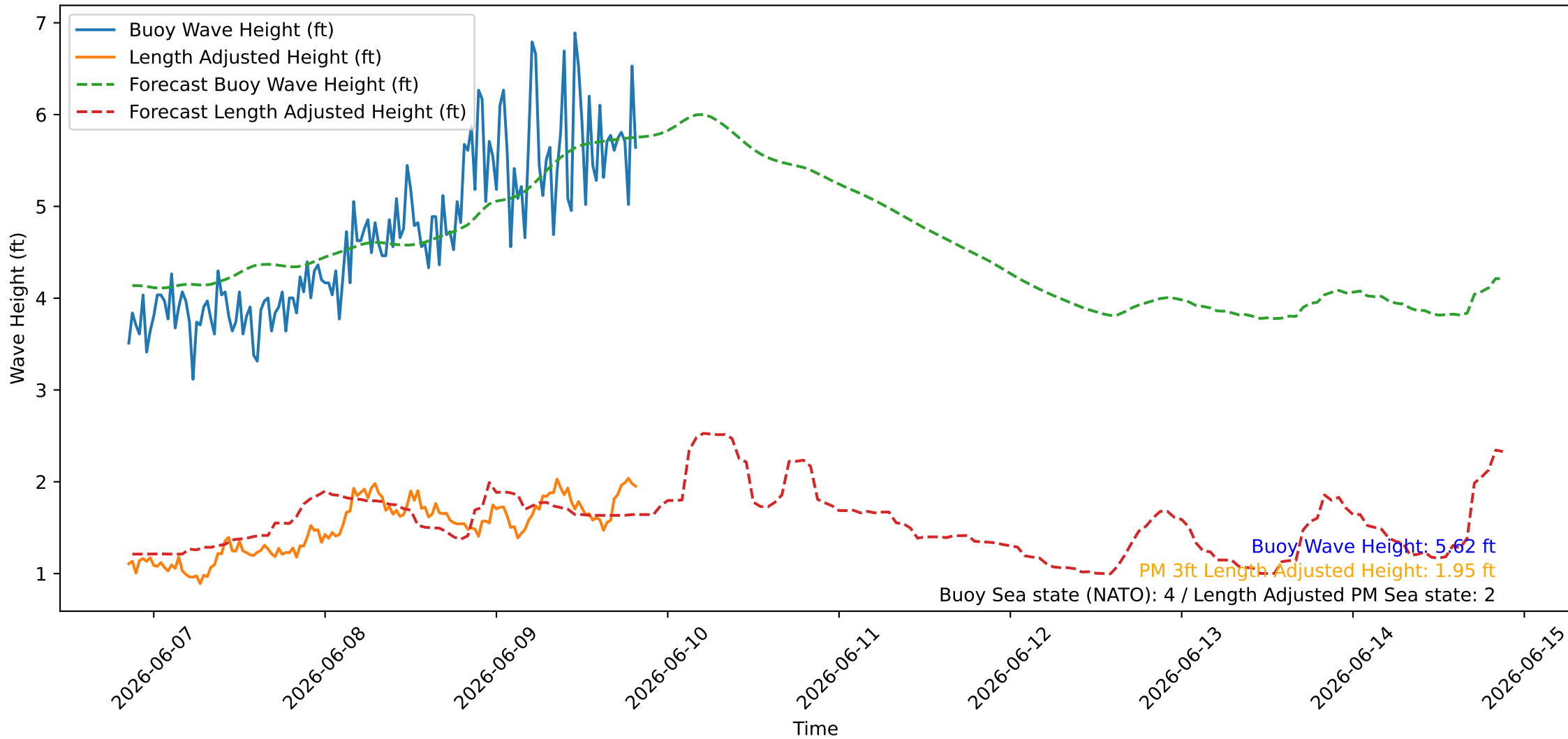
Wave Heights over Time for Green Beach at 2026-06-09 20:31:09
