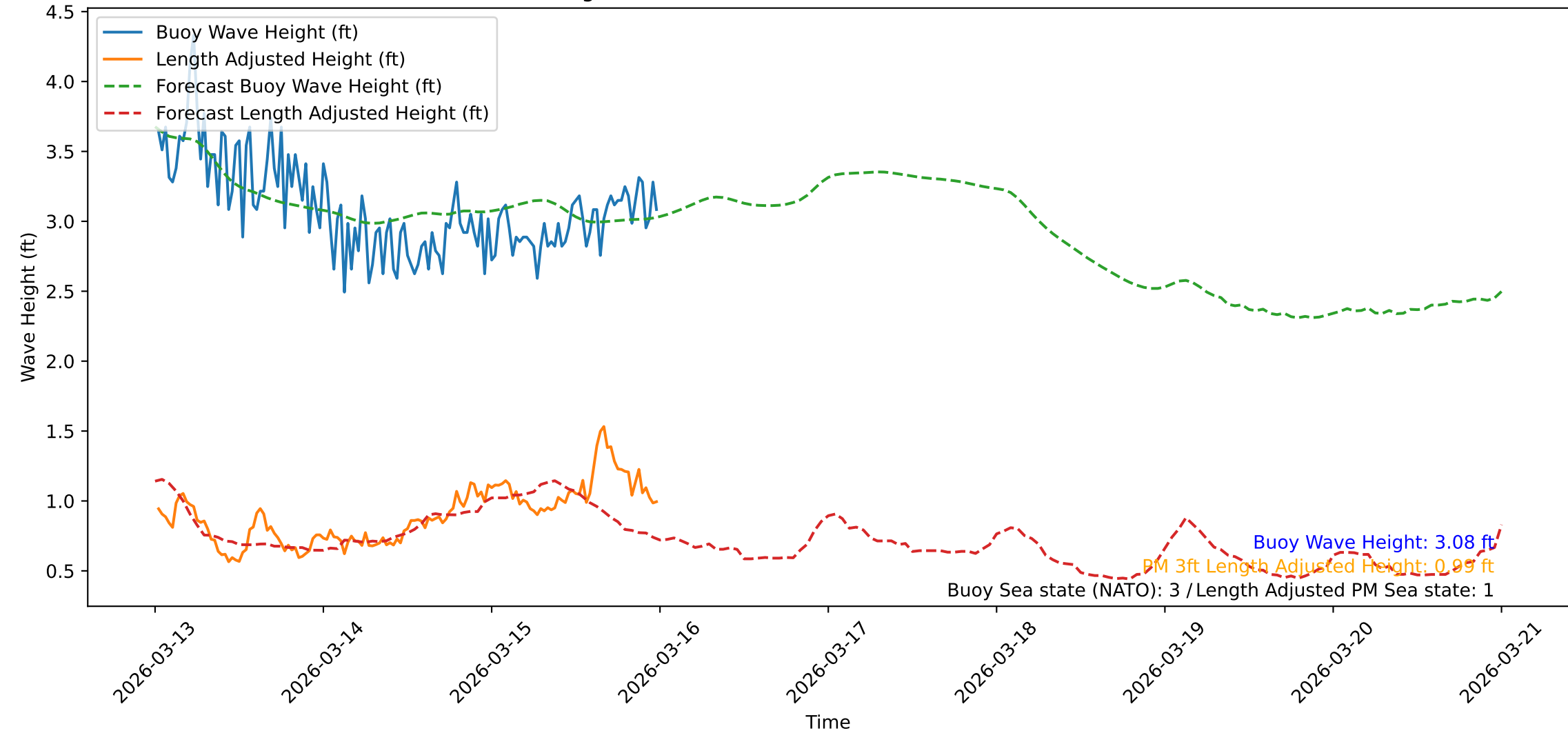
Wave Heights over Time for Red Beach at 2026-03-16 00:21:04
