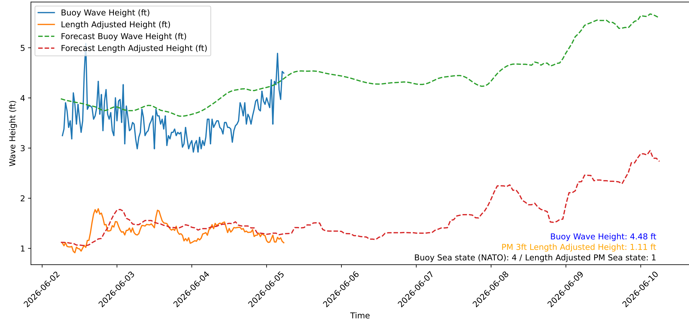
Wave Heights over Time for Oceanside Harbor at 2026-06-05 06:20:26
