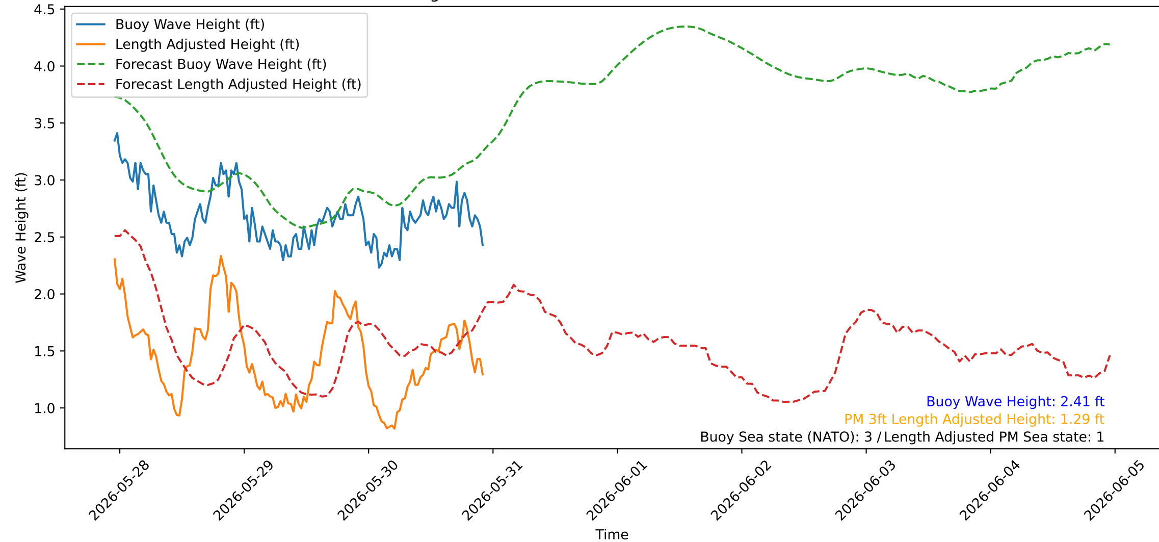
Wave Heights over Time for Red Beach at 2026-05-30 22:50:45
