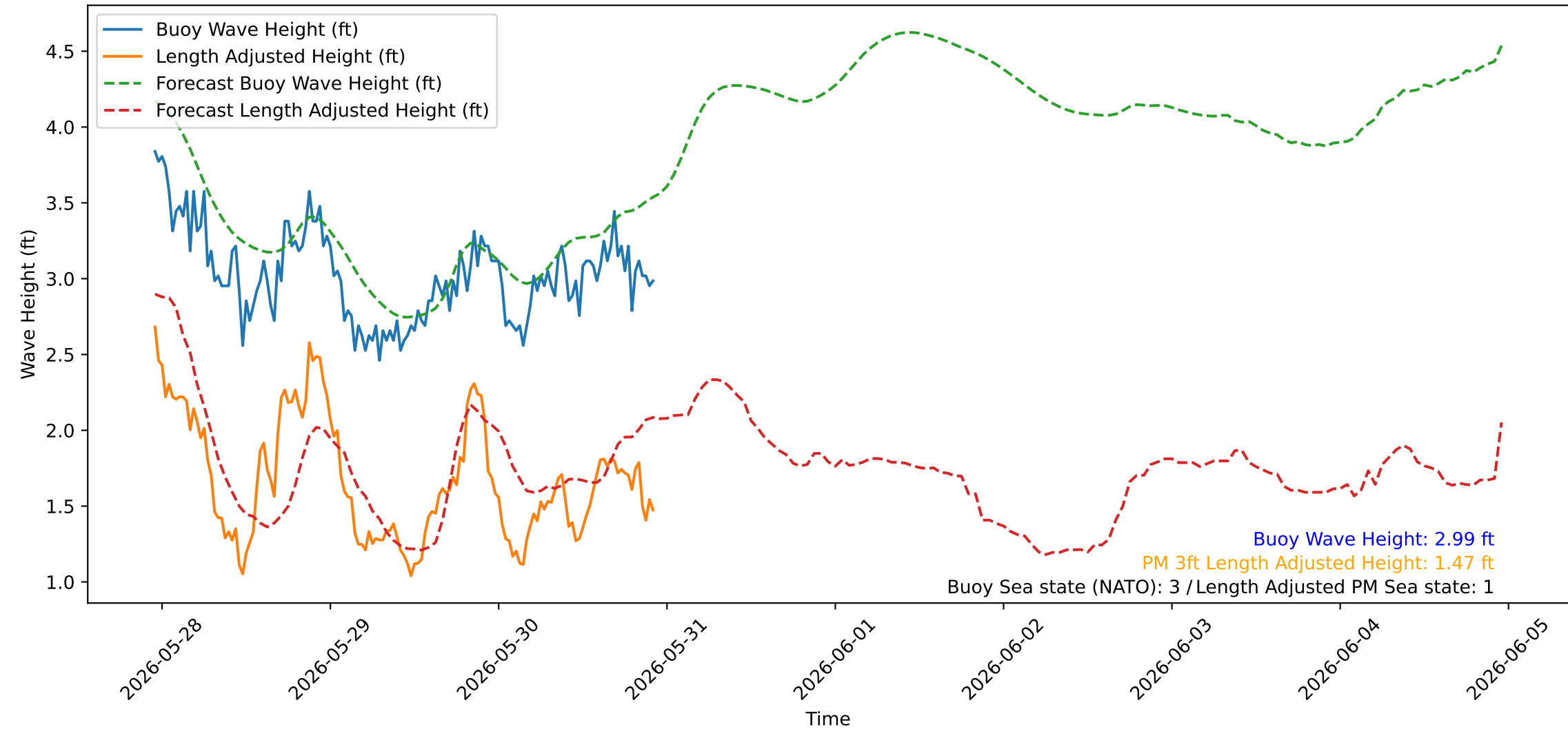
Wave Heights over Time for Green Beach at 2026-05-30 22:51:08
