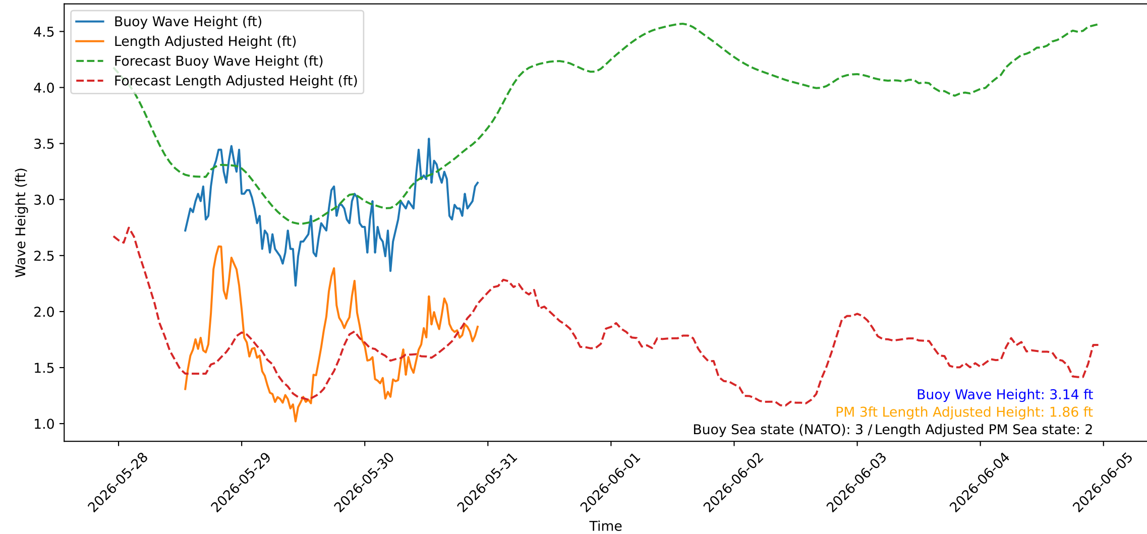
Wave Heights over Time for Oceanside Harbor at 2026-05-30 22:50:24
