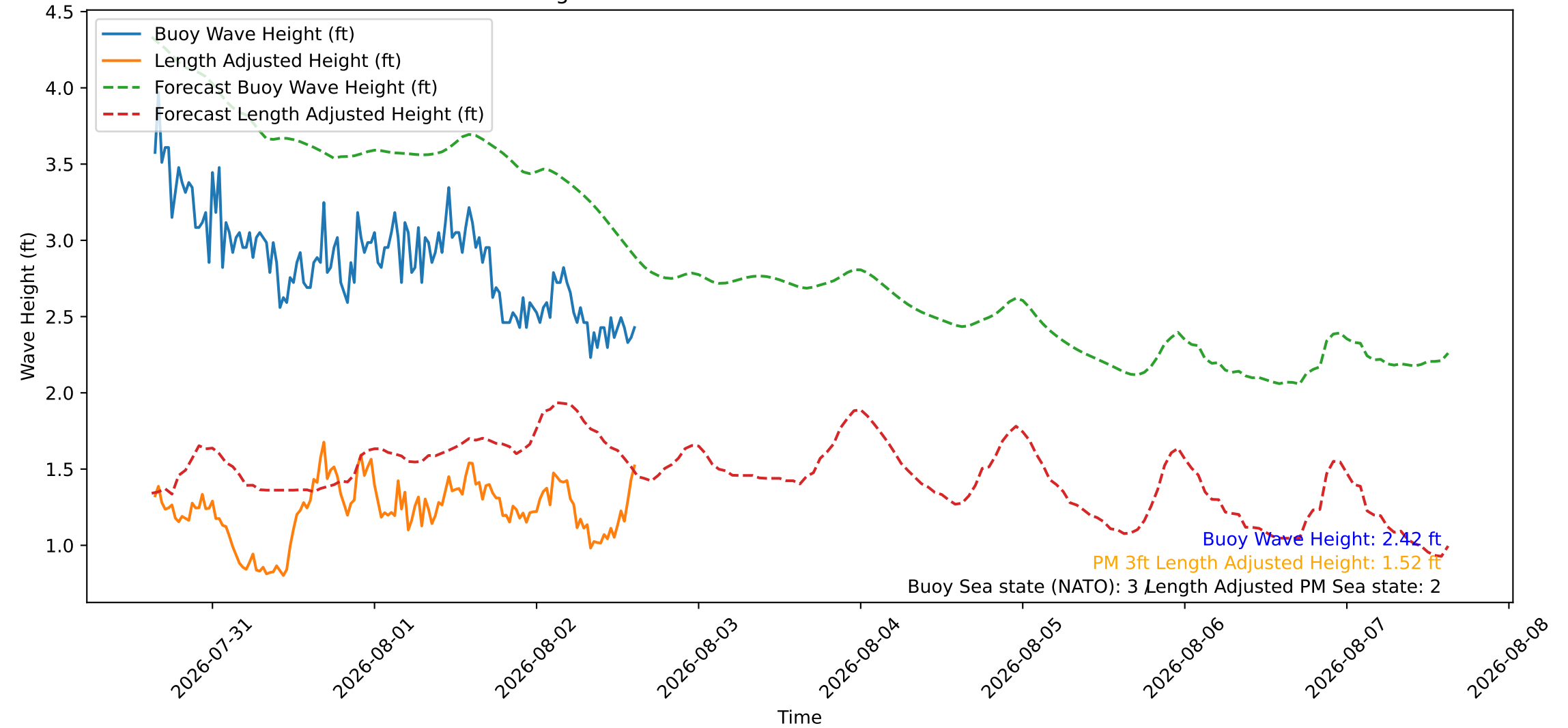
Wave Heights over Time for Red Beach at 2026-08-02 15:20:48
