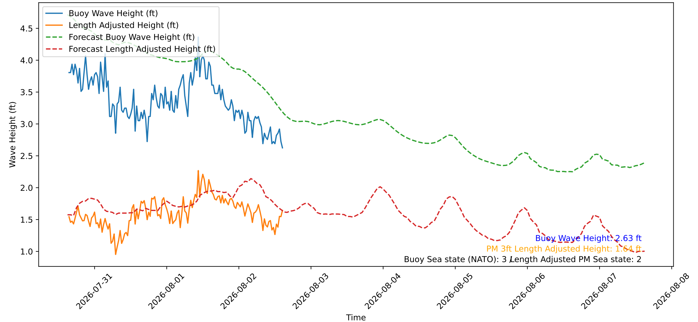
Wave Heights over Time for Oceanside Harbor at 2026-08-02 15:20:27
