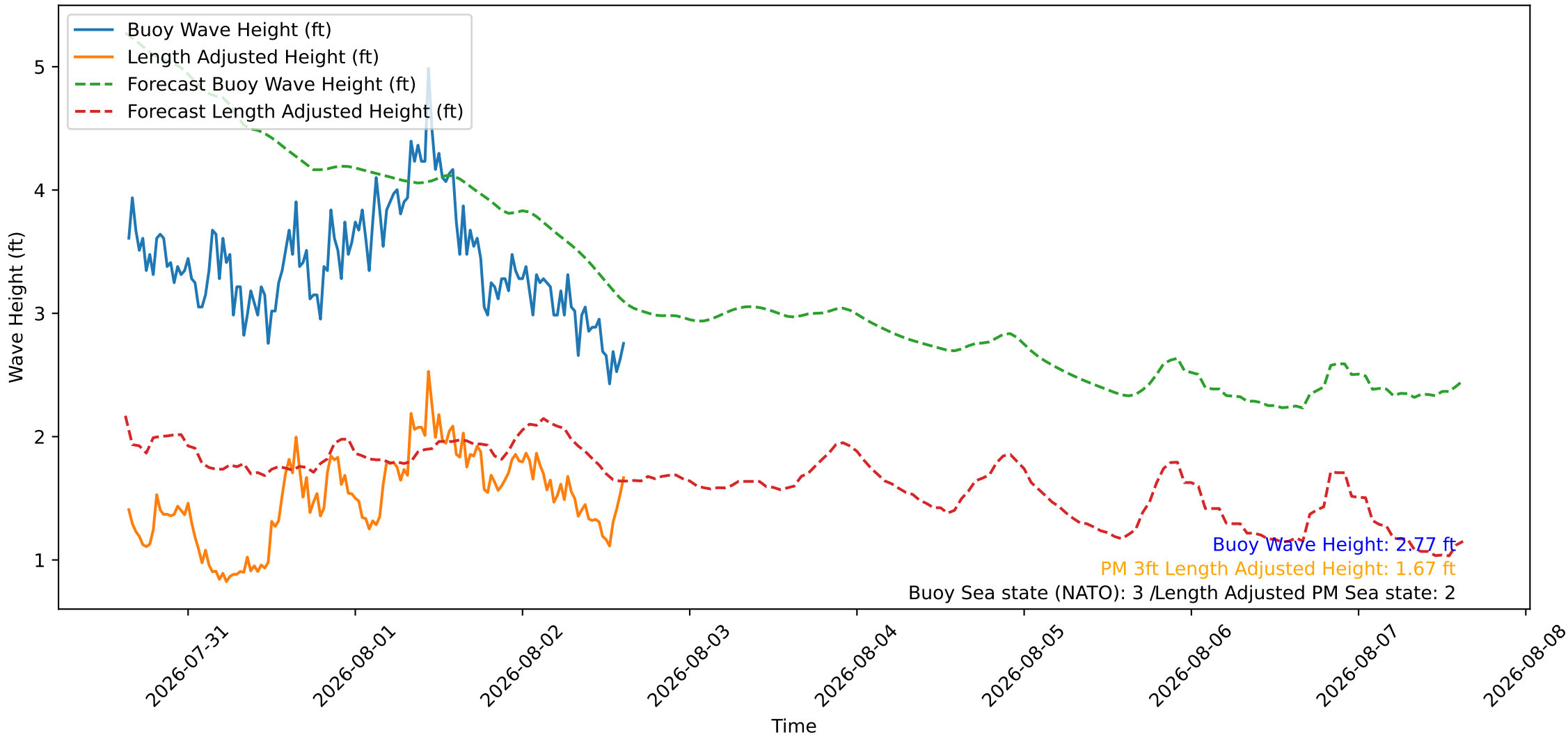
Wave Heights over Time for Green Beach at 2026-08-02 15:21:10
