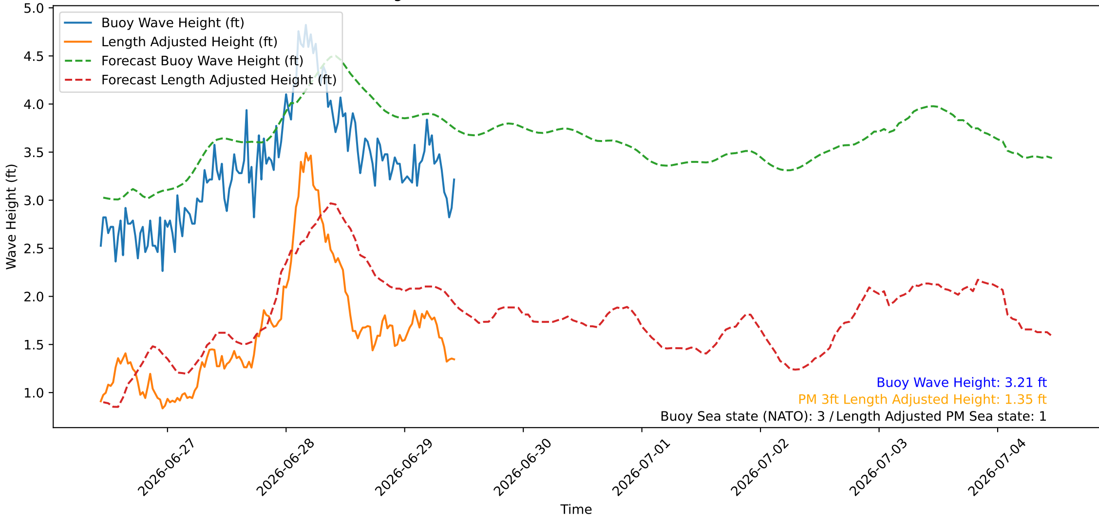
Wave Heights over Time for Green Beach at 2026-06-29 10:41:08
