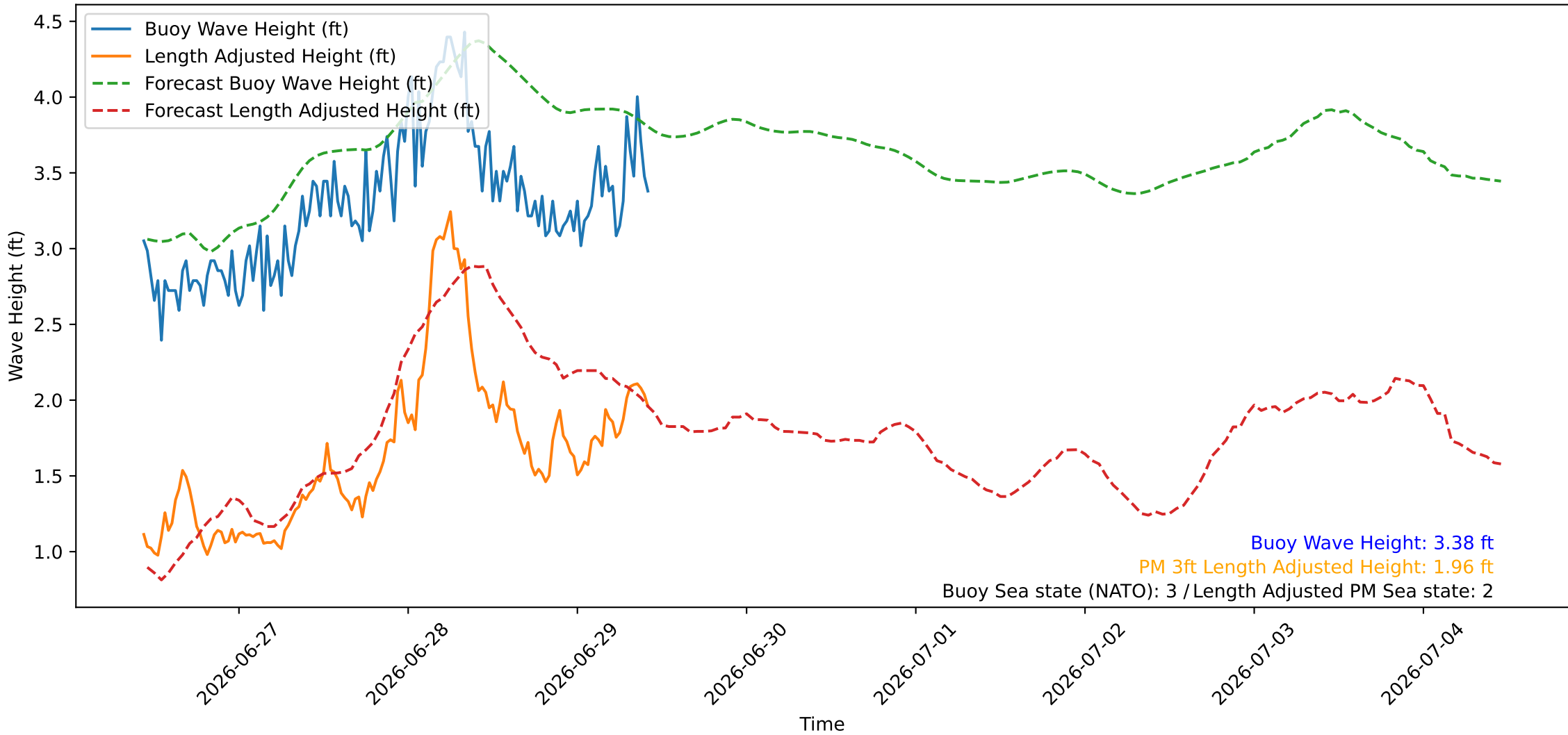
Wave Heights over Time for Oceanside Harbor at 2026-06-29 10:40:25
