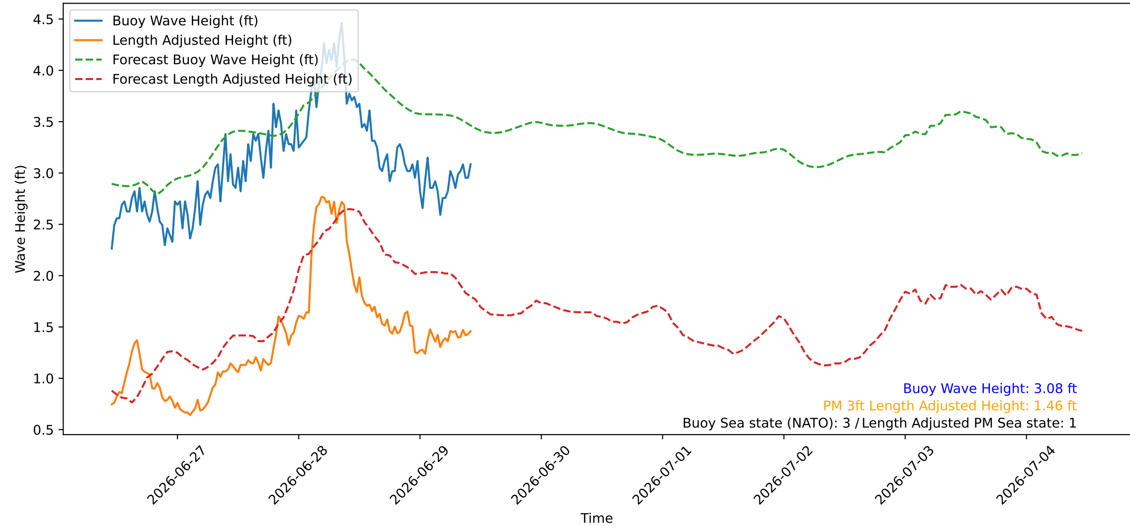
Wave Heights over Time for Red Beach at 2026-06-29 10:40:45
