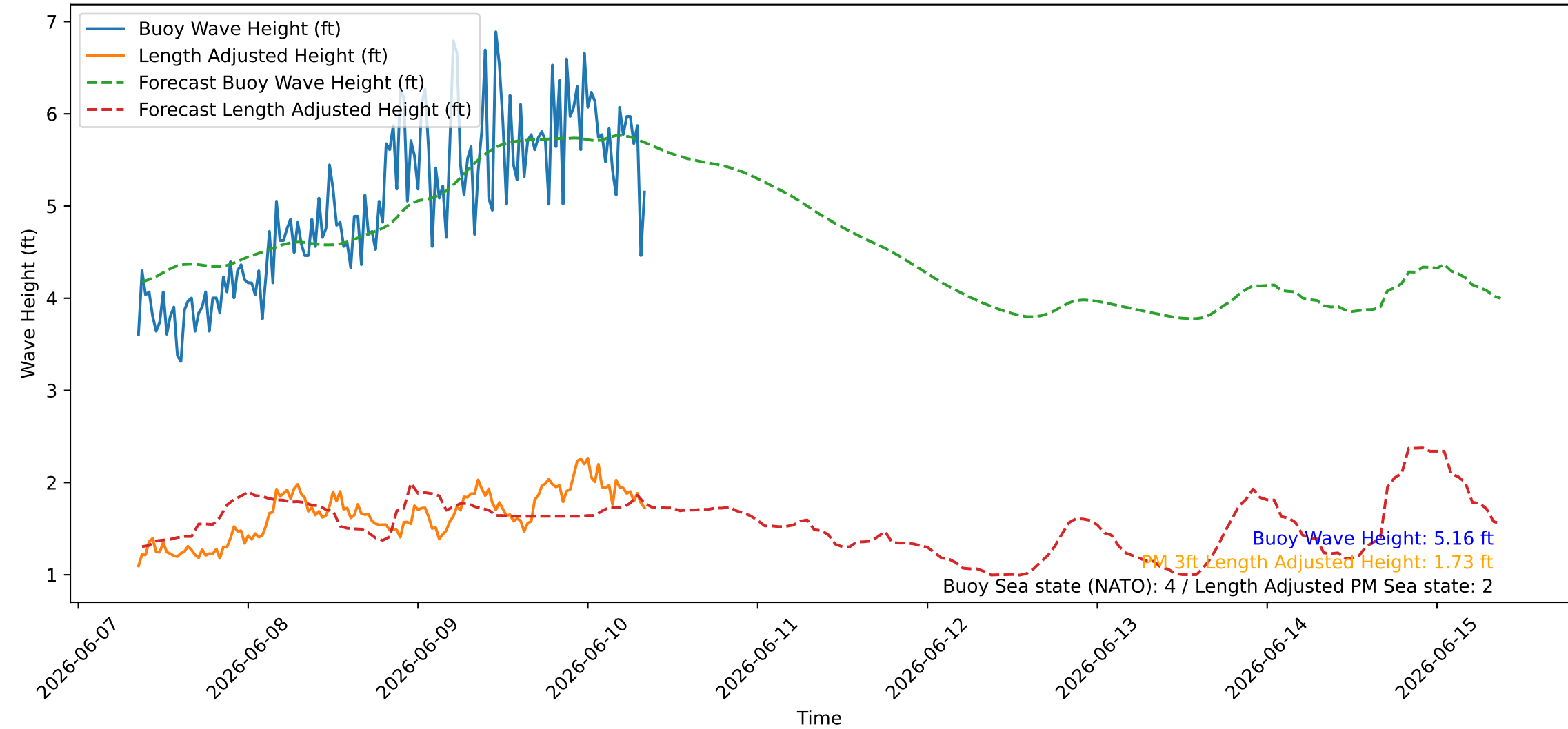
Wave Heights over Time for Green Beach at 2026-06-10 08:41:09
