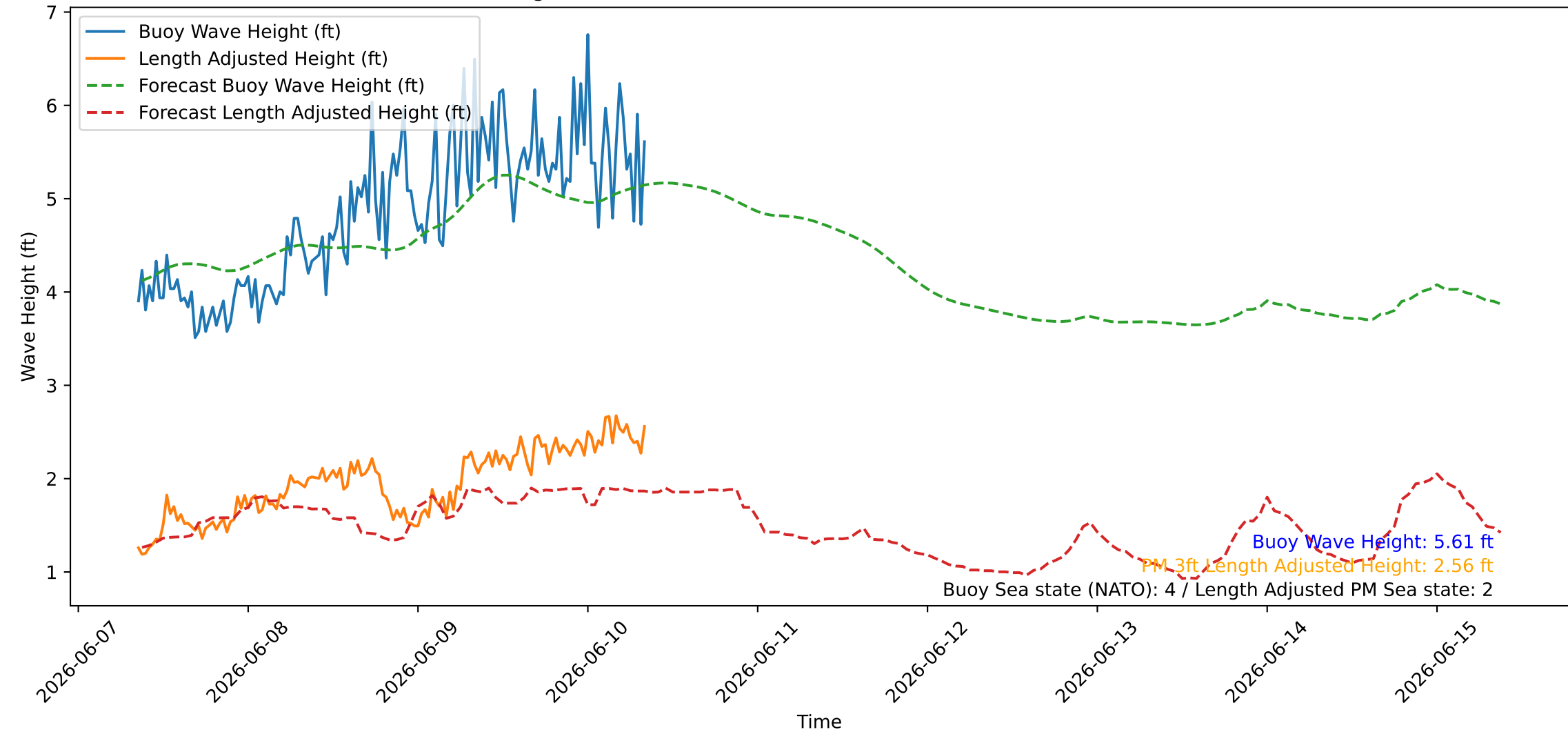
Wave Heights over Time for Oceanside Harbor at 2026-06-10 08:40:26
