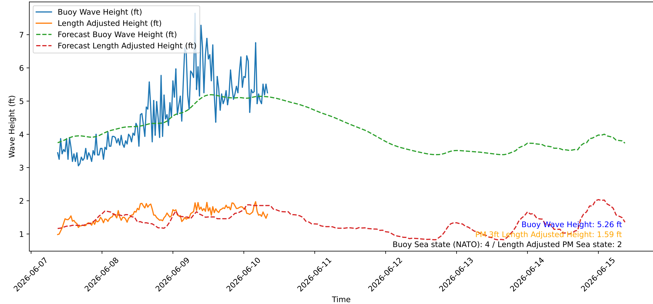
Wave Heights over Time for Red Beach at 2026-06-10 08:40:46
