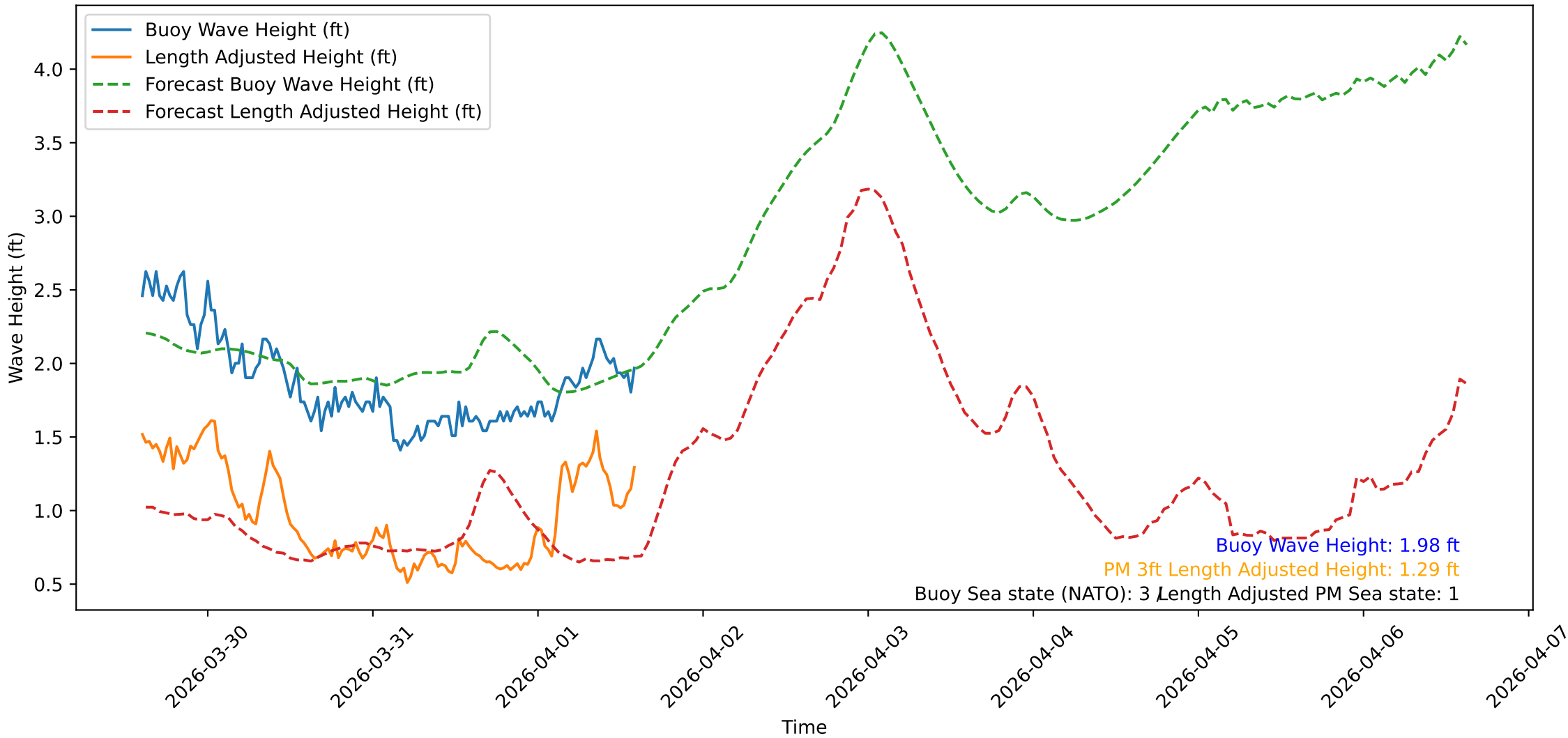
Wave Heights over Time for Green Beach at 2026-04-01 14:41:09
