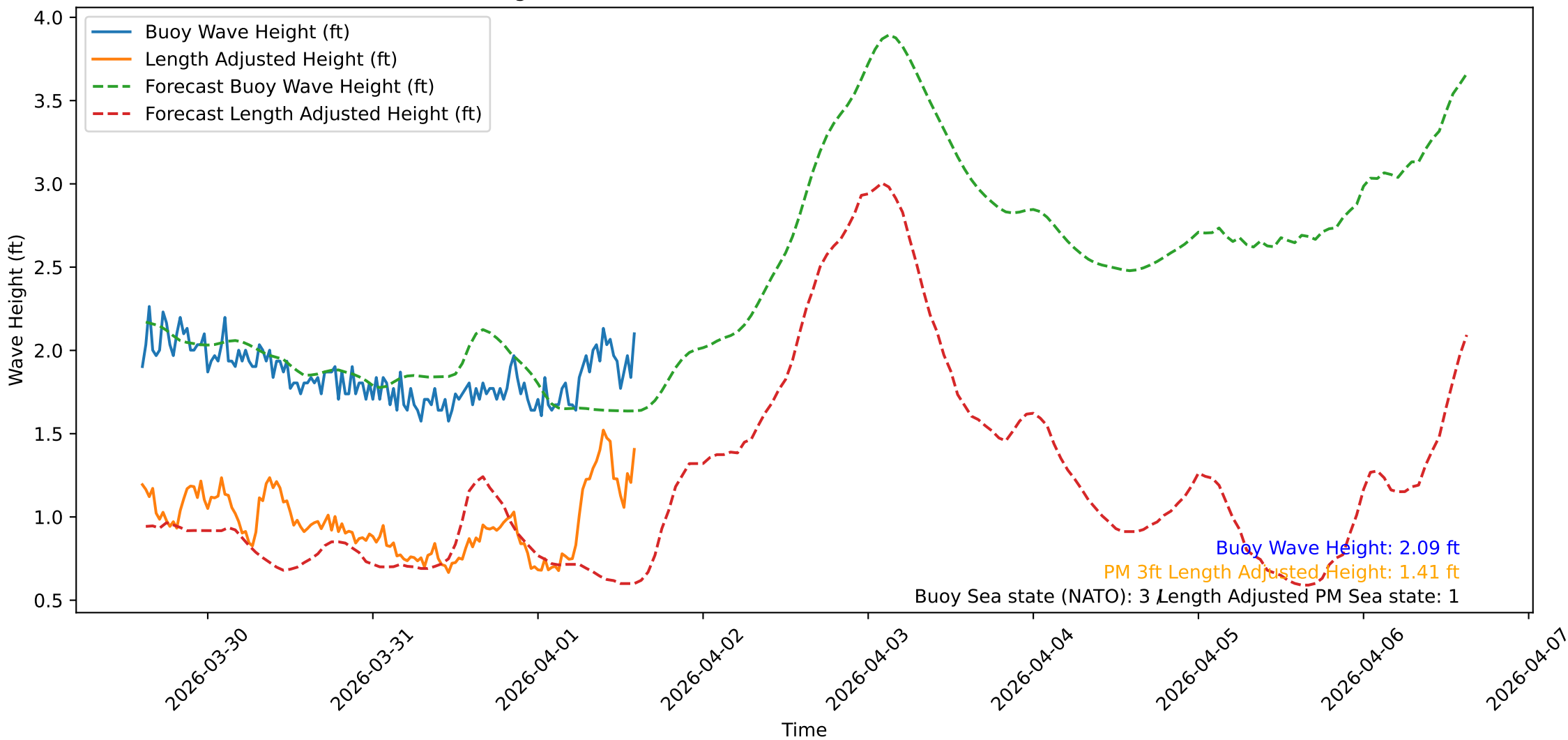
Wave Heights over Time for Oceanside Harbor at 2026-04-01 14:40:31
