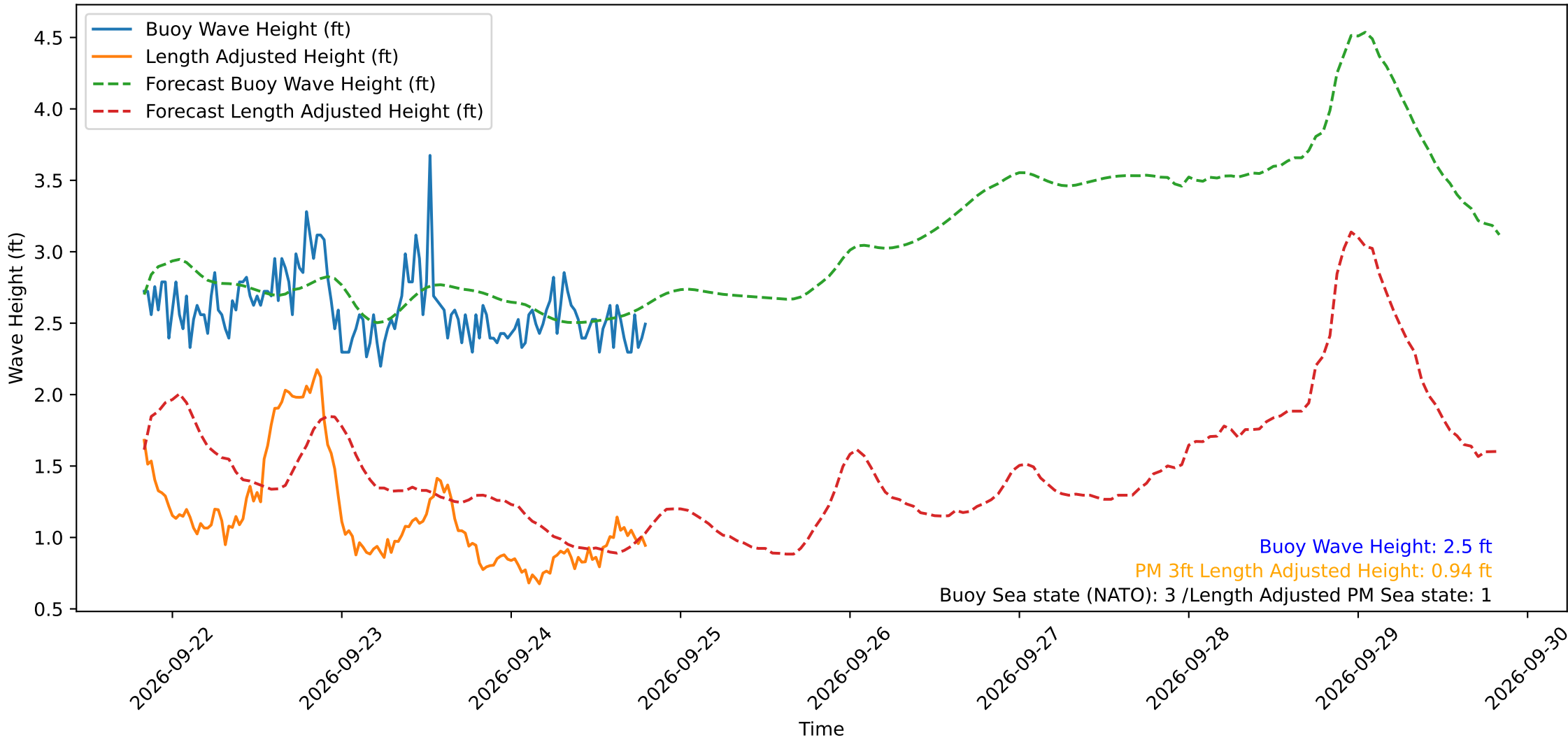
Wave Heights over Time for Red Beach at 2026-09-24 19:50:50
