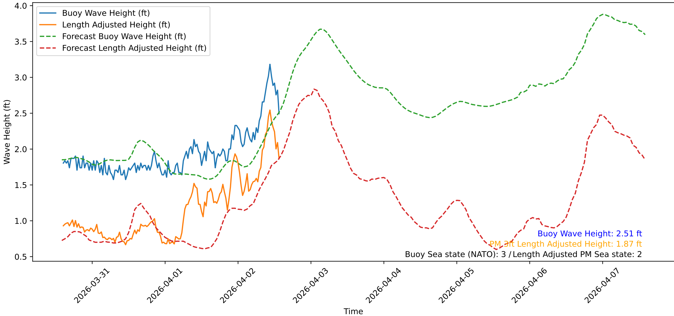
Wave Heights over Time for Oceanside Harbor at 2026-04-02 14:20:31
