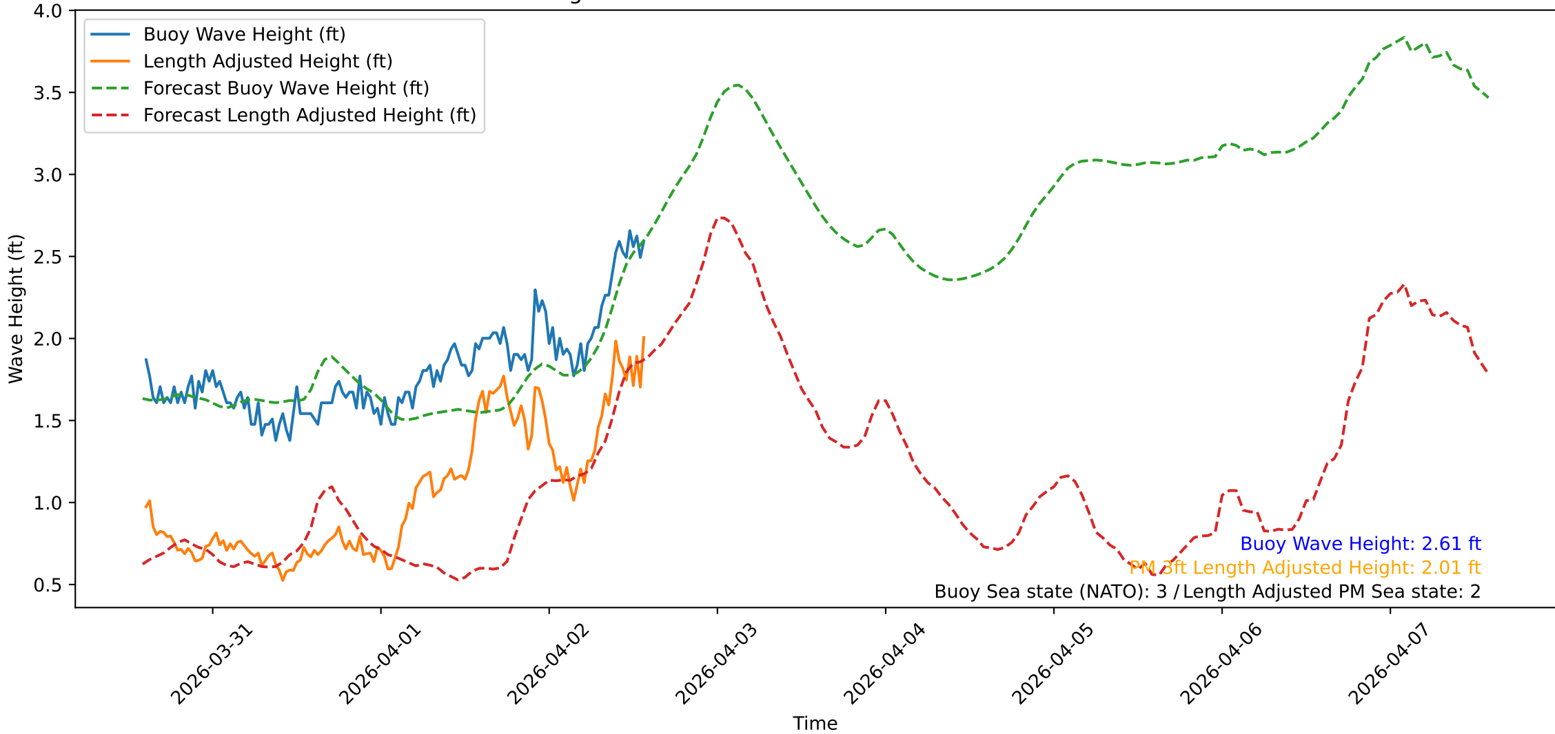
Wave Heights over Time for Red Beach at 2026-04-02 14:20:48
