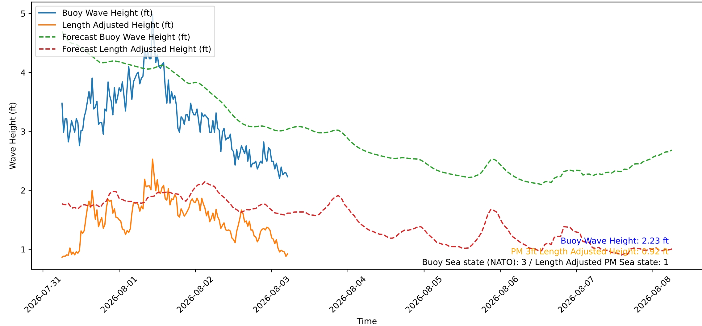
Wave Heights over Time for Green Beach at 2026-08-03 05:51:09
