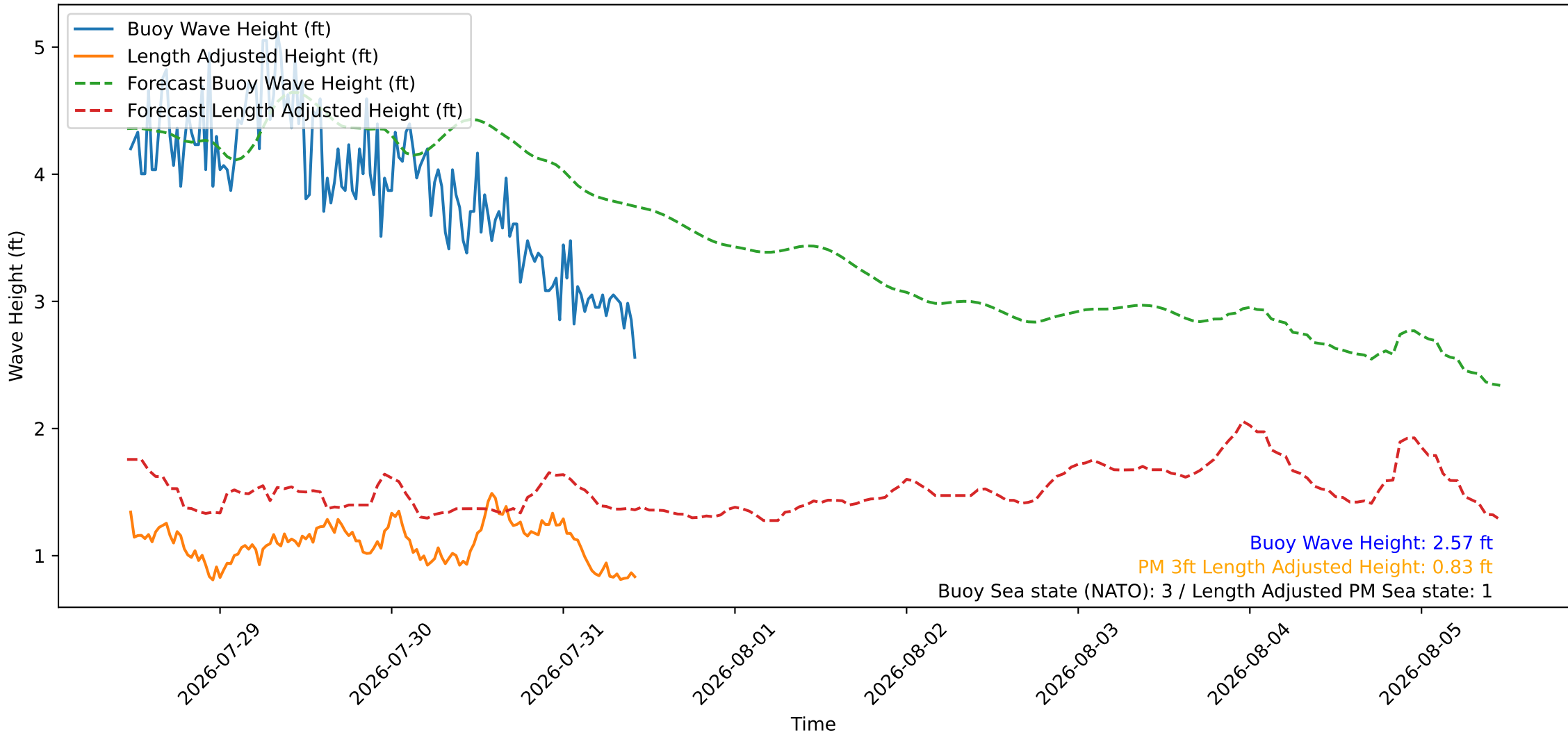
Wave Heights over Time for Red Beach at 2026-07-31 11:10:46
