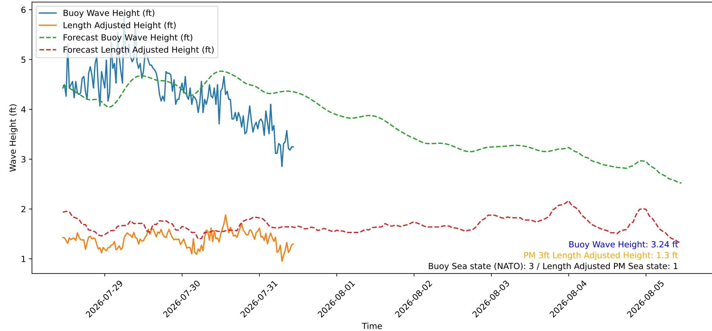
Wave Heights over Time for Oceanside Harbor at 2026-07-31 11:10:26
