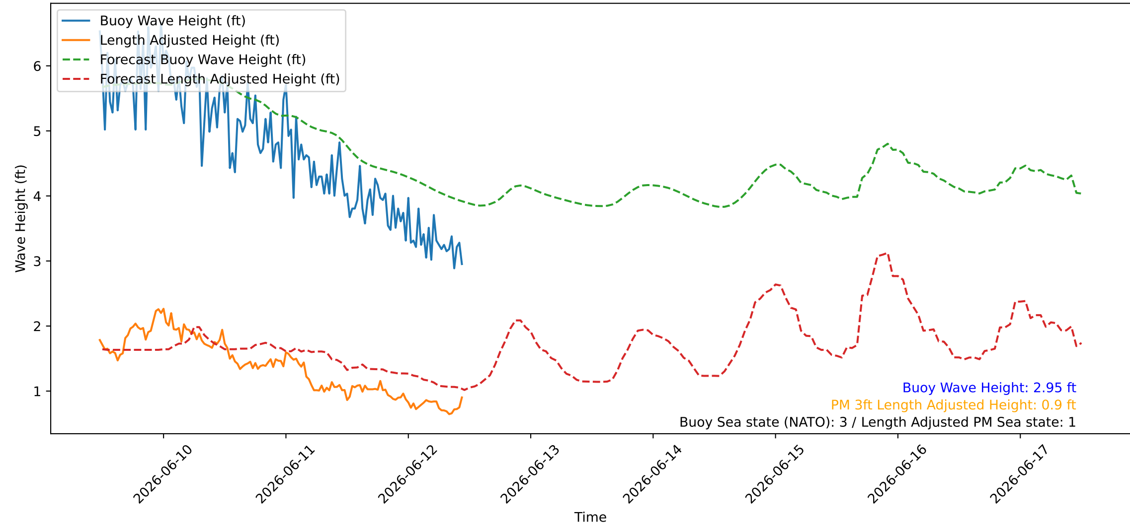
Wave Heights over Time for Green Beach at 2026-06-12 11:31:09
