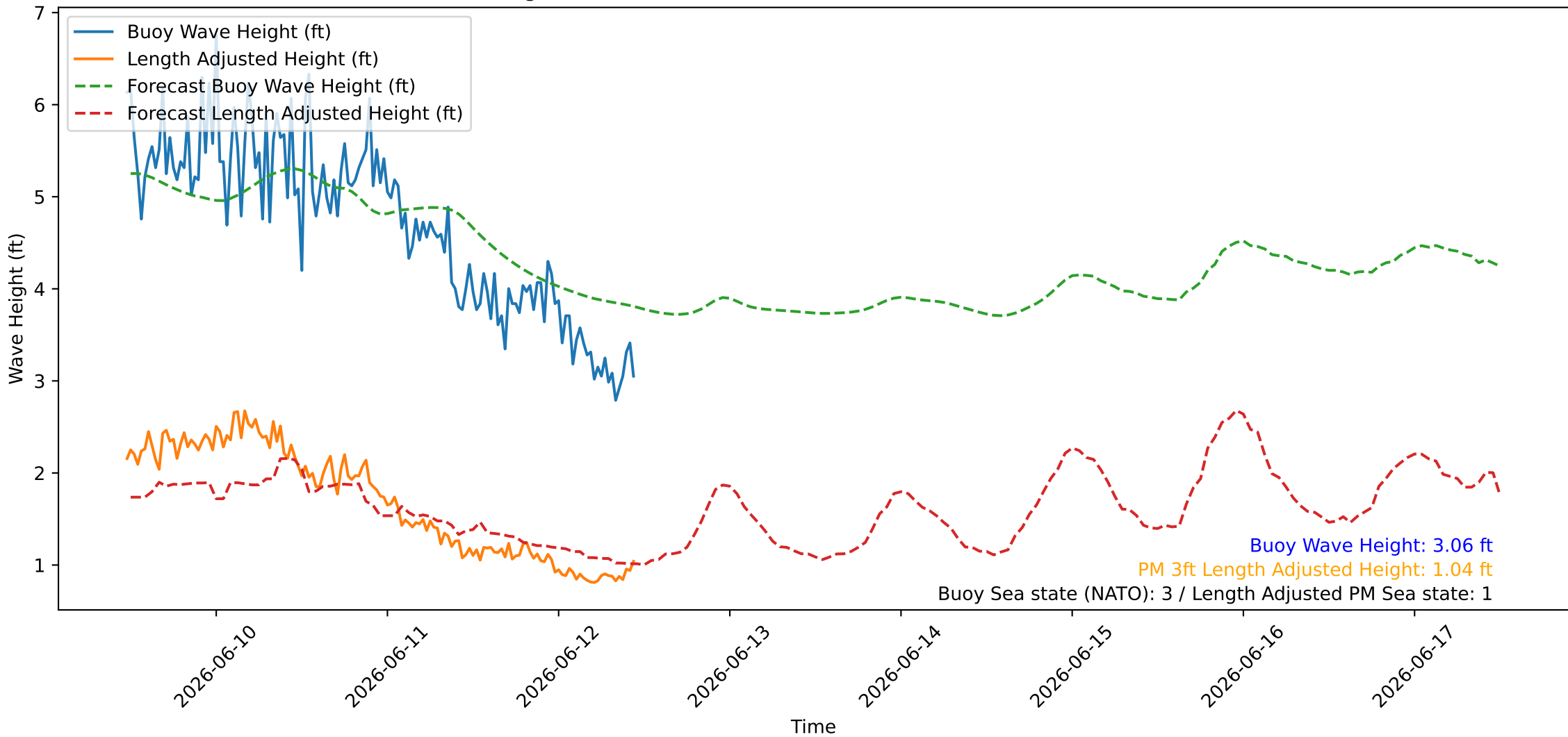
Wave Heights over Time for Oceanside Harbor at 2026-06-12 11:30:26
