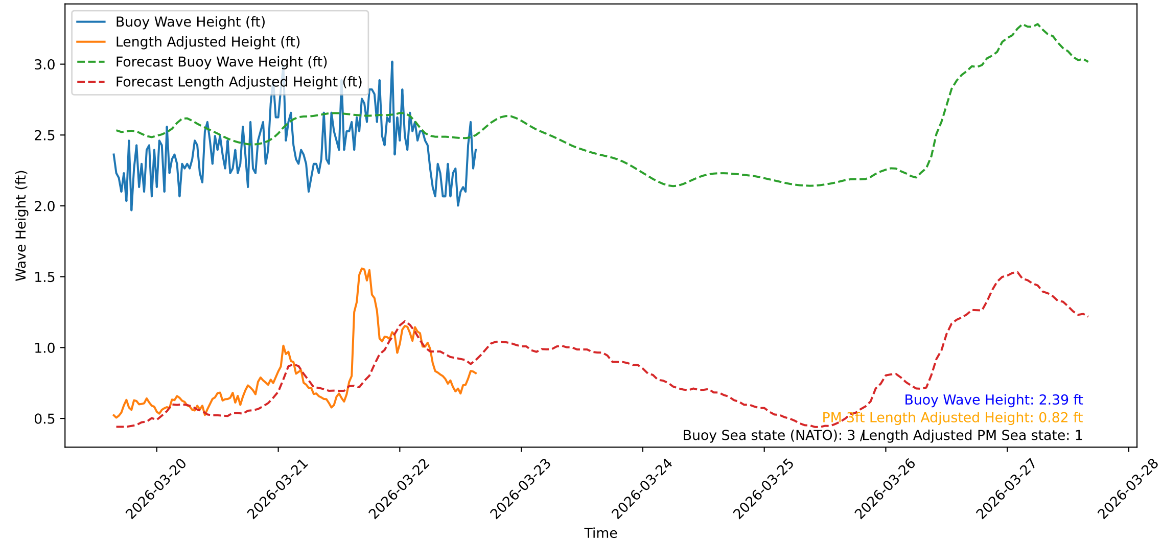
Wave Heights over Time for Oceanside Harbor at 2026-03-22 15:40:31
