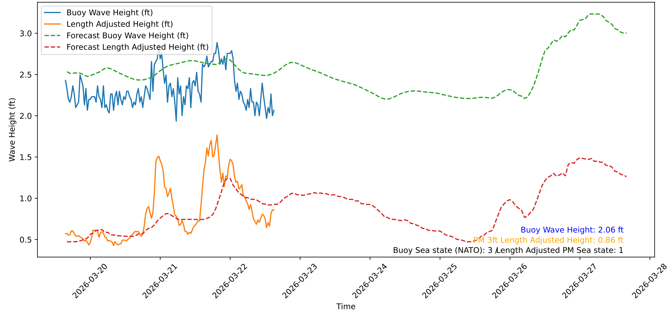
Wave Heights over Time for Green Beach at 2026-03-22 15:41:10
