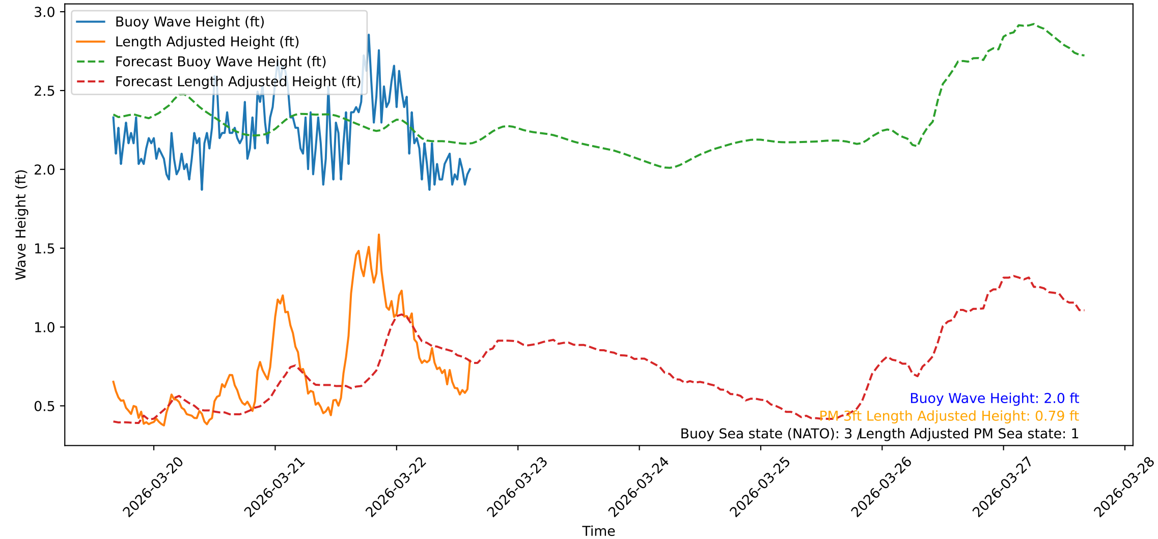
Wave Heights over Time for Red Beach at 2026-03-22 15:40:47
