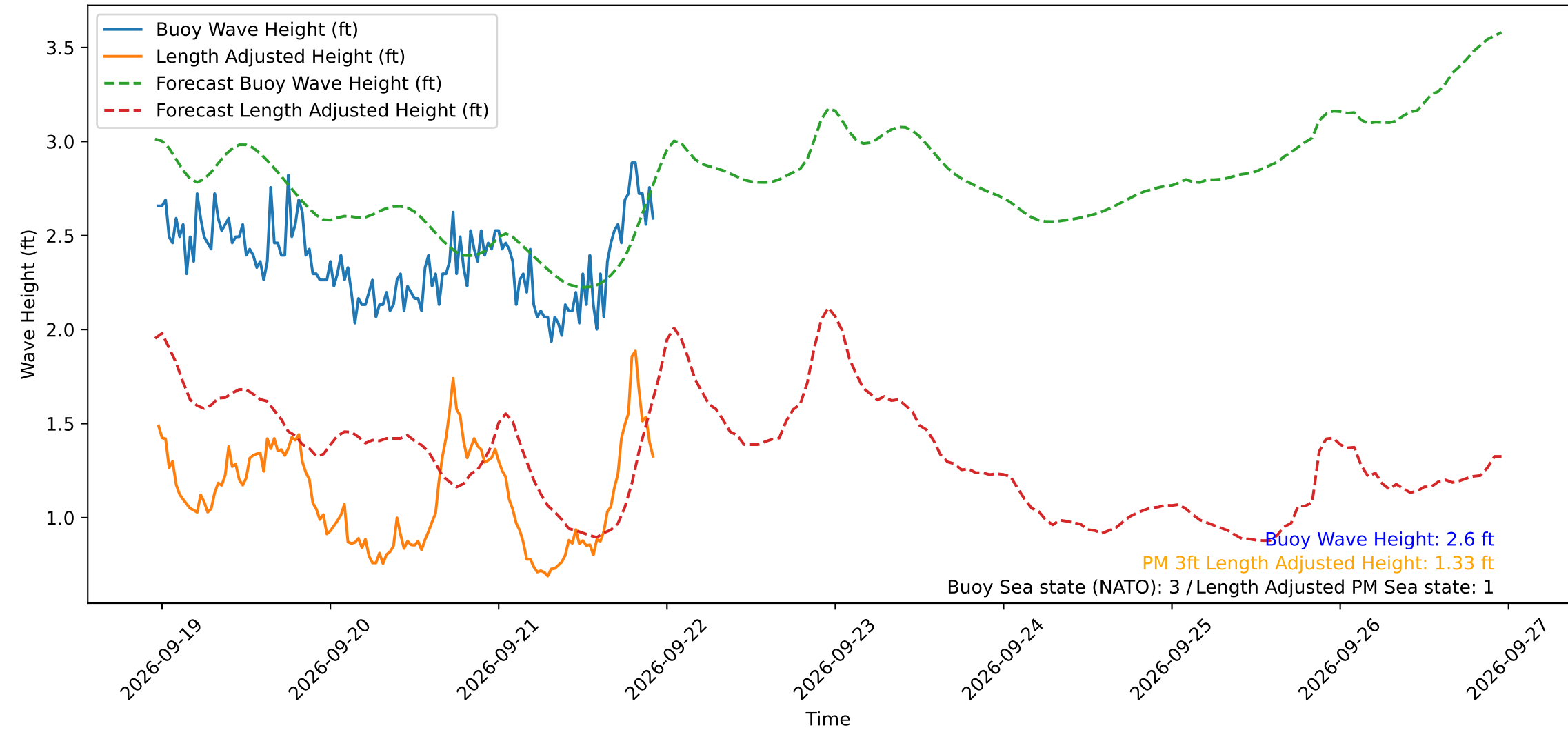
Wave Heights over Time for Red Beach at 2026-09-21 23:00:49
