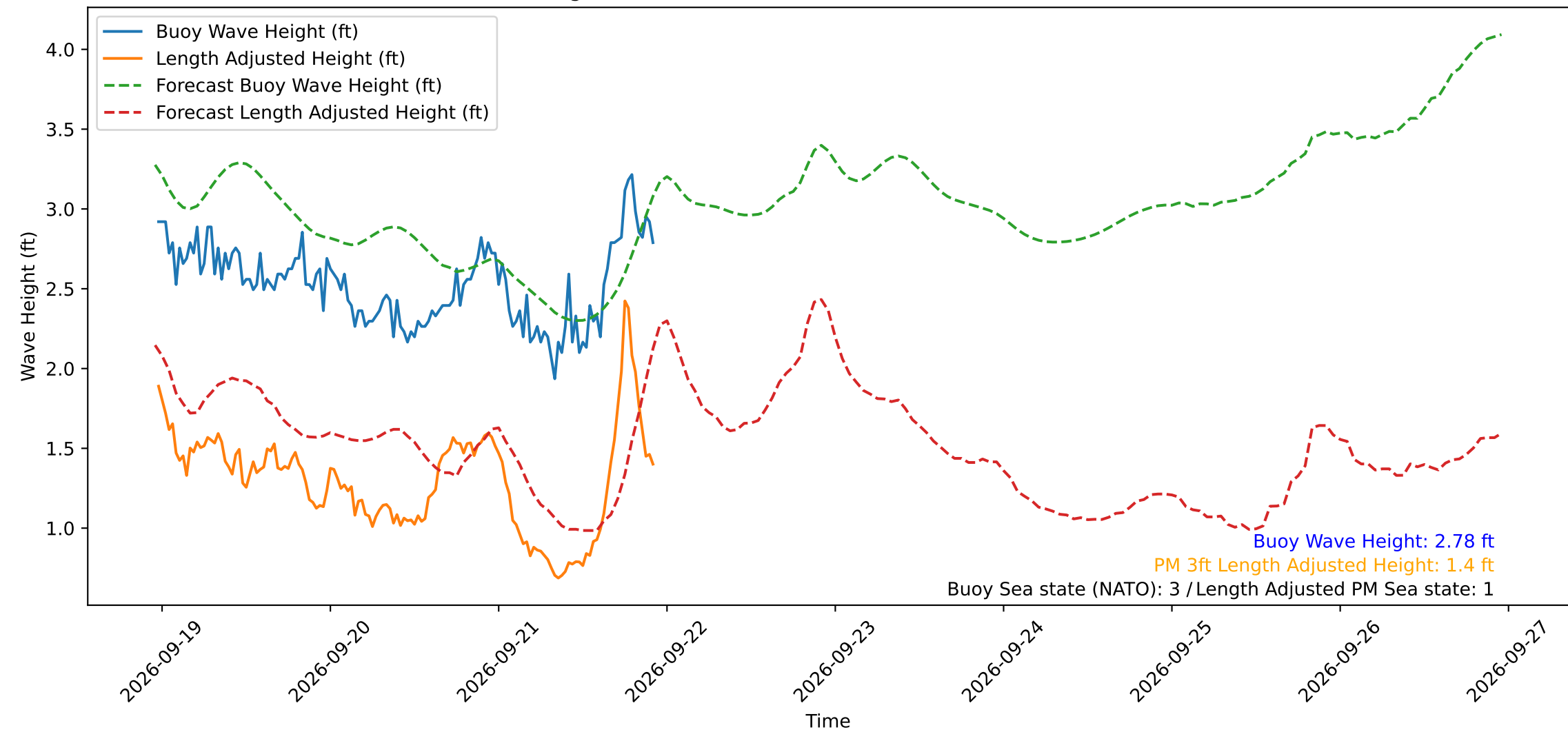
Wave Heights over Time for Green Beach at 2026-09-21 23:01:11
