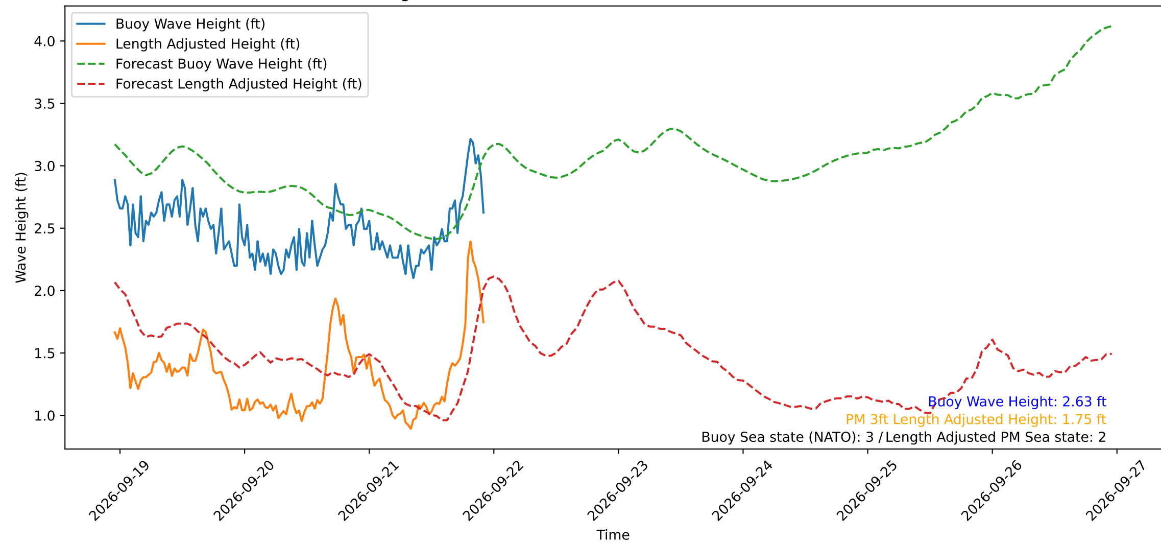
Wave Heights over Time for Oceanside Harbor at 2026-09-21 23:00:29
