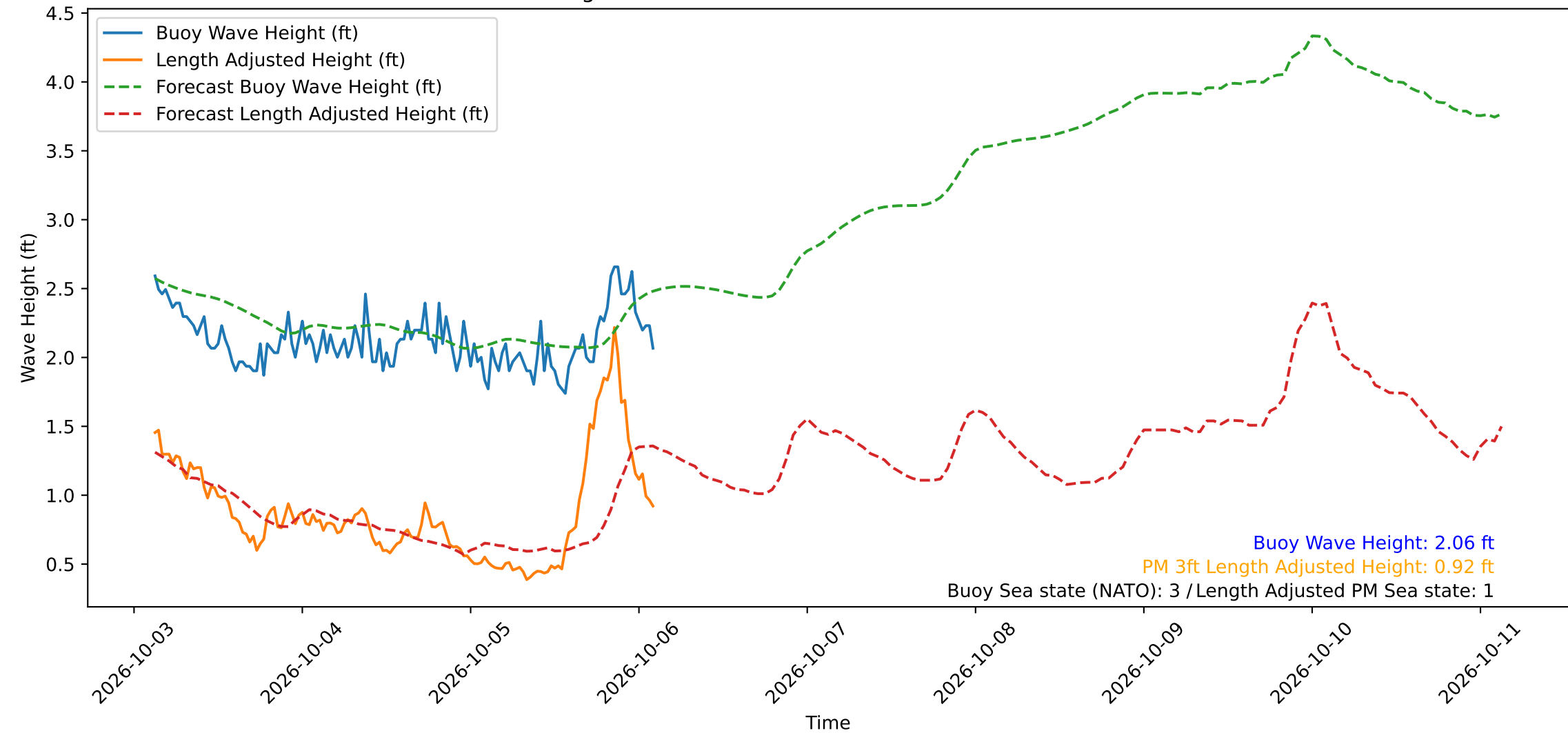
Wave Heights over Time for Red Beach at 2026-10-06 02:50:51
