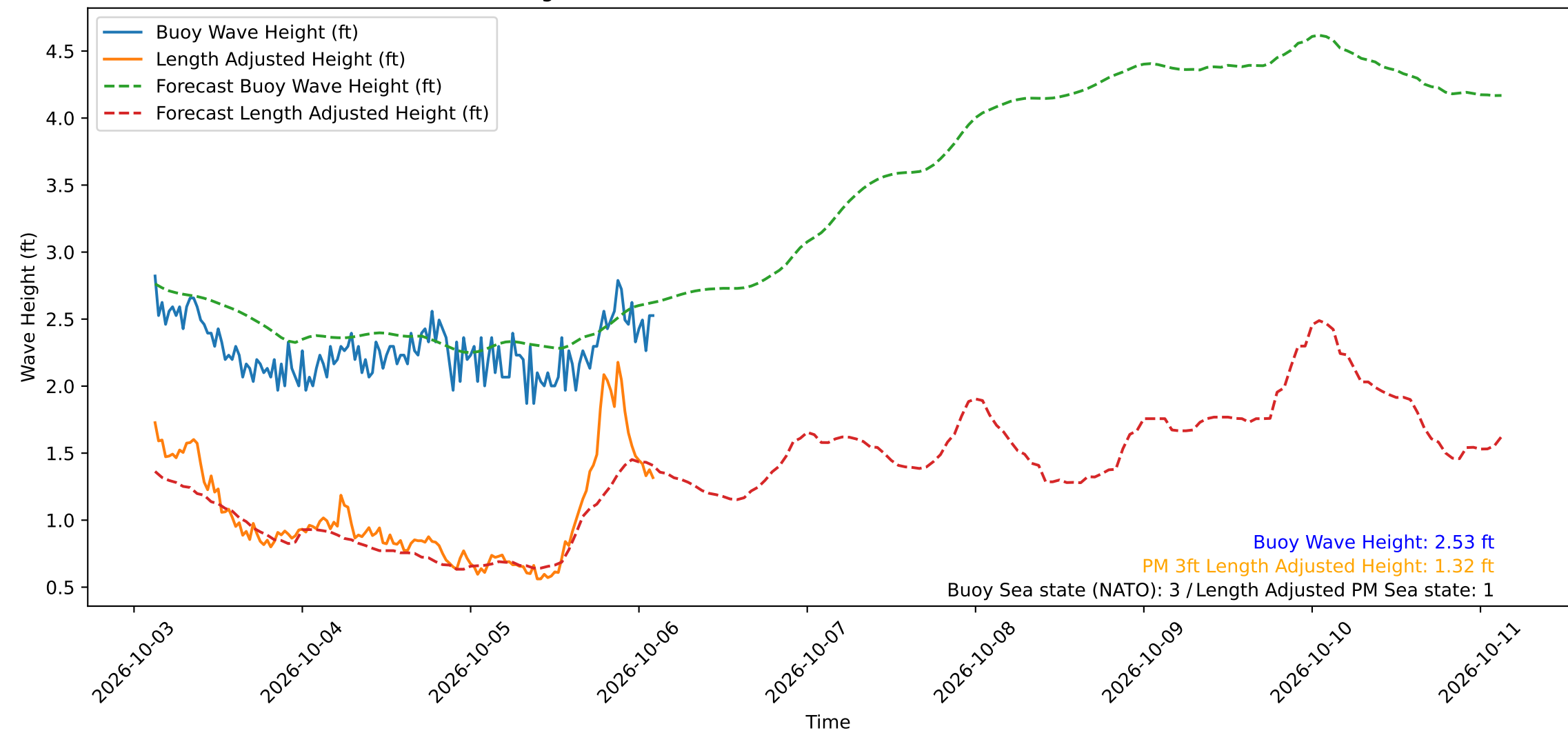
Wave Heights over Time for Oceanside Harbor at 2026-10-06 02:50:30
