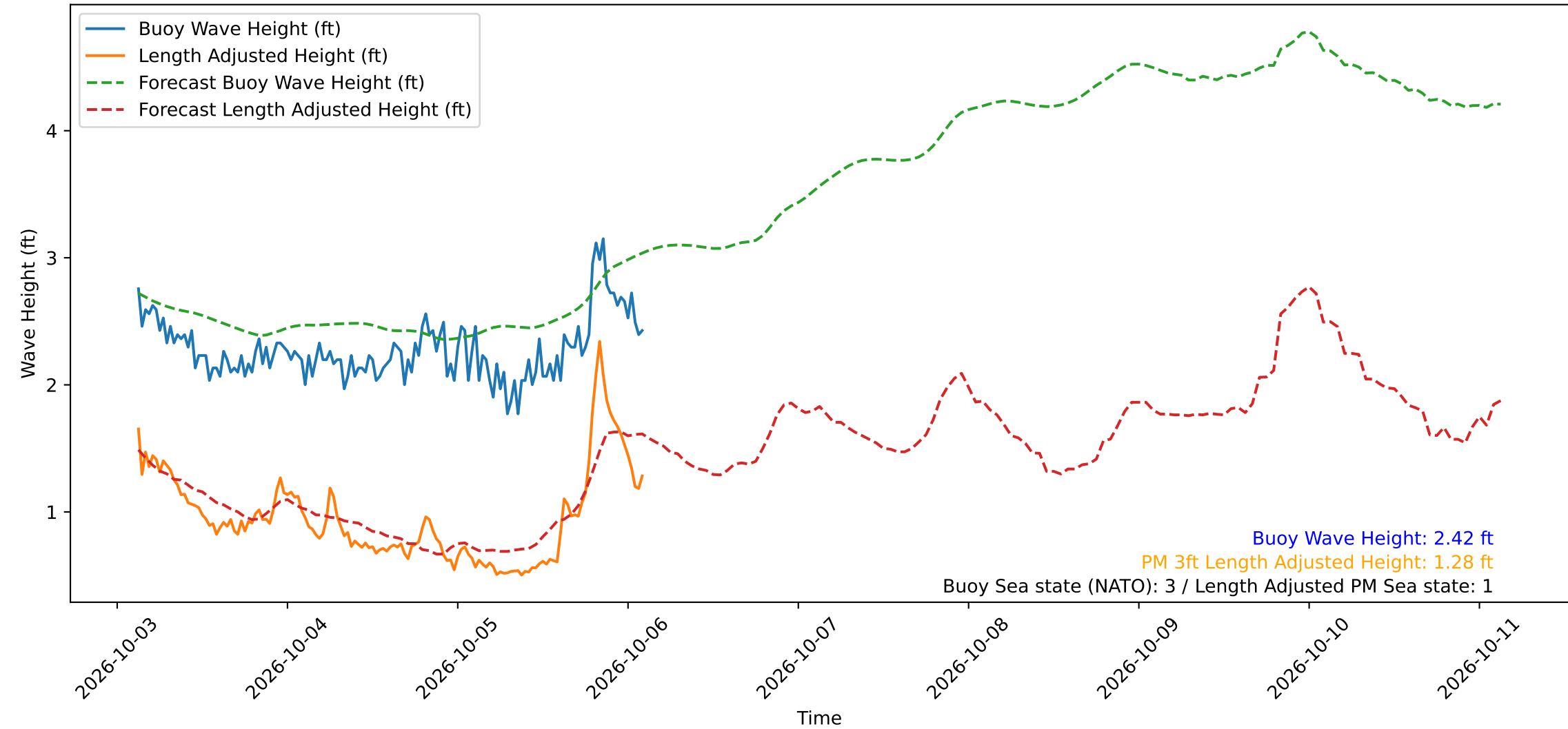
Wave Heights over Time for Green Beach at 2026-10-06 02:51:15
