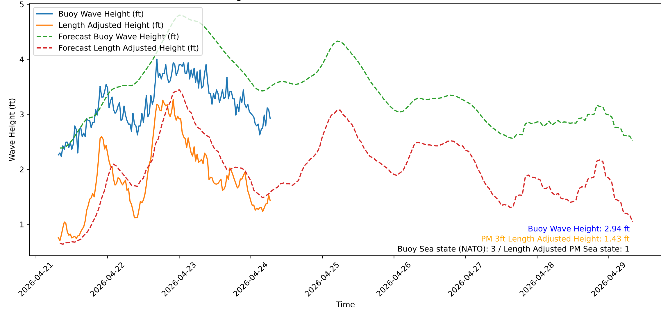
Wave Heights over Time for Green Beach at 2026-04-24 07:31:12
