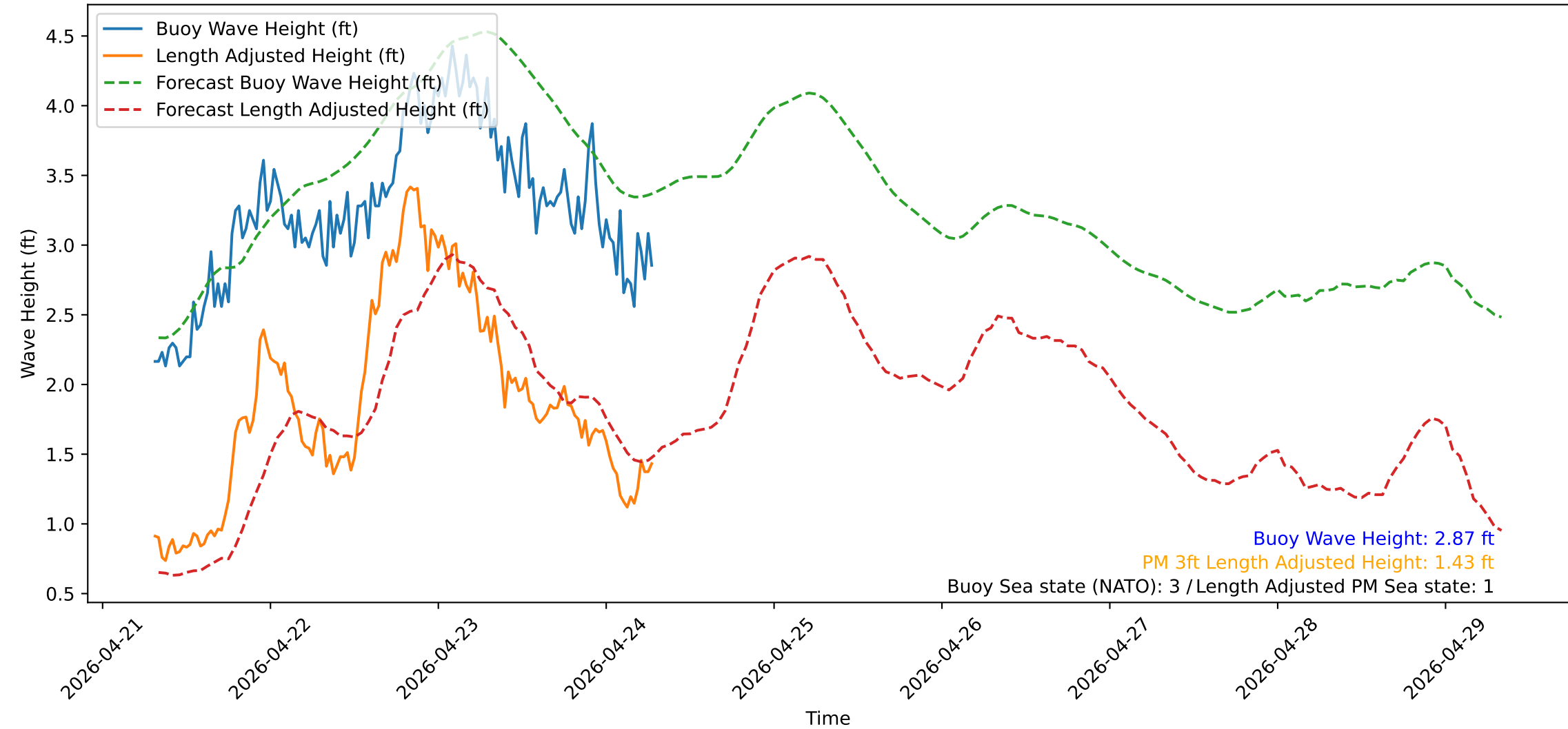
Wave Heights over Time for Oceanside Harbor at 2026-04-24 07:30:31
