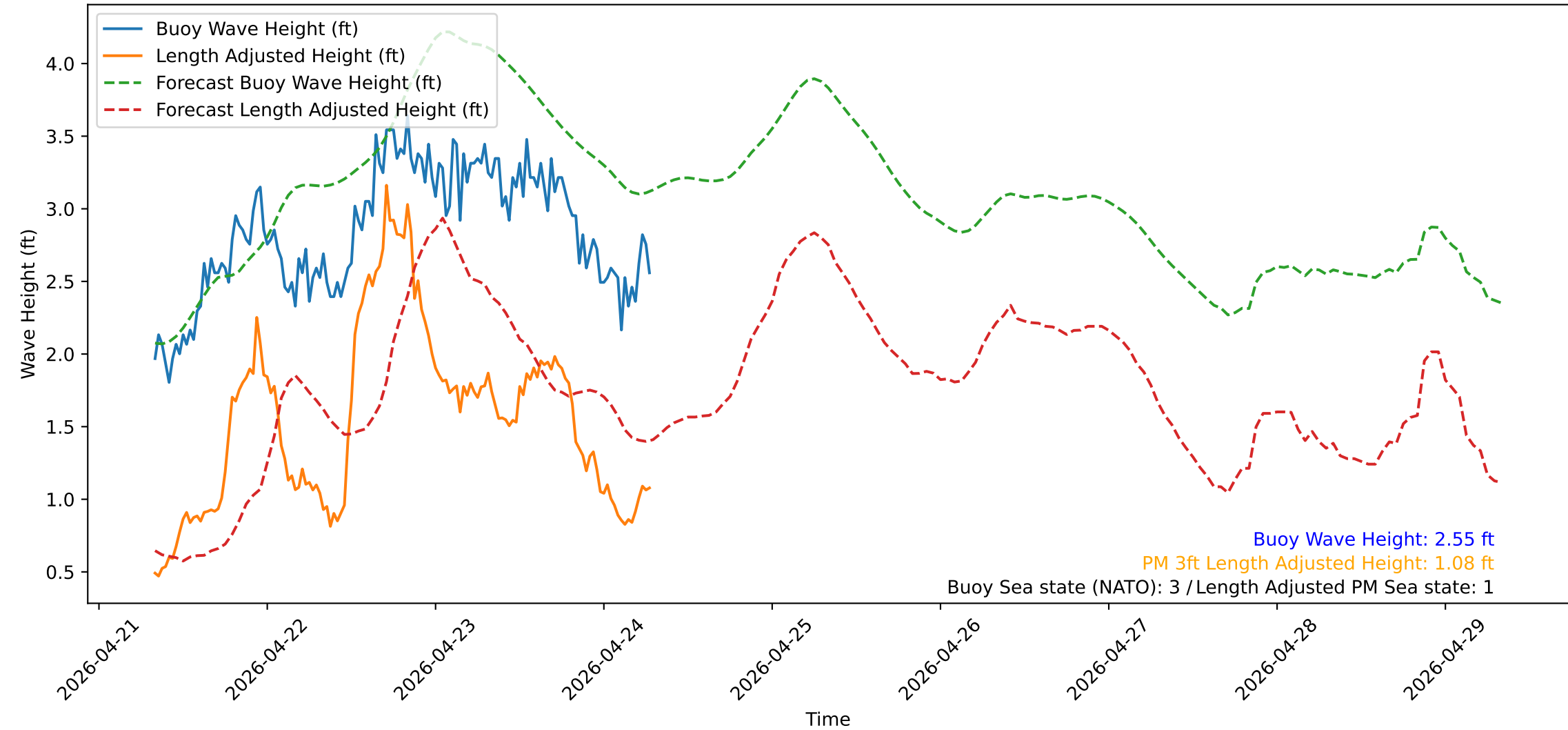
Wave Heights over Time for Red Beach at 2026-04-24 07:30:50
