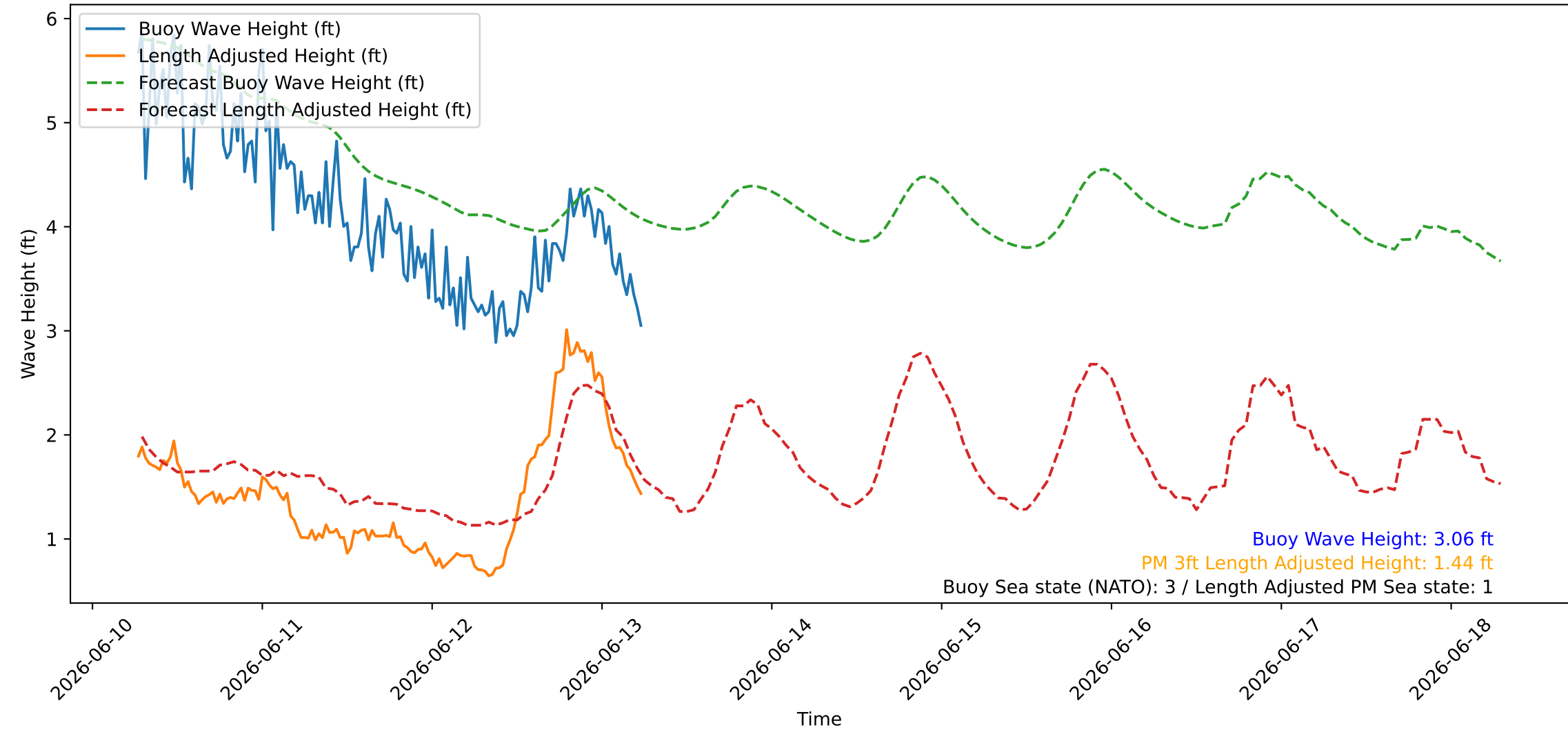
Wave Heights over Time for Green Beach at 2026-06-13 06:31:08
