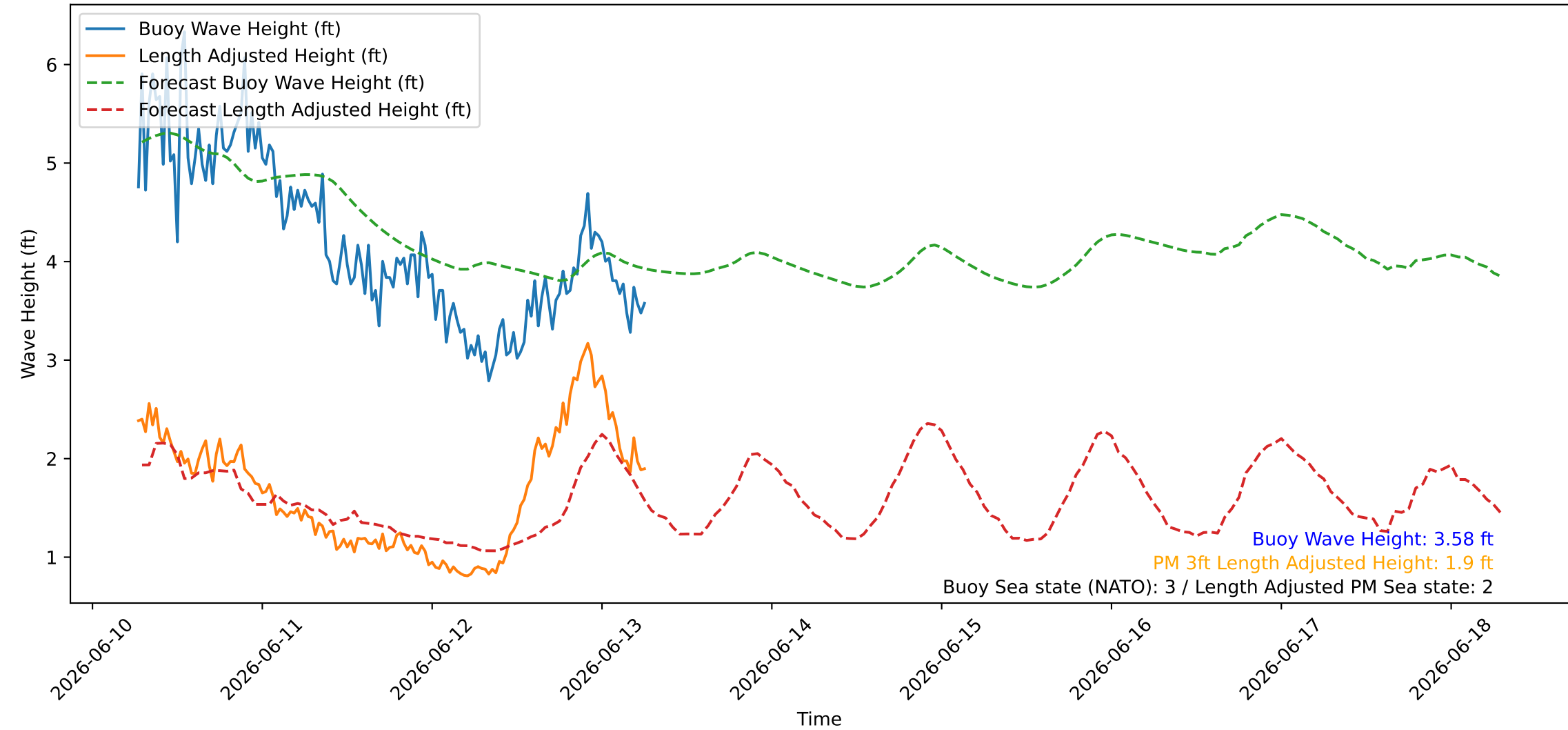
Wave Heights over Time for Oceanside Harbor at 2026-06-13 06:30:26
