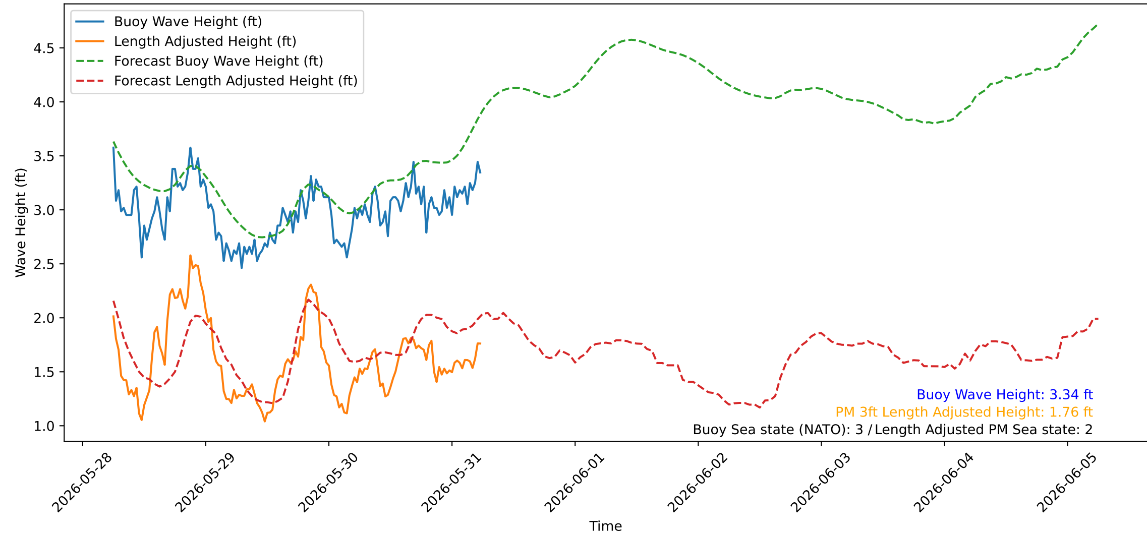
Wave Heights over Time for Green Beach at 2026-05-31 06:11:07
