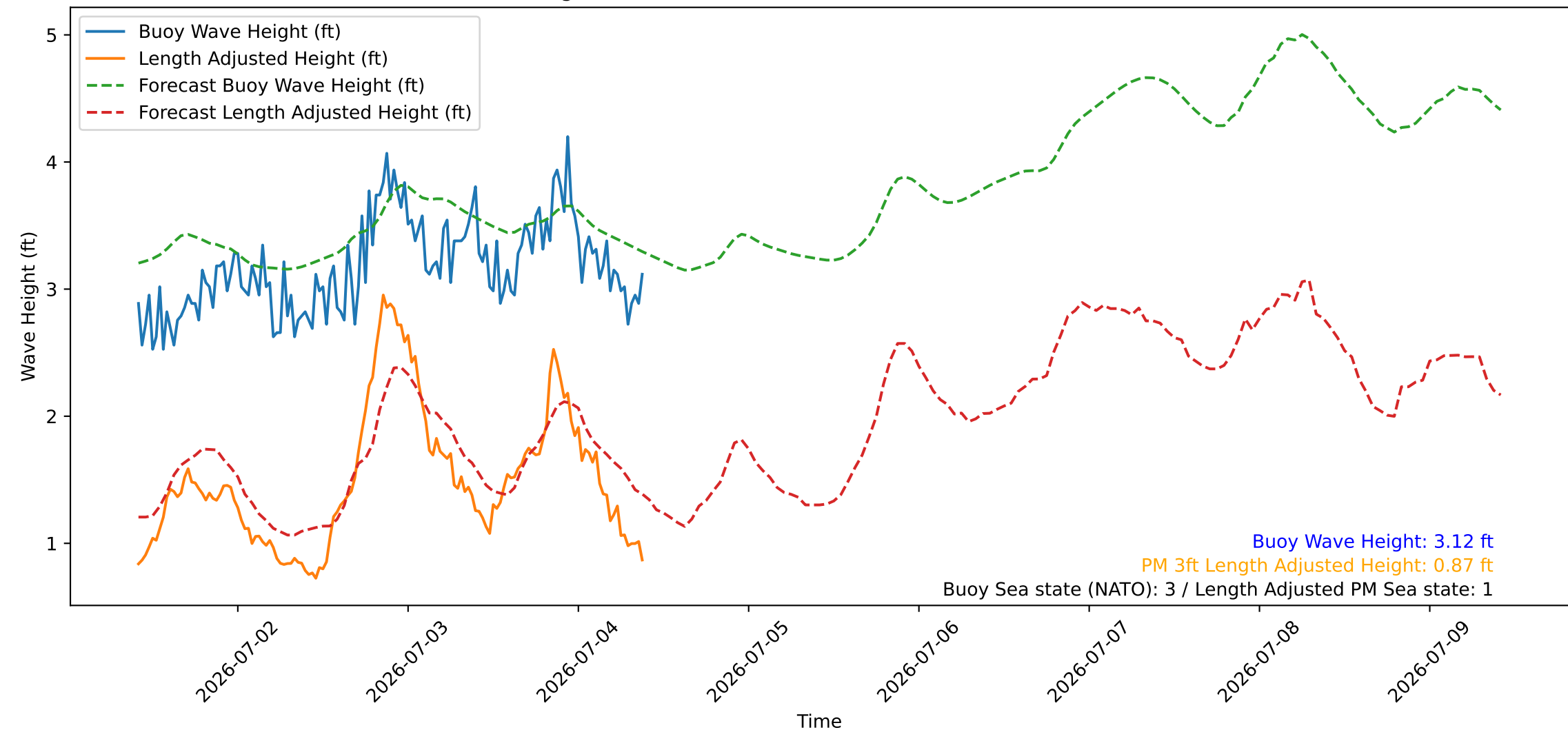
Wave Heights over Time for Green Beach at 2026-07-04 09:51:09
