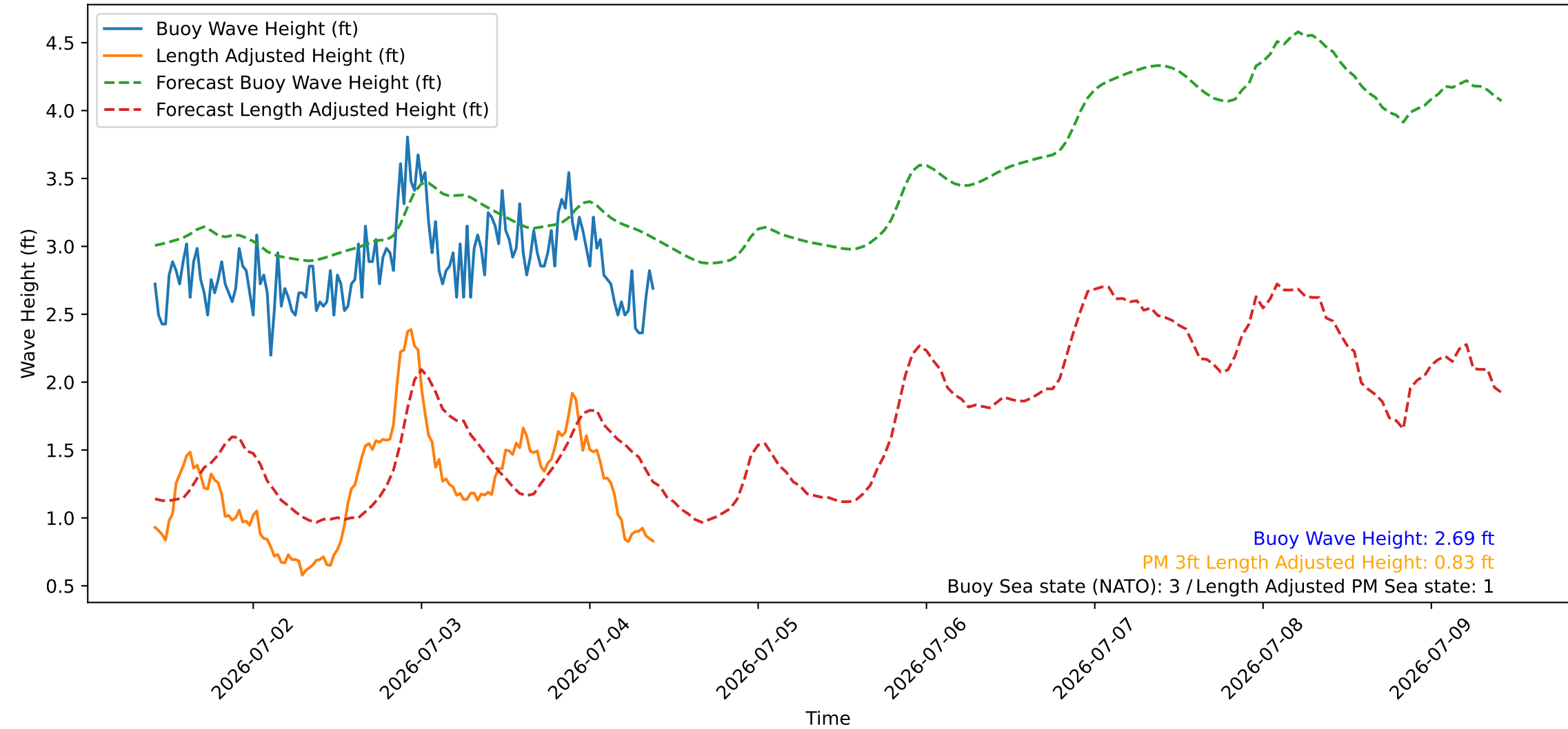
Wave Heights over Time for Red Beach at 2026-07-04 09:50:47
