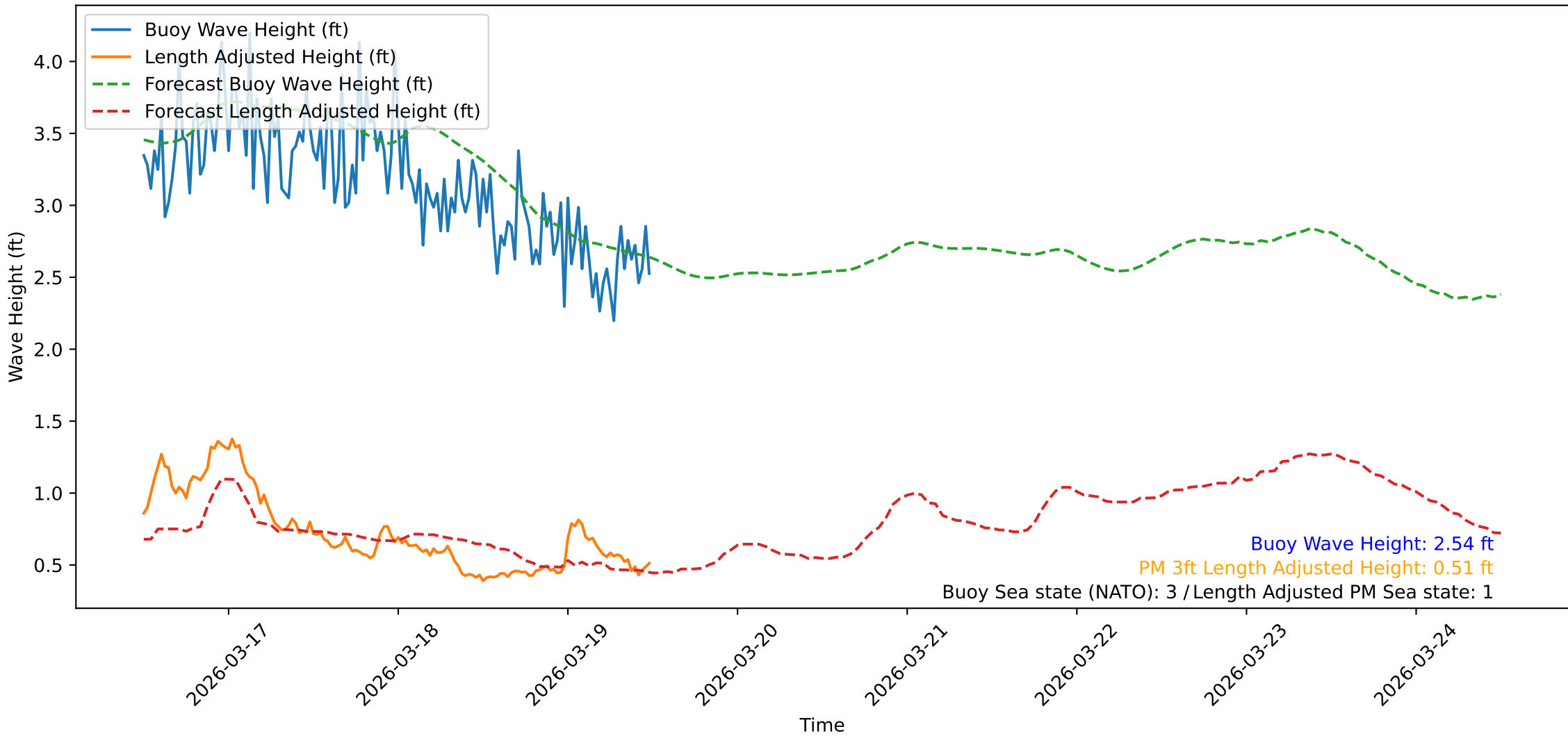
Wave Heights over Time for Green Beach at 2026-03-19 12:11:10
