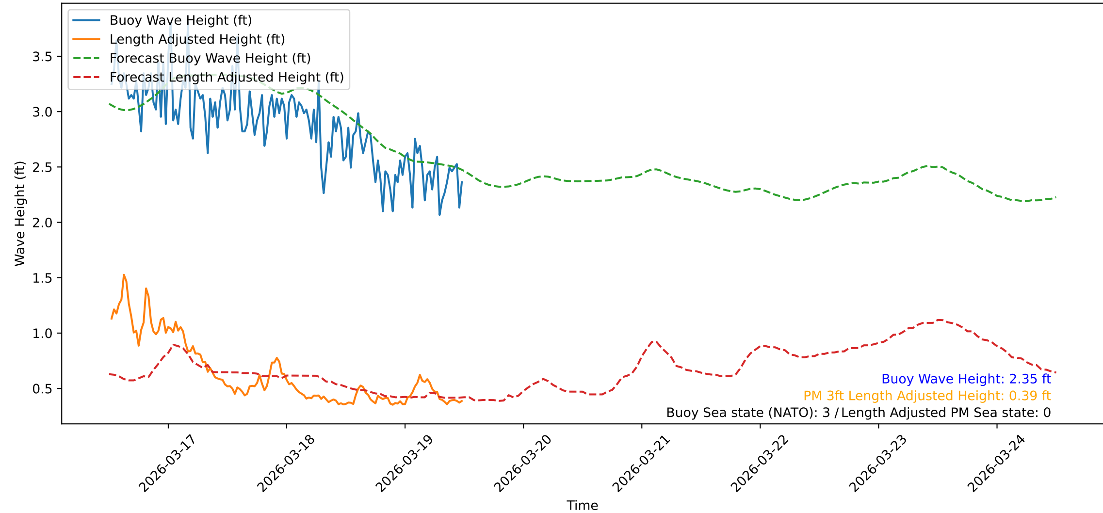
Wave Heights over Time for Red Beach at 2026-03-19 12:10:48
