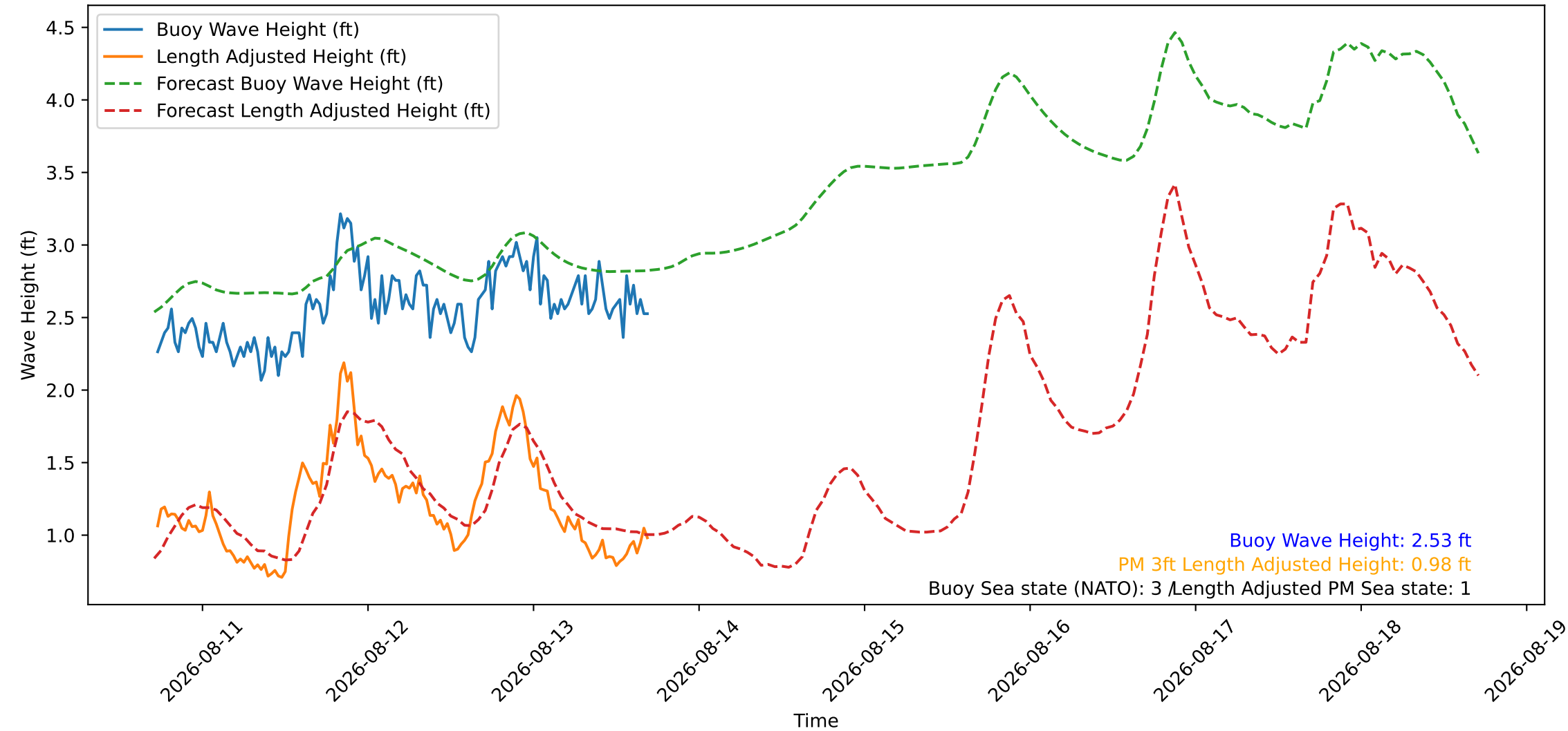
Wave Heights over Time for Green Beach at 2026-08-13 17:21:08
