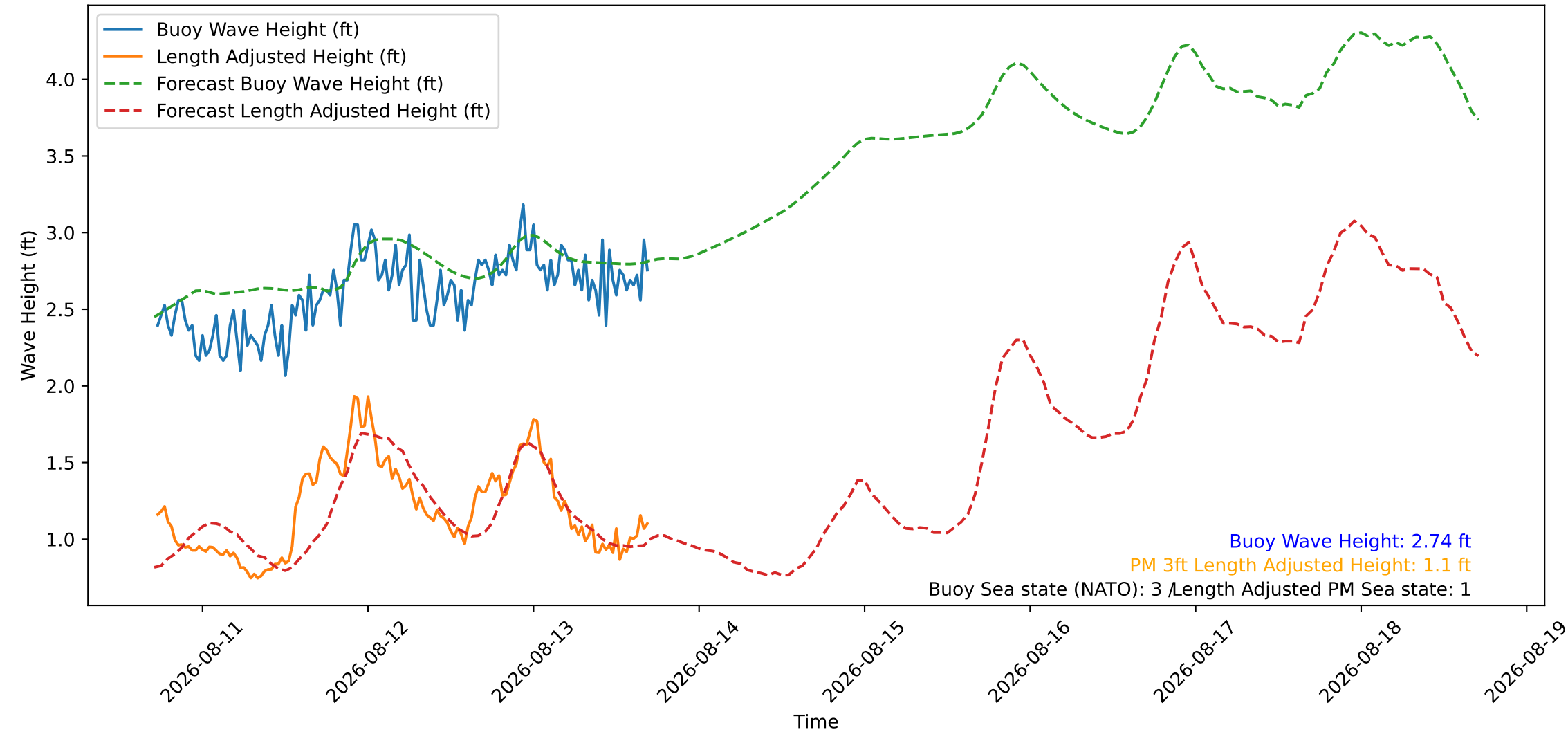
Wave Heights over Time for Oceanside Harbor at 2026-08-13 17:20:26
