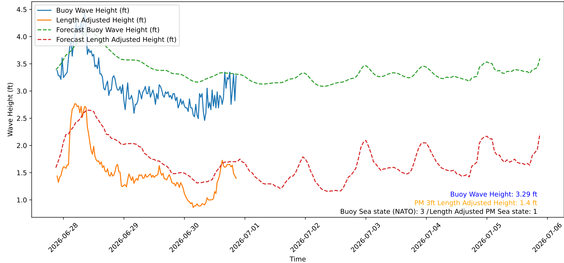
Wave Heights over Time for Red Beach at 2026-06-30 21:10:46
