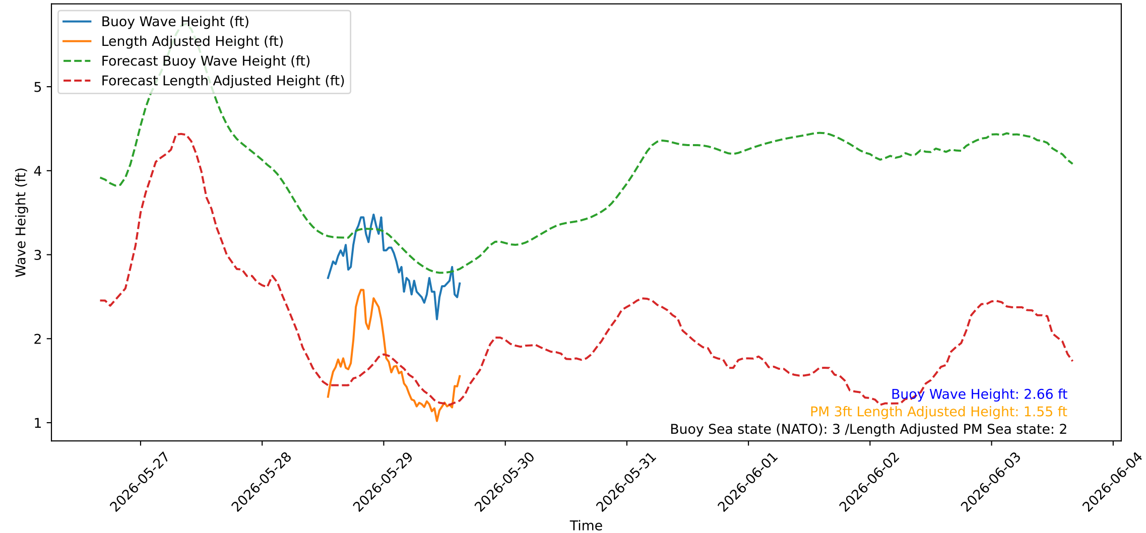
Wave Heights over Time for Oceanside Harbor at 2026-05-29 15:40:22
