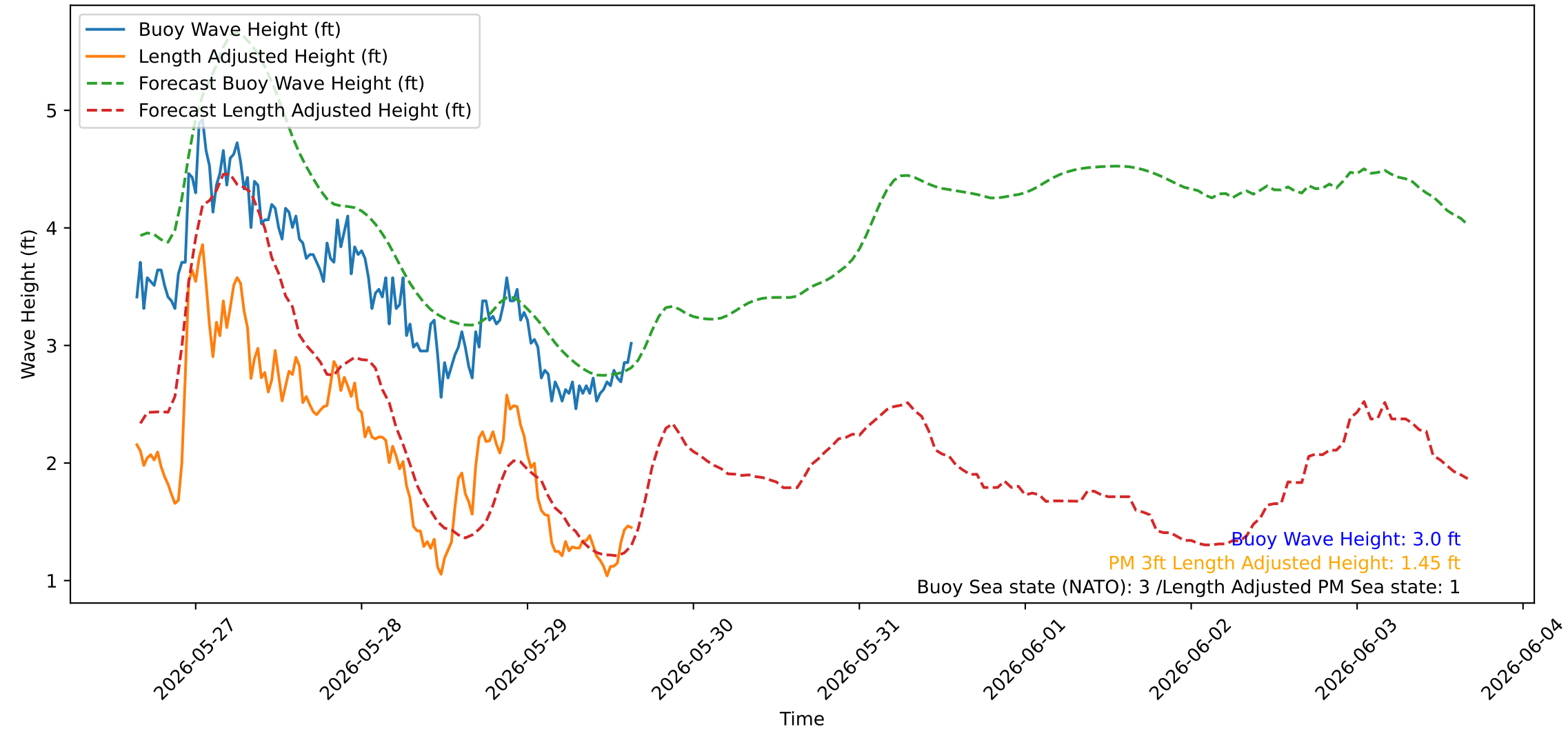
Wave Heights over Time for Green Beach at 2026-05-29 15:41:05
