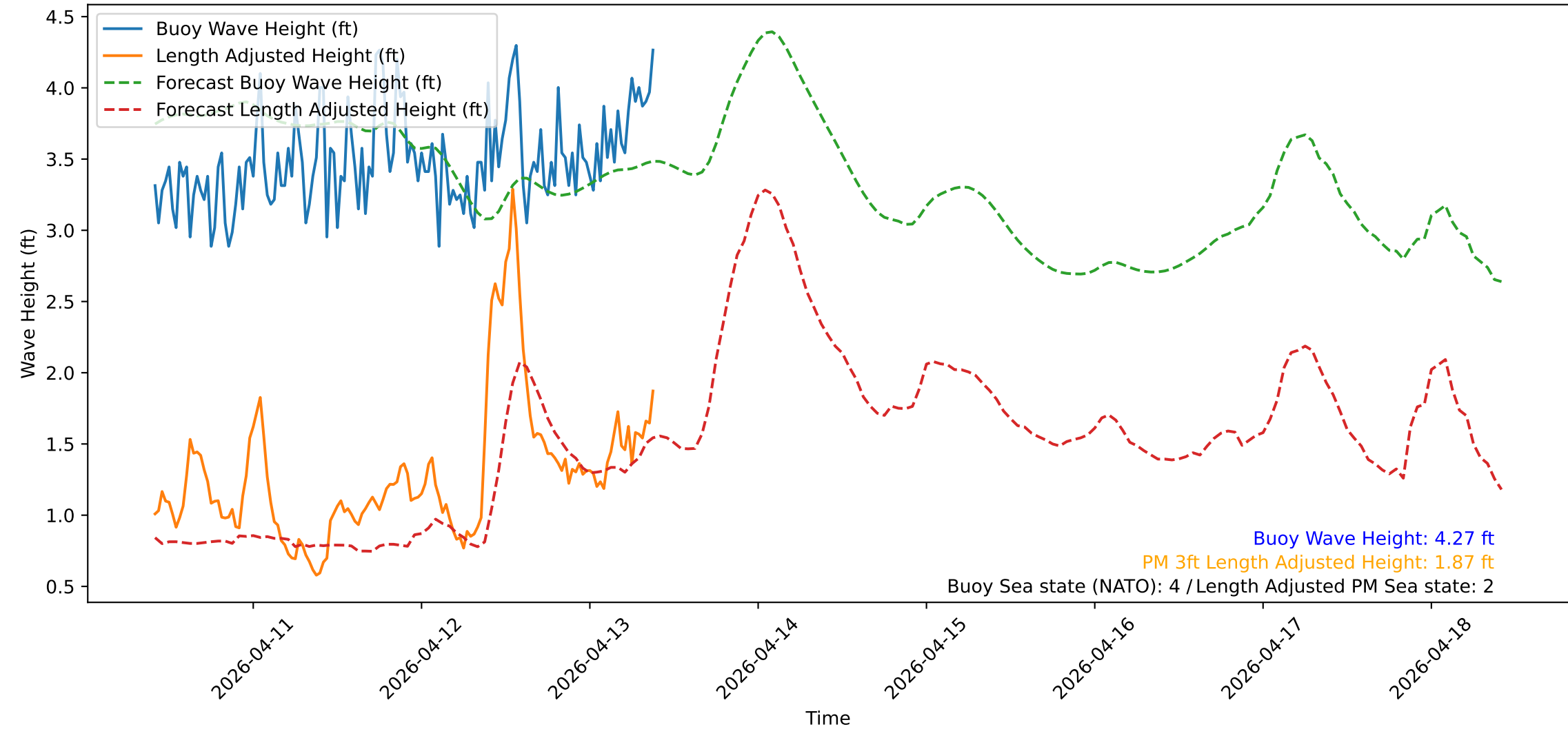
Wave Heights over Time for Red Beach at 2026-04-13 09:50:52
