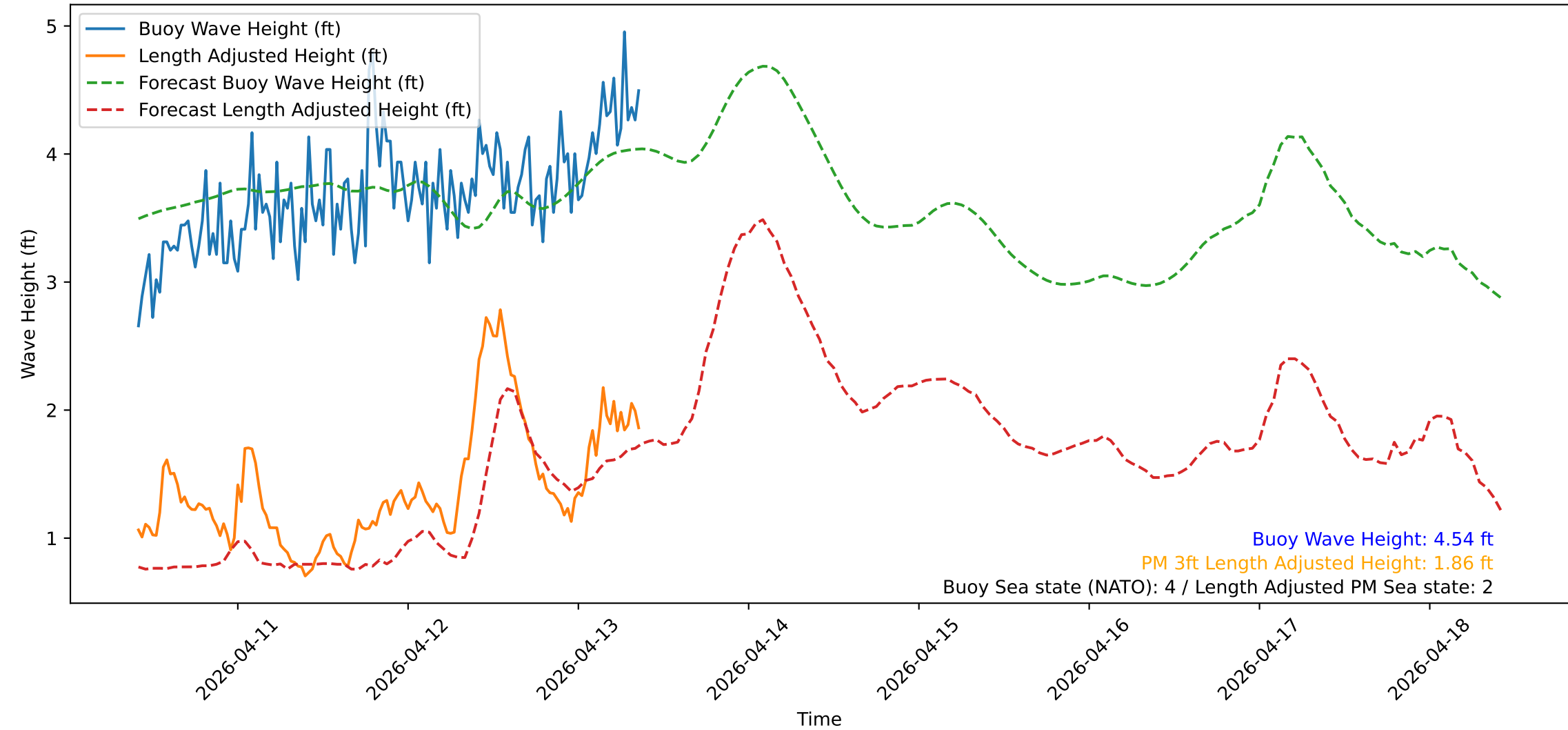
Wave Heights over Time for Oceanside Harbor at 2026-04-13 09:50:31
