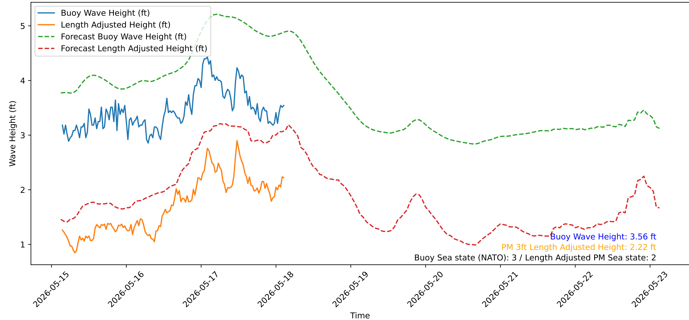
Wave Heights over Time for Green Beach at 2026-05-18 03:21:15
