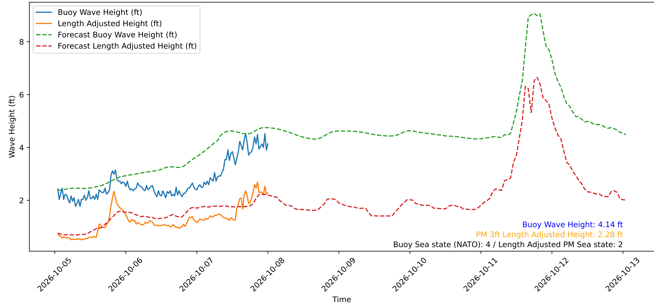
Wave Heights over Time for Green Beach at 2026-10-08 00:41:12
