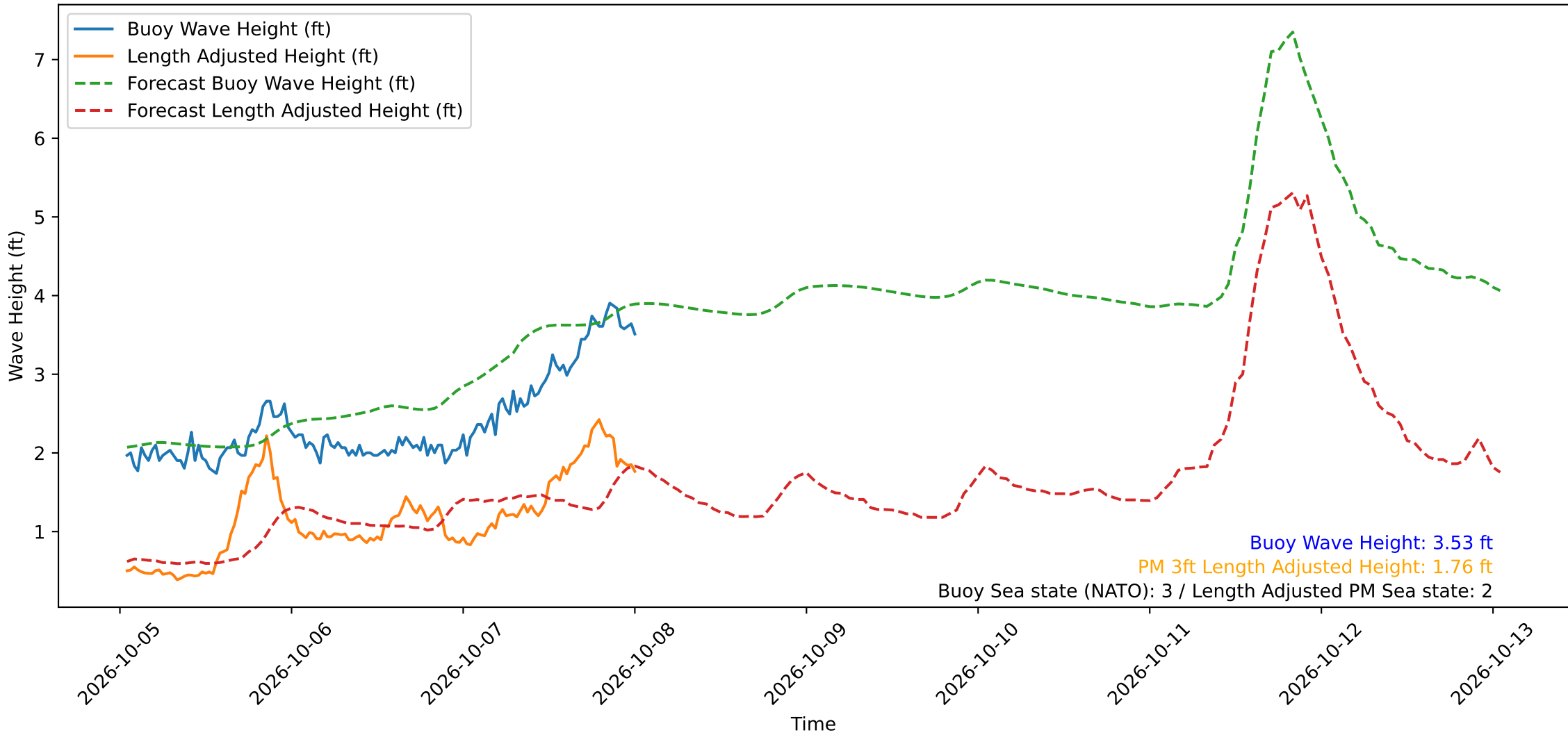
Wave Heights over Time for Red Beach at 2026-10-08 00:40:50
