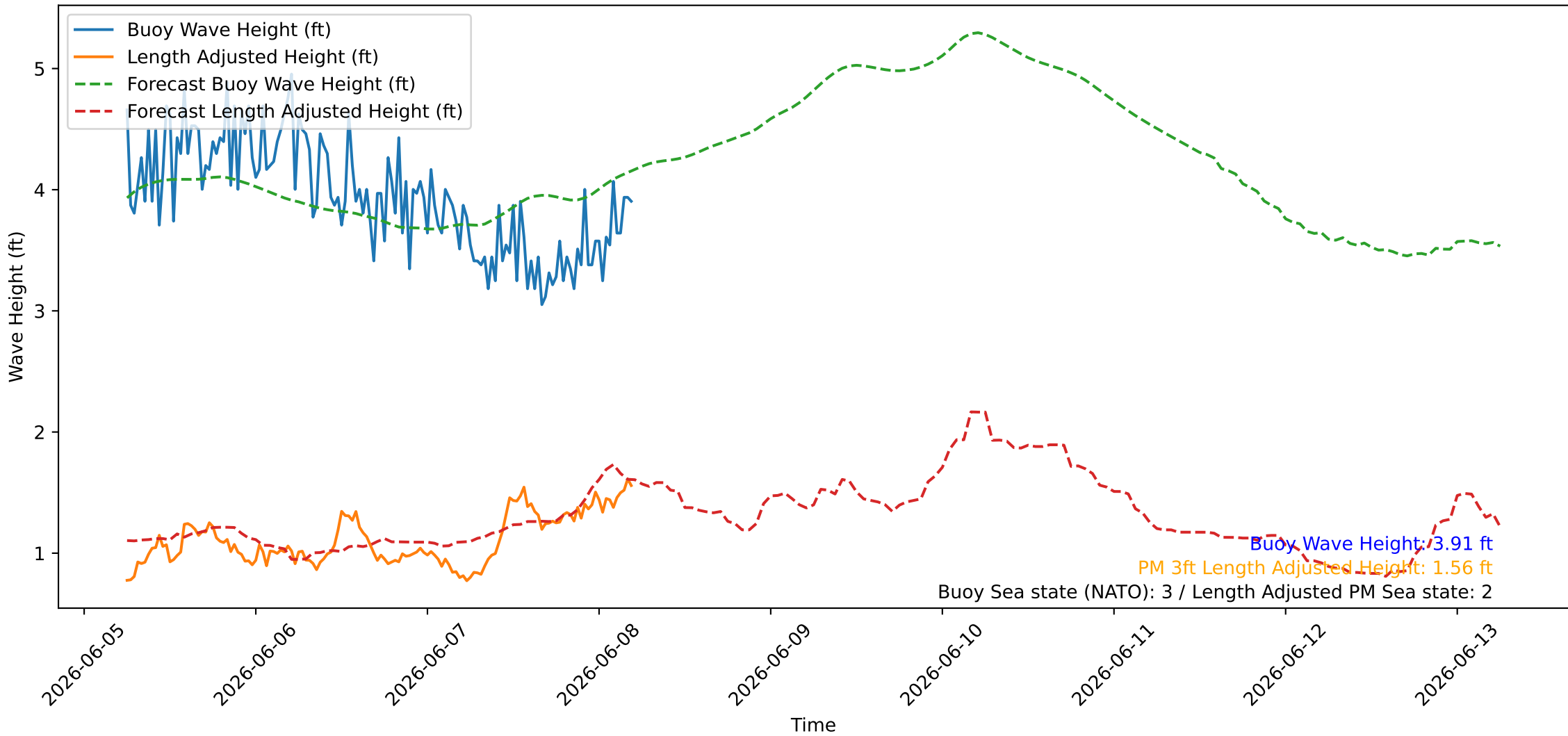
Wave Heights over Time for Red Beach at 2026-06-08 05:30:45
