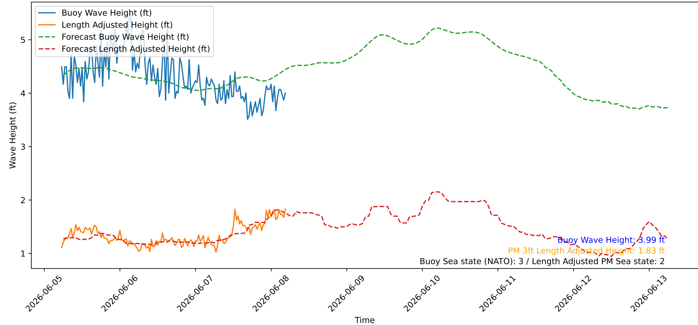
Wave Heights over Time for Oceanside Harbor at 2026-06-08 05:30:26
