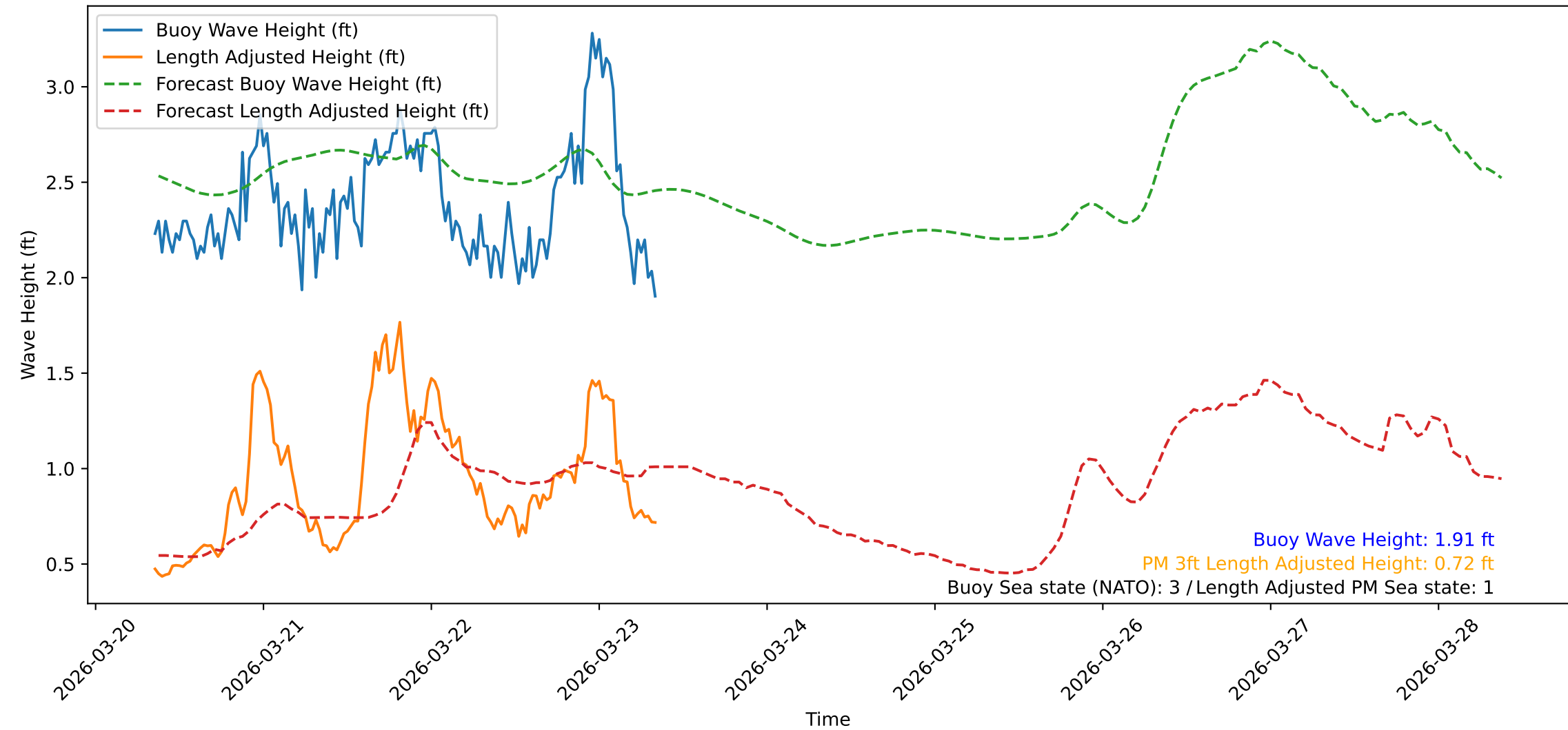
Wave Heights over Time for Green Beach at 2026-03-23 08:41:09
