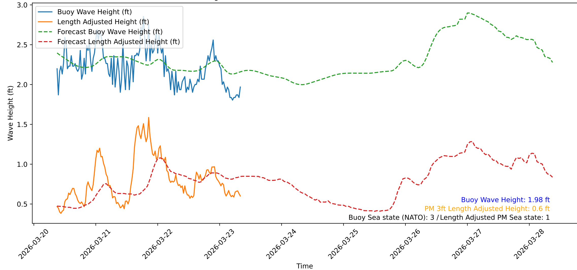
Wave Heights over Time for Red Beach at 2026-03-23 08:40:47
