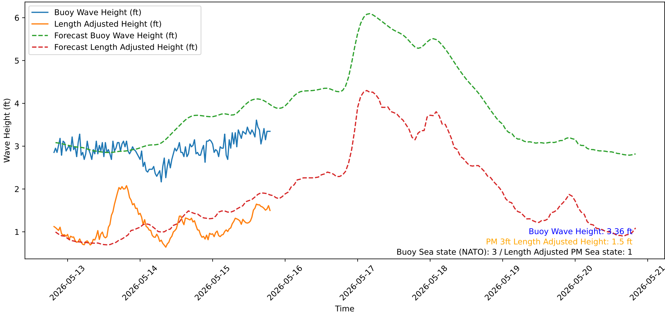
Wave Heights over Time for Oceanside Harbor at 2026-05-15 19:30:32
