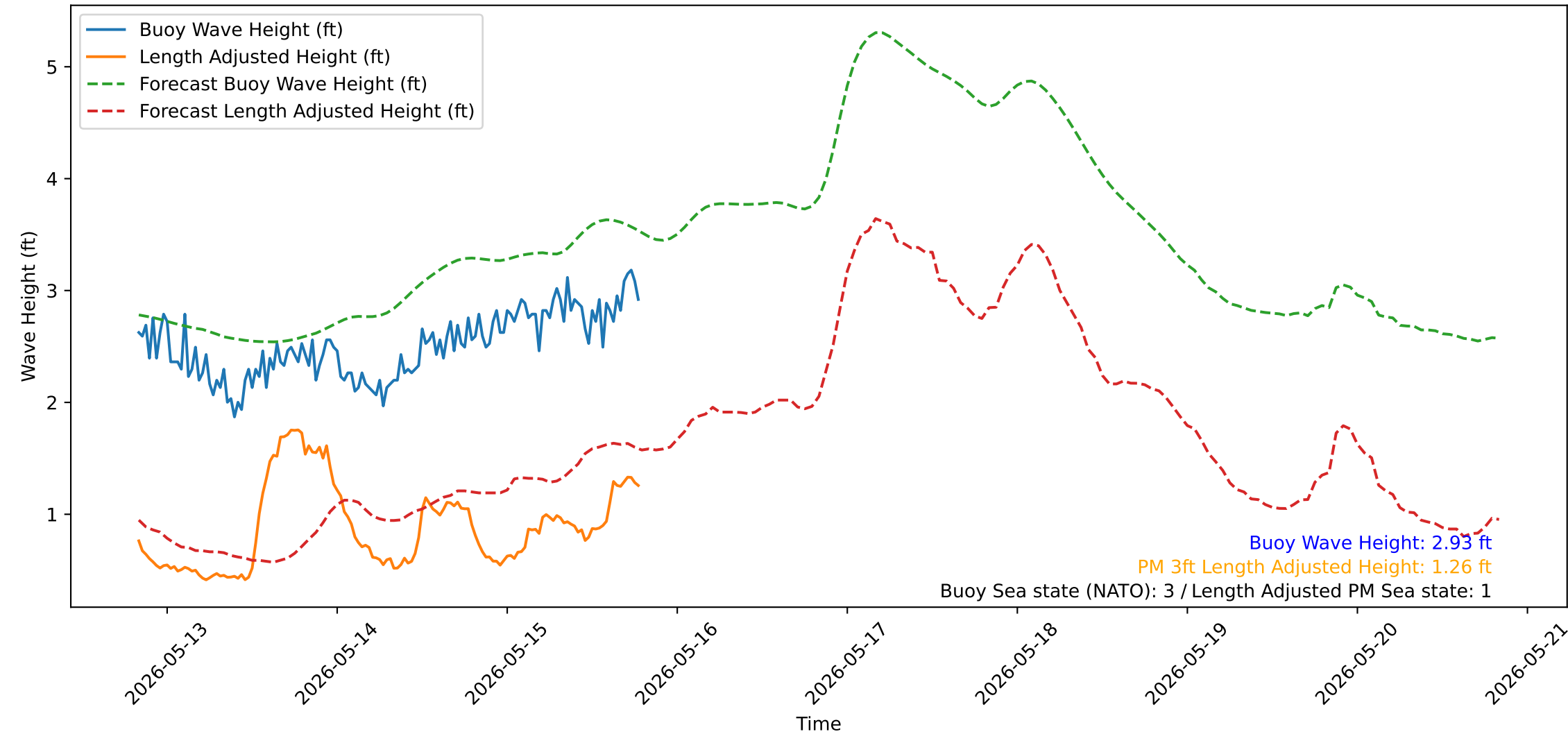
Wave Heights over Time for Red Beach at 2026-05-15 19:30:51
