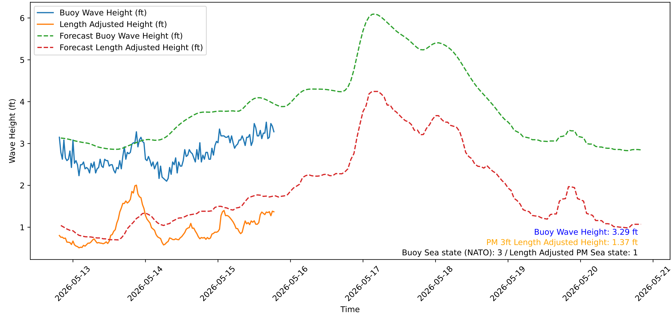
Wave Heights over Time for Green Beach at 2026-05-15 19:31:16
