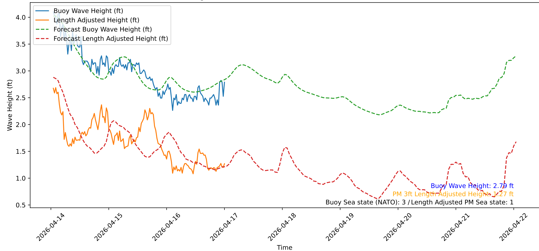
Wave Heights over Time for Red Beach at 2026-04-17 00:50:52
