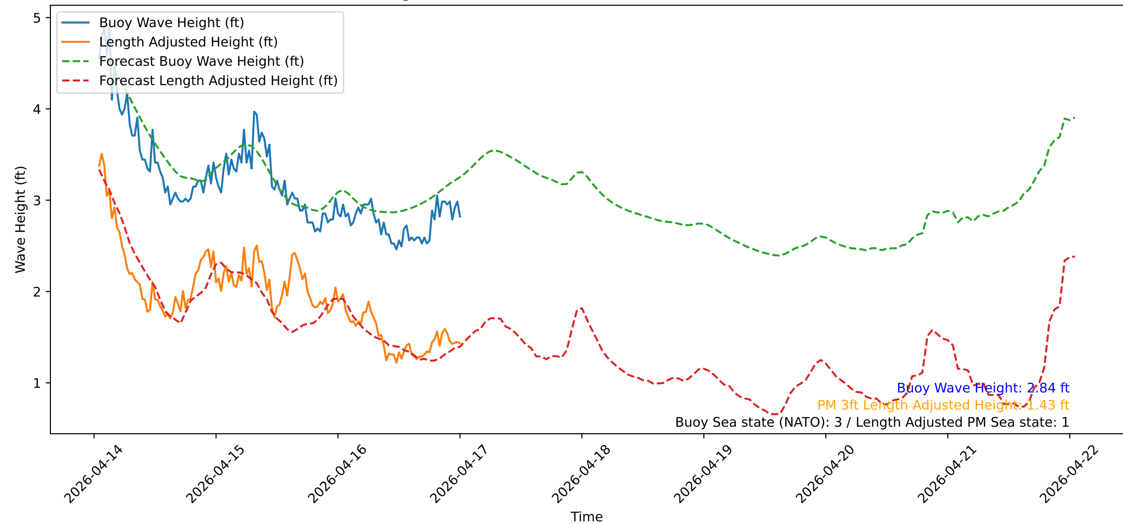
Wave Heights over Time for Green Beach at 2026-04-17 00:51:15
