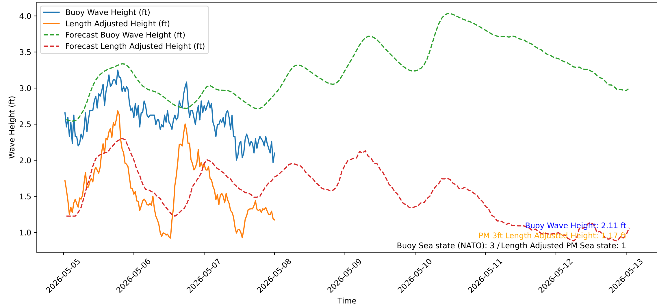
Wave Heights over Time for Oceanside Harbor at 2026-05-08 00:30:31
