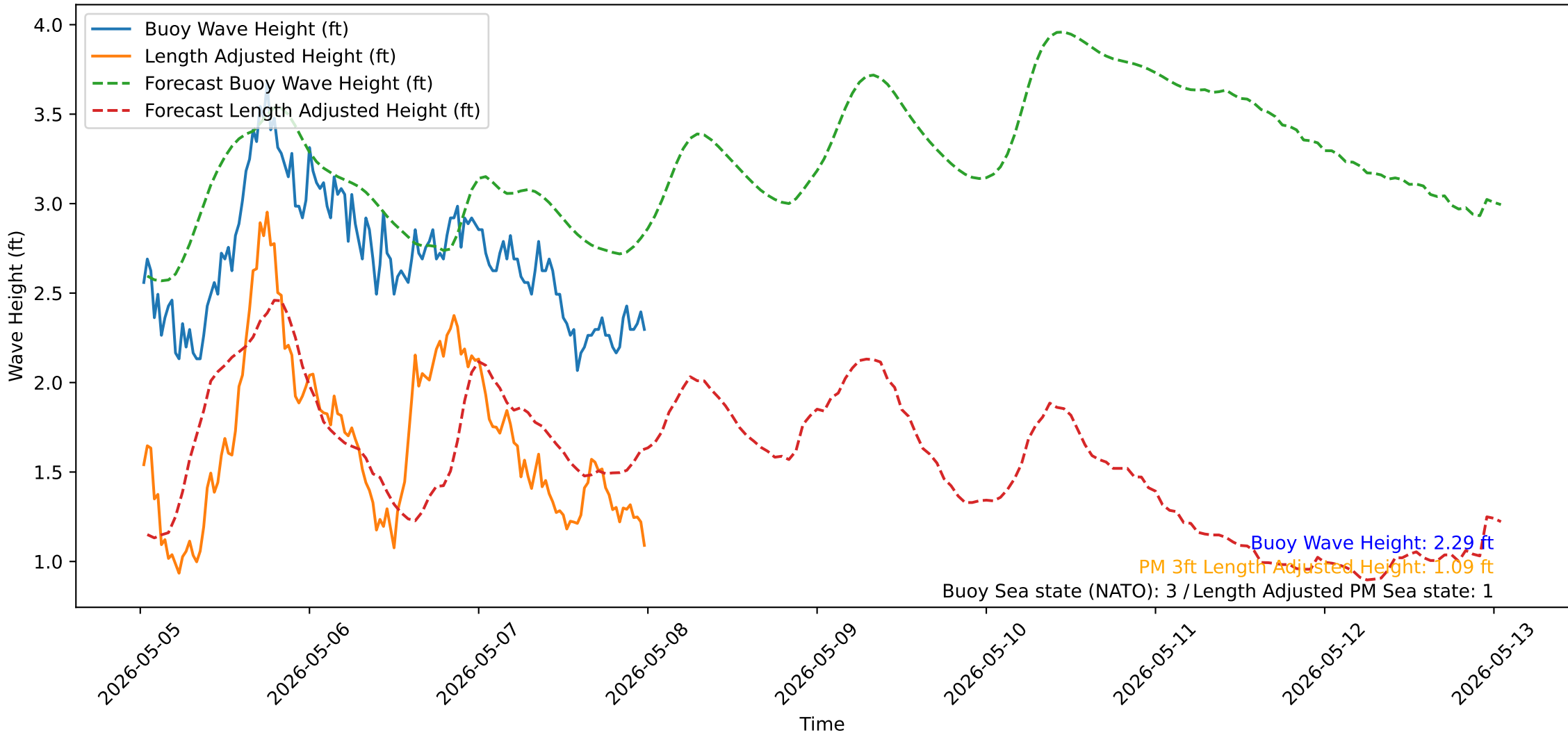
Wave Heights over Time for Green Beach at 2026-05-08 00:31:12
