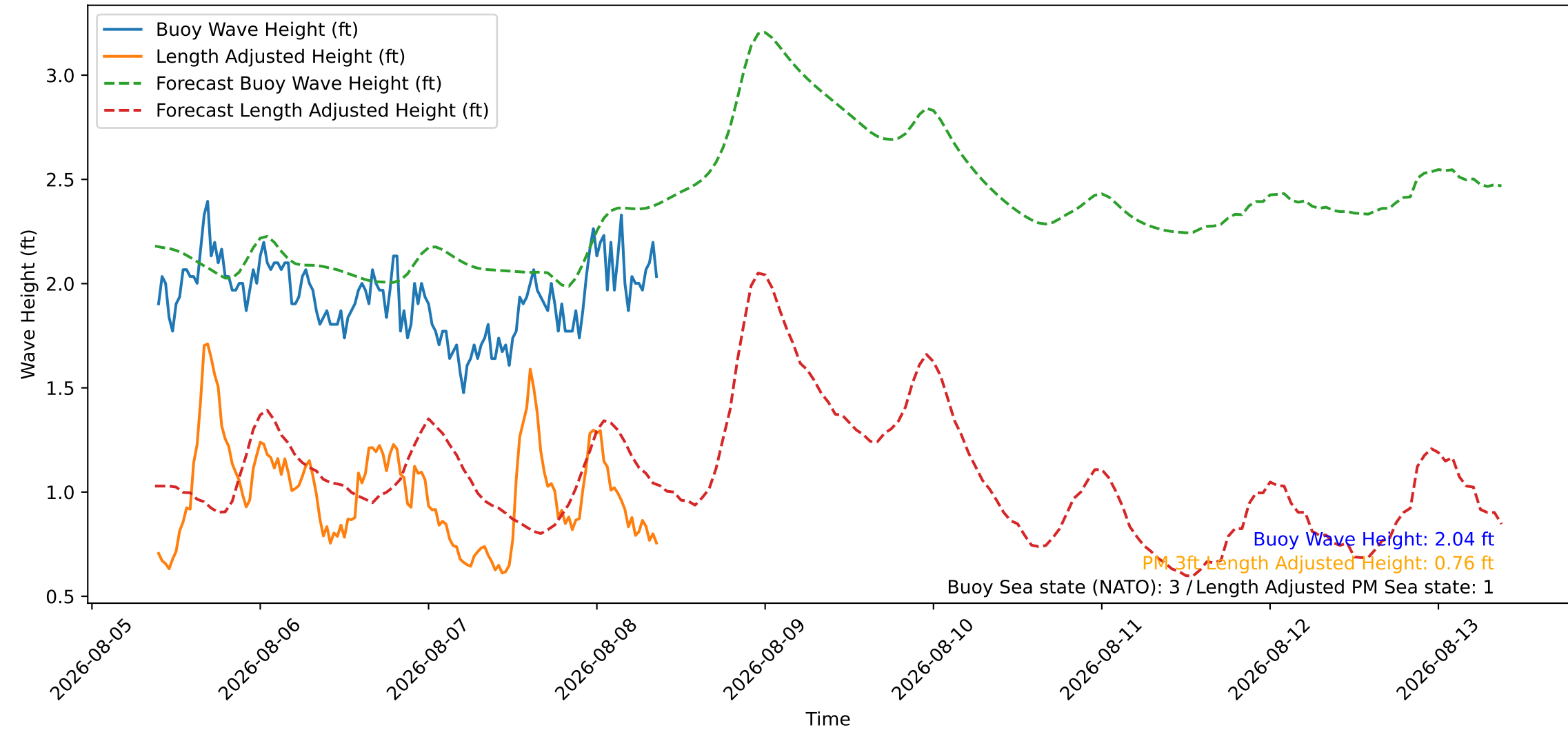
Wave Heights over Time for Red Beach at 2026-08-08 09:10:46
