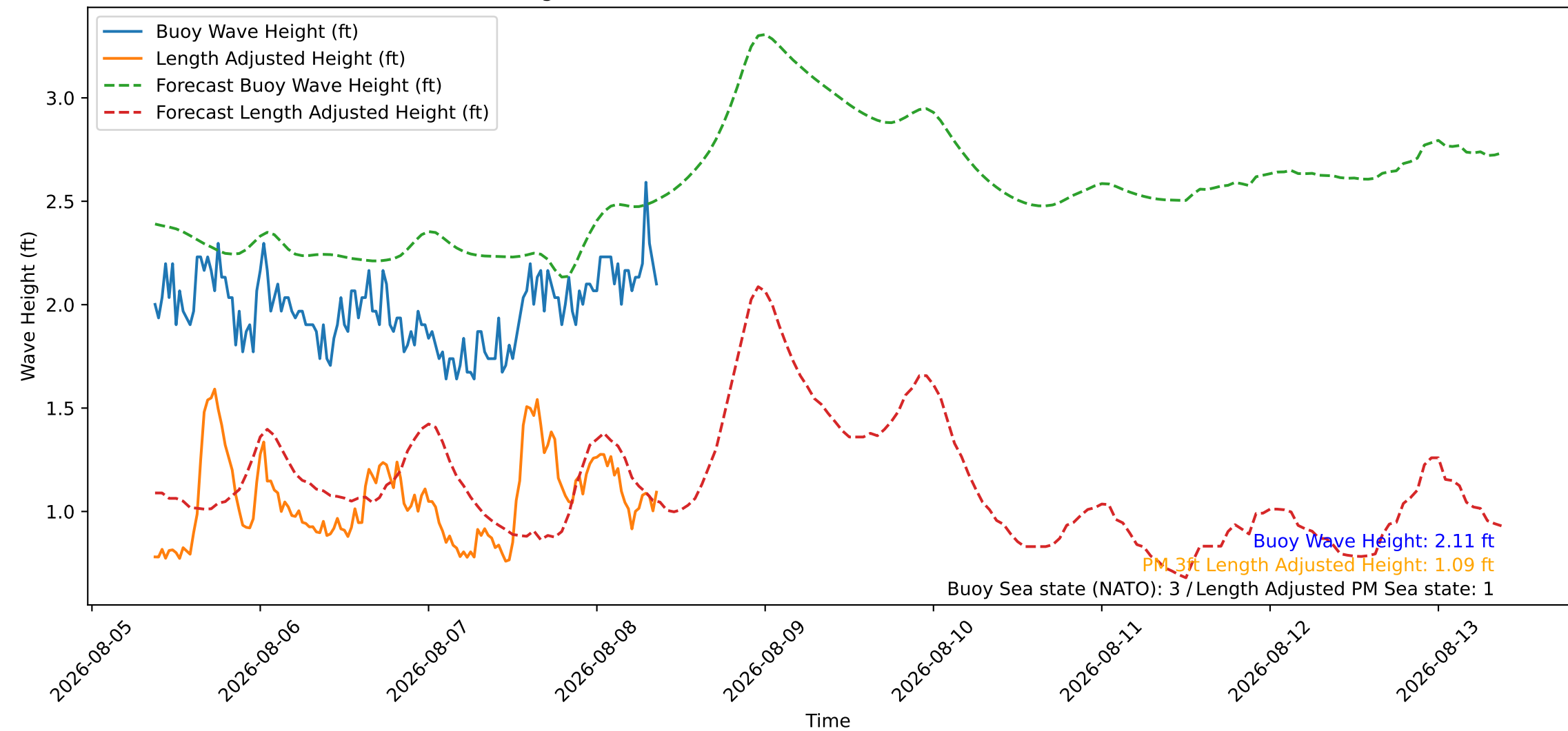
Wave Heights over Time for Oceanside Harbor at 2026-08-08 09:10:26
