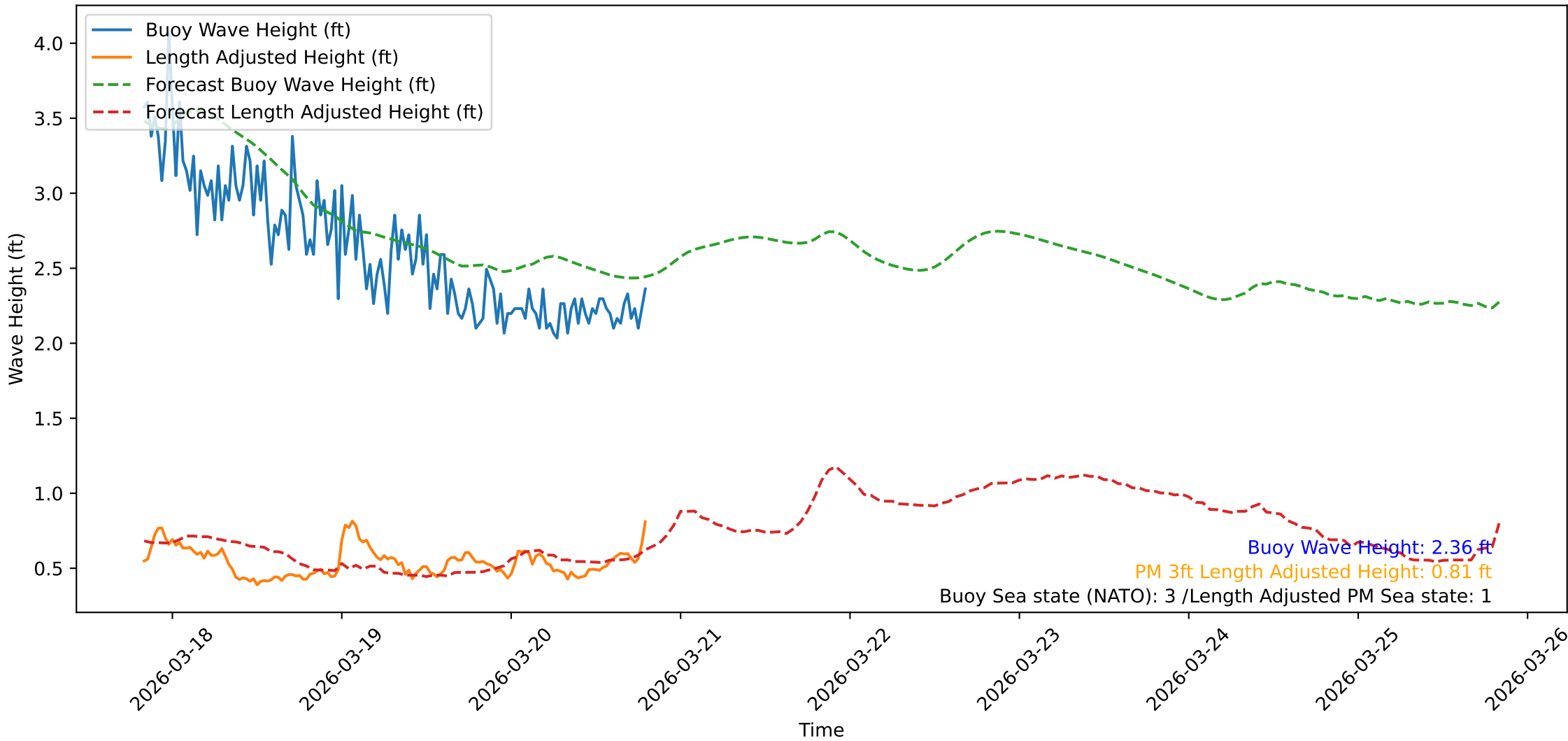
Wave Heights over Time for Green Beach at 2026-03-20 19:51:09
