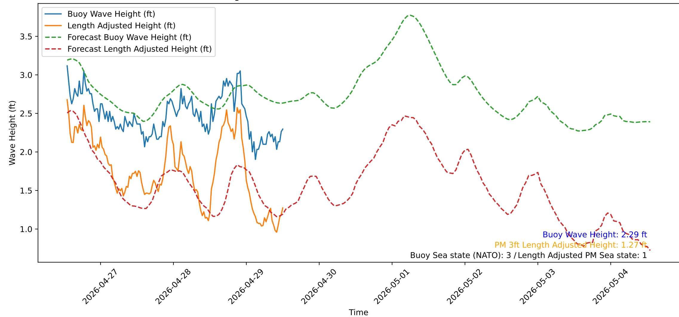
Wave Heights over Time for Oceanside Harbor at 2026-04-29 12:50:31
