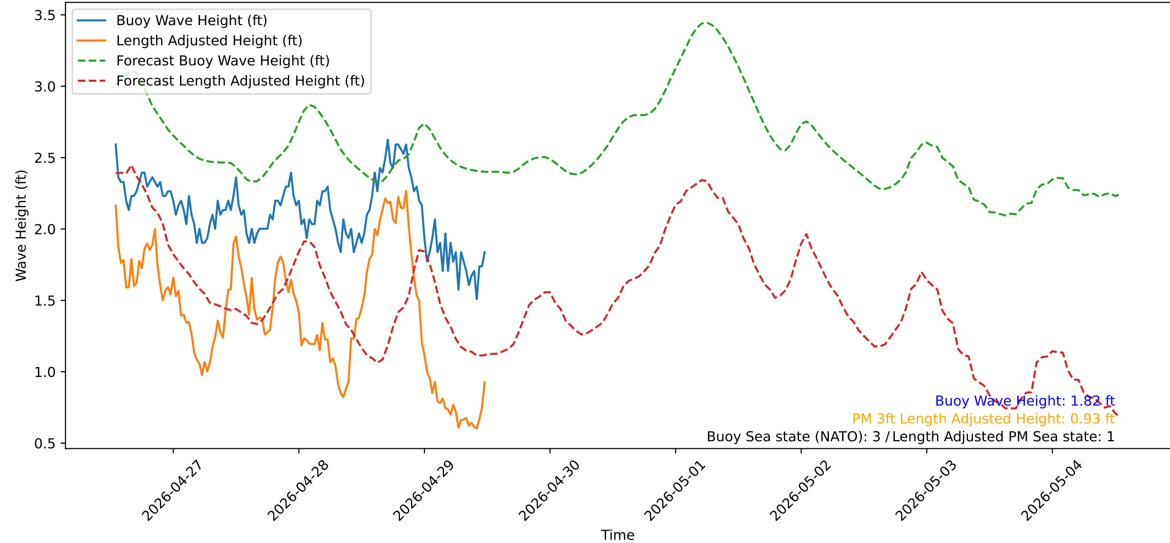
Wave Heights over Time for Red Beach at 2026-04-29 12:50:52
