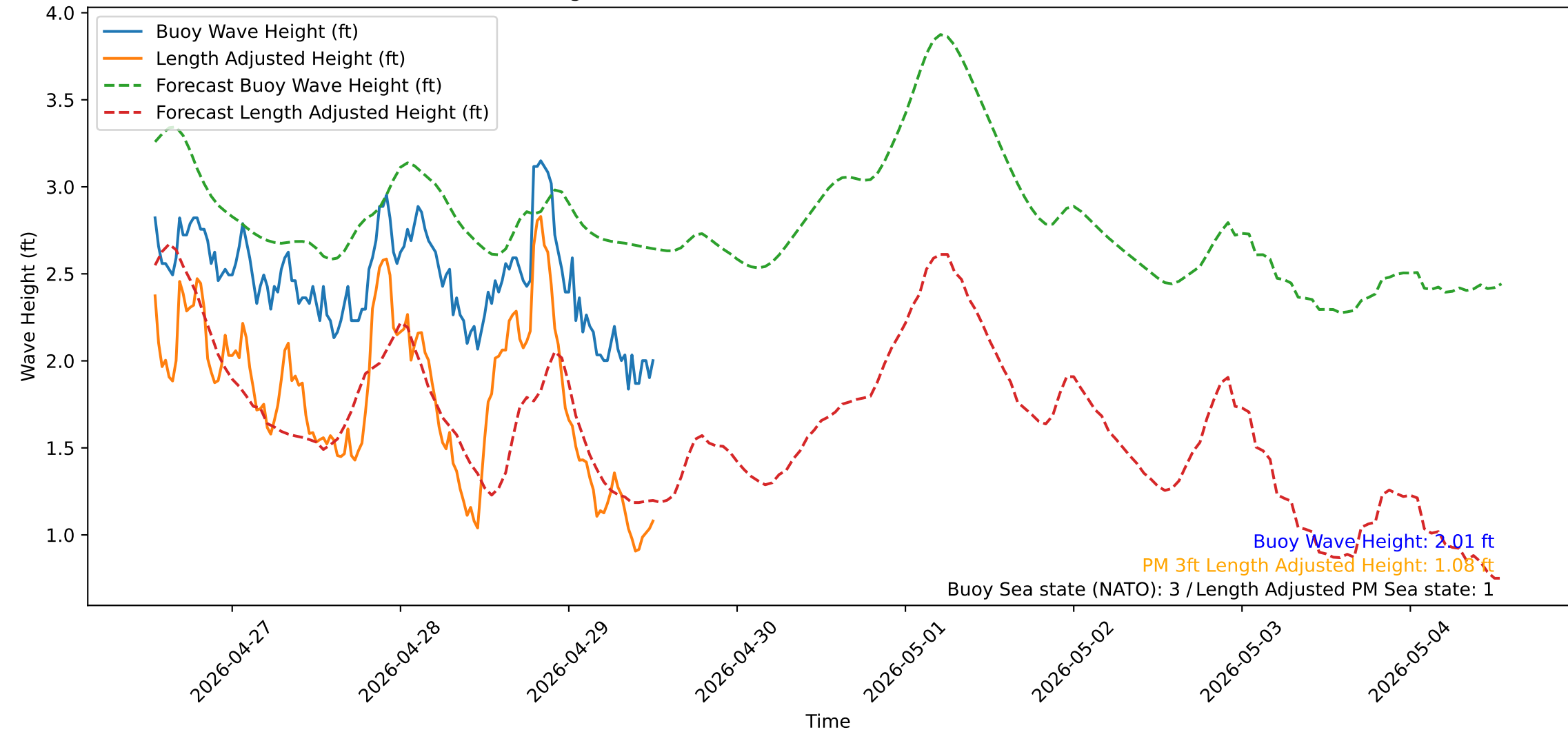
Wave Heights over Time for Green Beach at 2026-04-29 12:51:15
