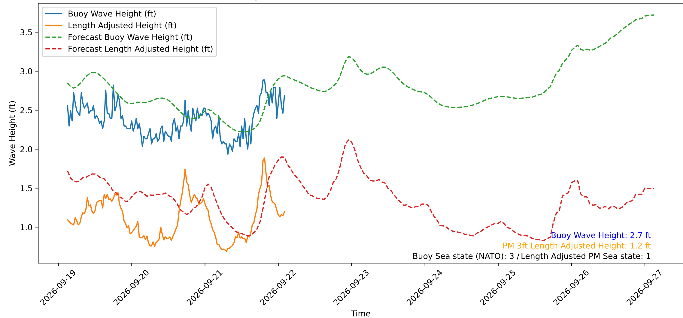
Wave Heights over Time for Red Beach at 2026-09-22 02:50:50
