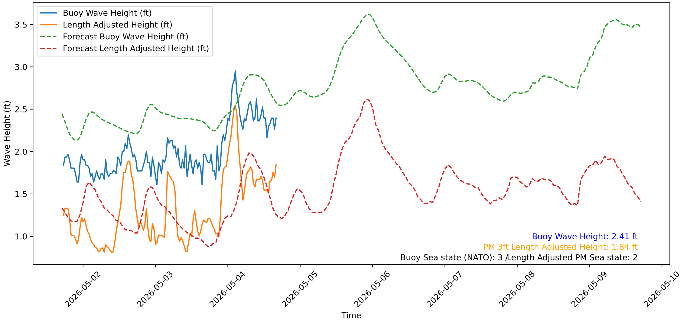
Wave Heights over Time for Red Beach at 2026-05-04 17:00:50
