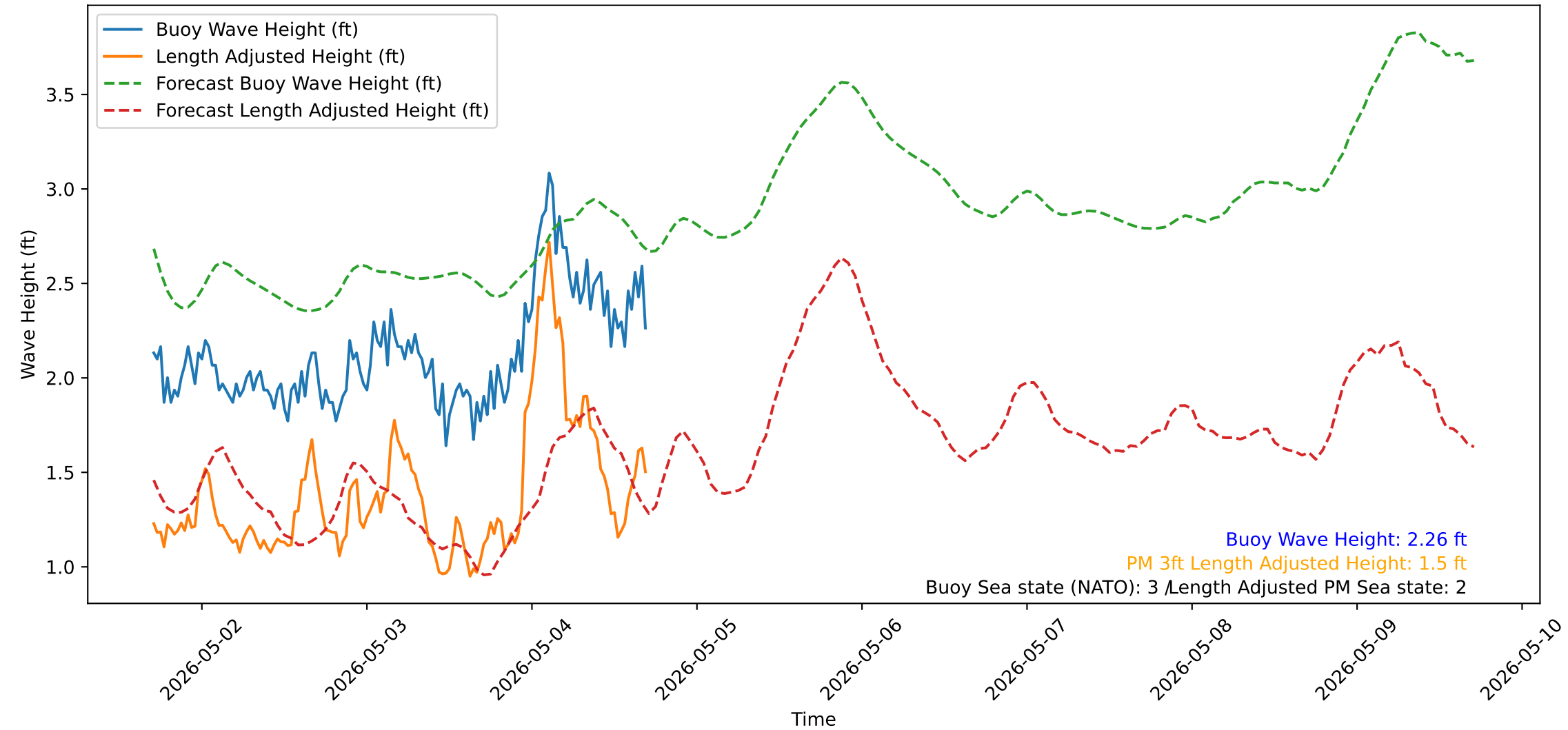
Wave Heights over Time for Oceanside Harbor at 2026-05-04 17:00:31
