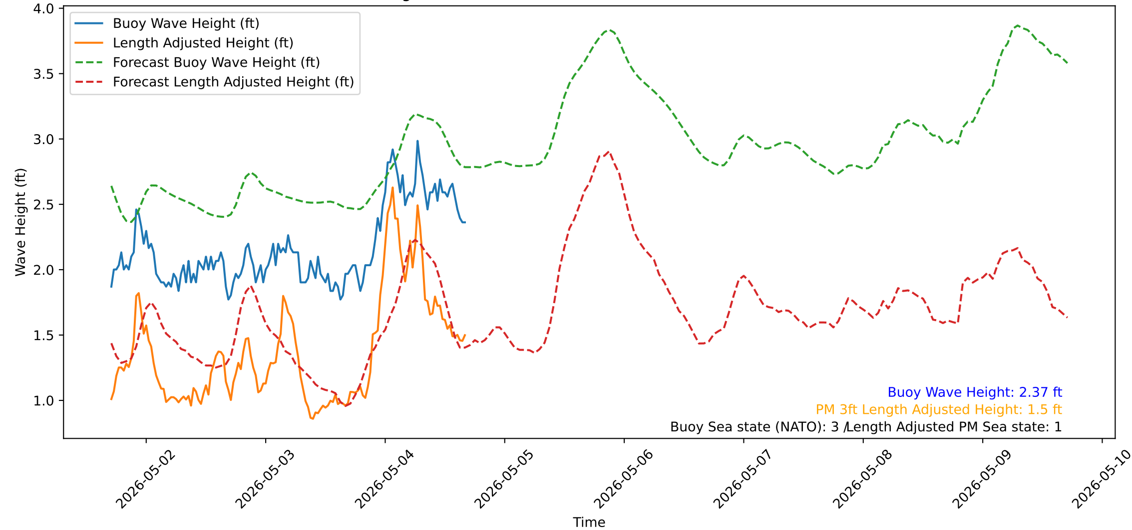
Wave Heights over Time for Green Beach at 2026-05-04 17:01:12
