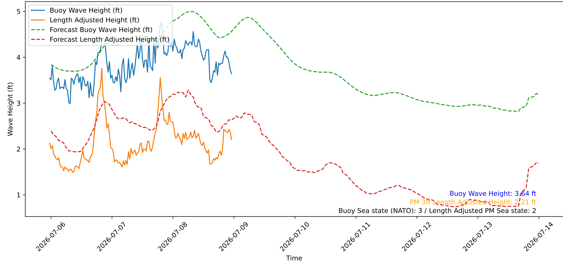
Wave Heights over Time for Green Beach at 2026-07-08 23:41:08
