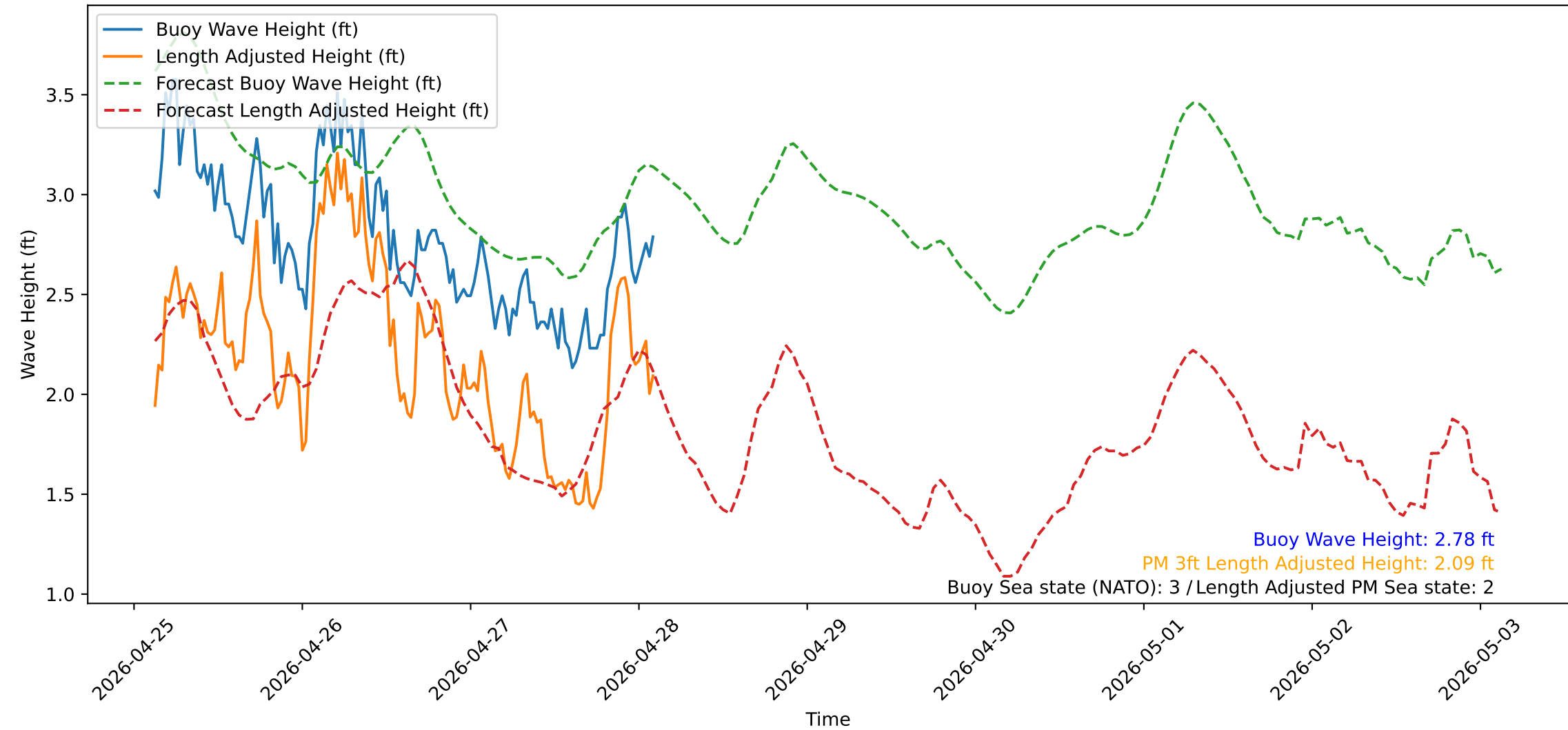
Wave Heights over Time for Green Beach at 2026-04-28 02:51:14
