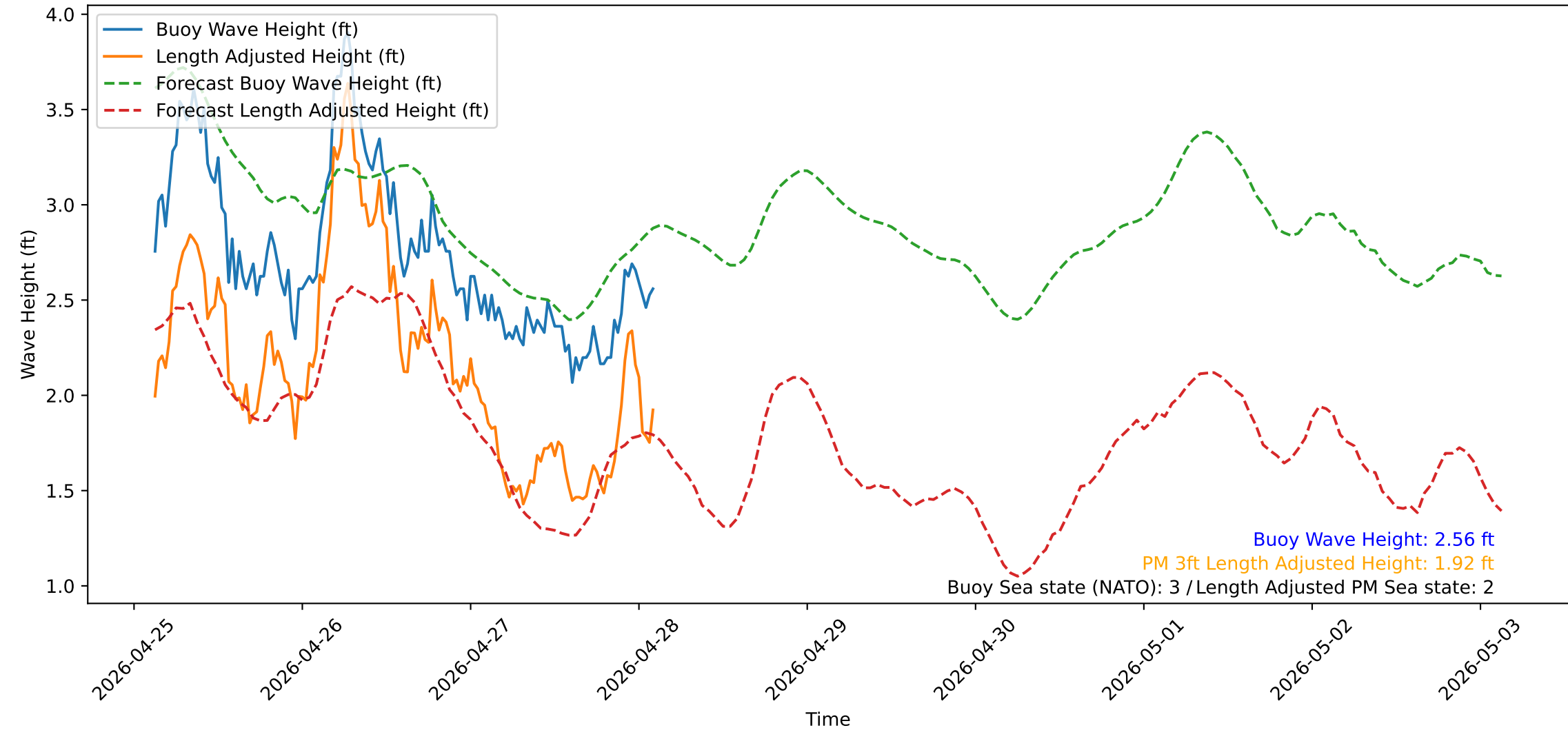
Wave Heights over Time for Oceanside Harbor at 2026-04-28 02:50:31
